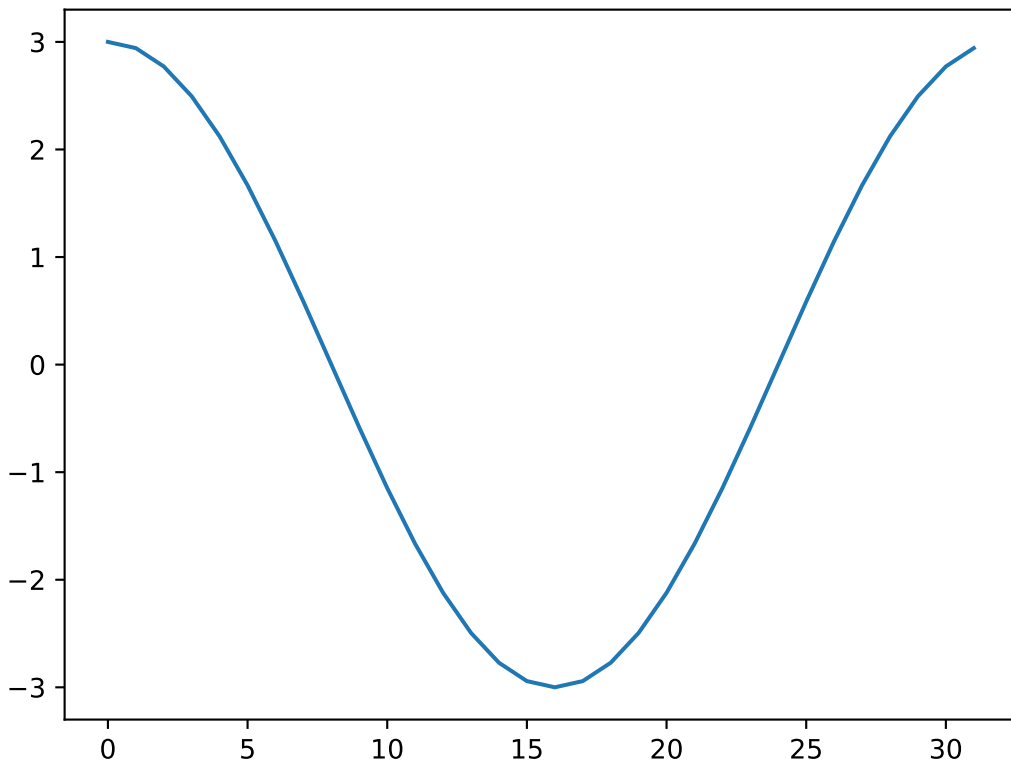
Reconstructed unshifted cosine
