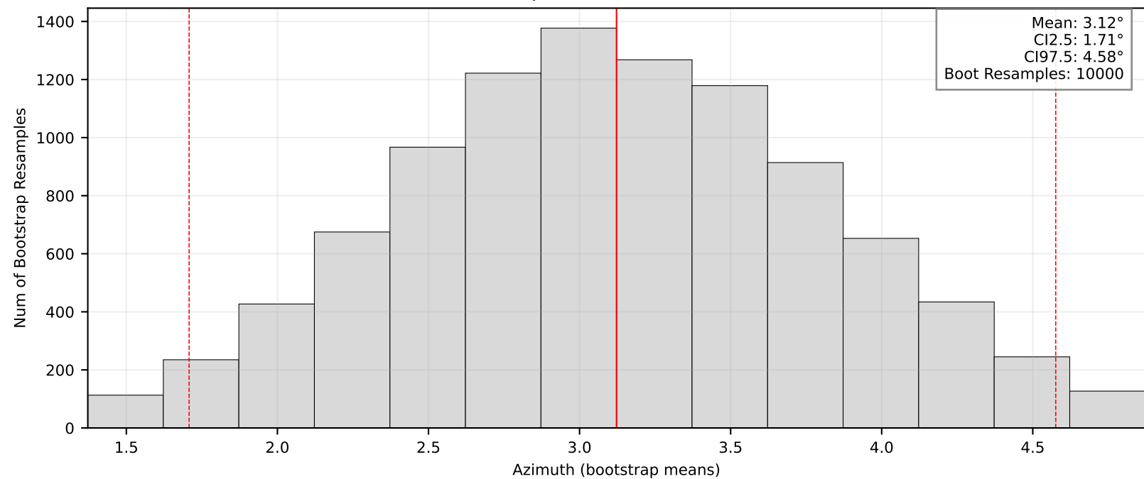
Bootstrap Means/95% CI: BK.MERC
