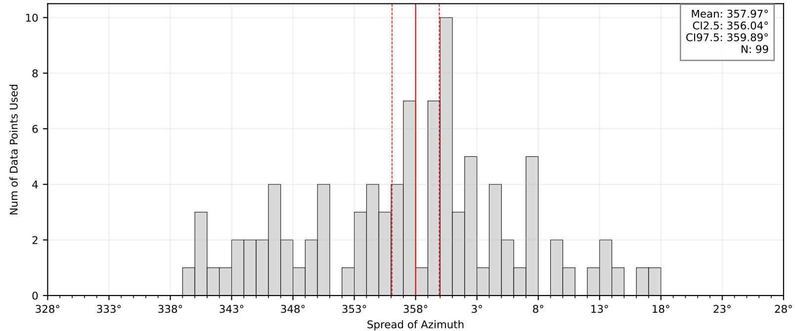
Bootstrap Mean and Confidence Intervals: BK.GCKB
