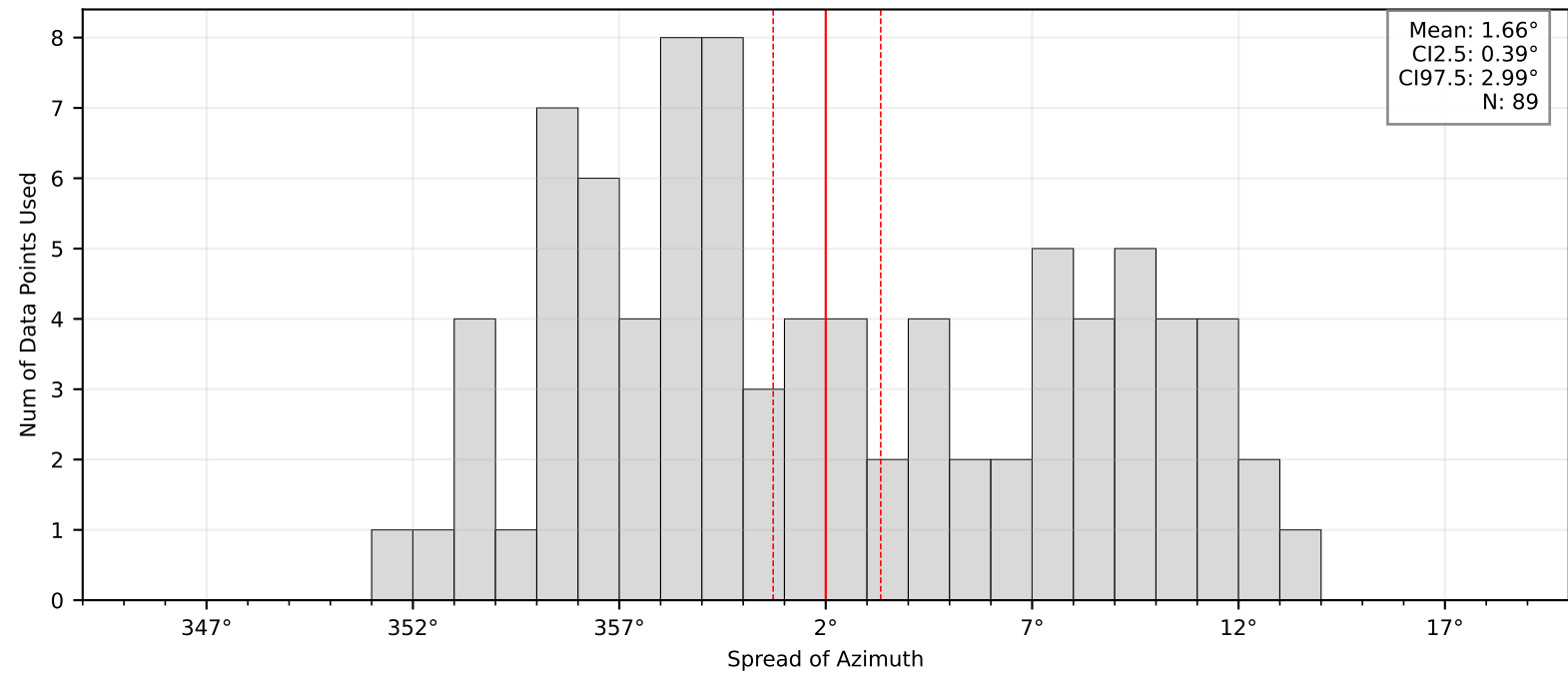
Bootstrap Mean and Confidence Intervals: BK.LAND
