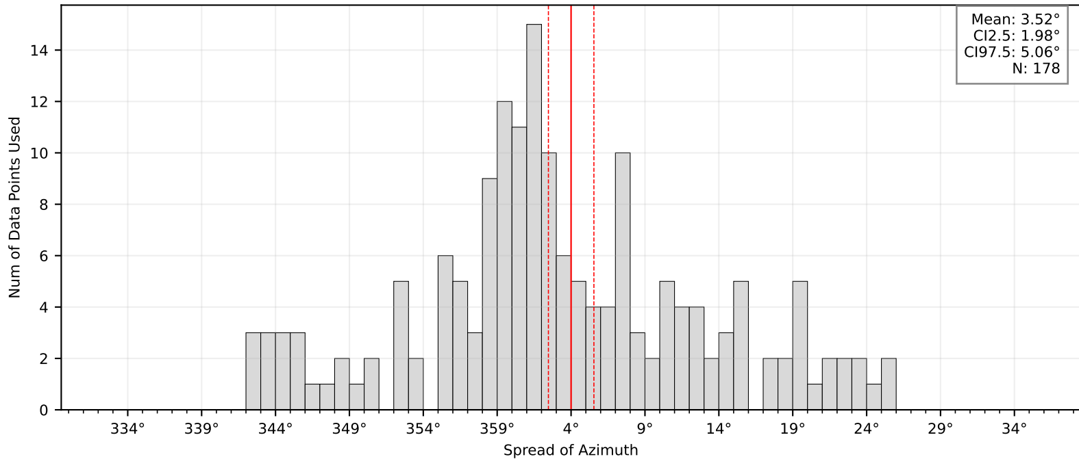
Bootstrap Mean and Confidence Intervals: BK.DRDG
