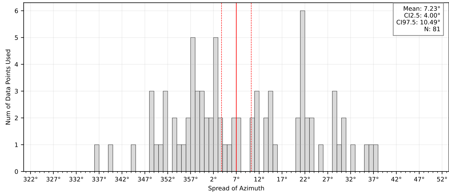
Bootstrap Mean and Confidence Intervals: BK.TOLH
