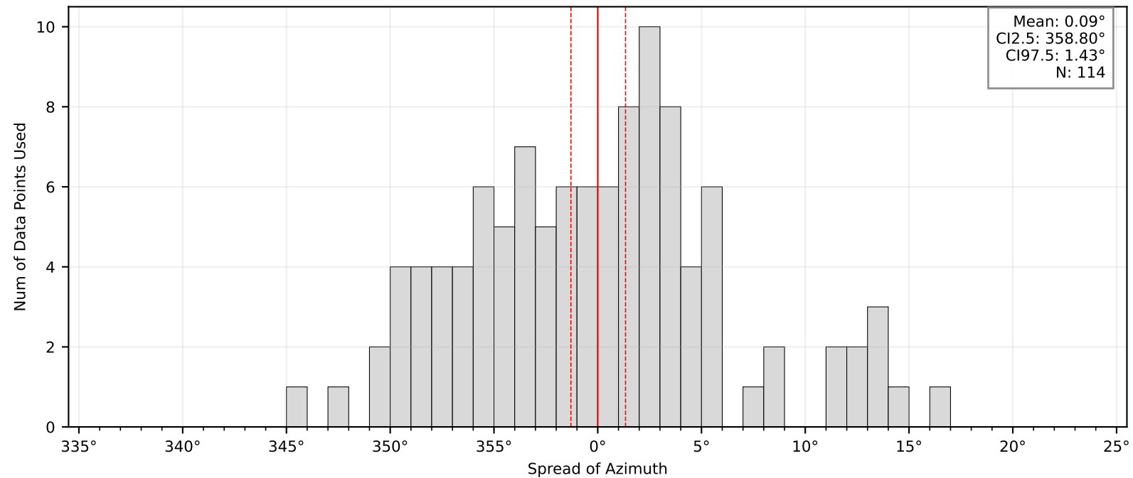
Bootstrap Mean and Confidence Intervals: BK.SHEP
