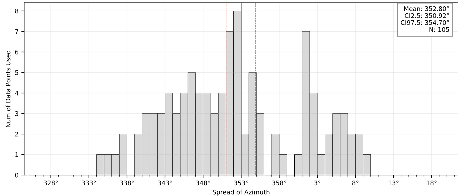
Bootstrap Mean and Confidence Intervals: BK.ETSL
