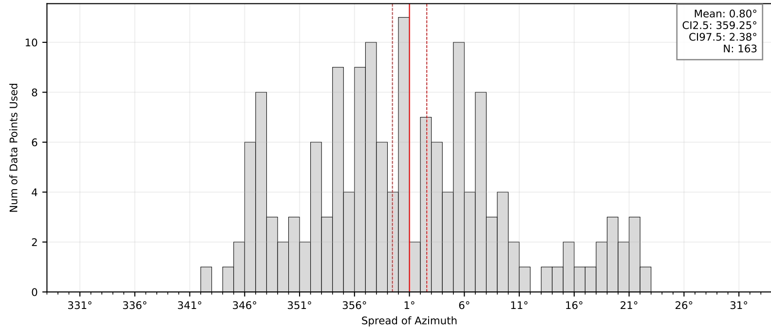
Bootstrap Mean and Confidence Intervals: BK.BKS
