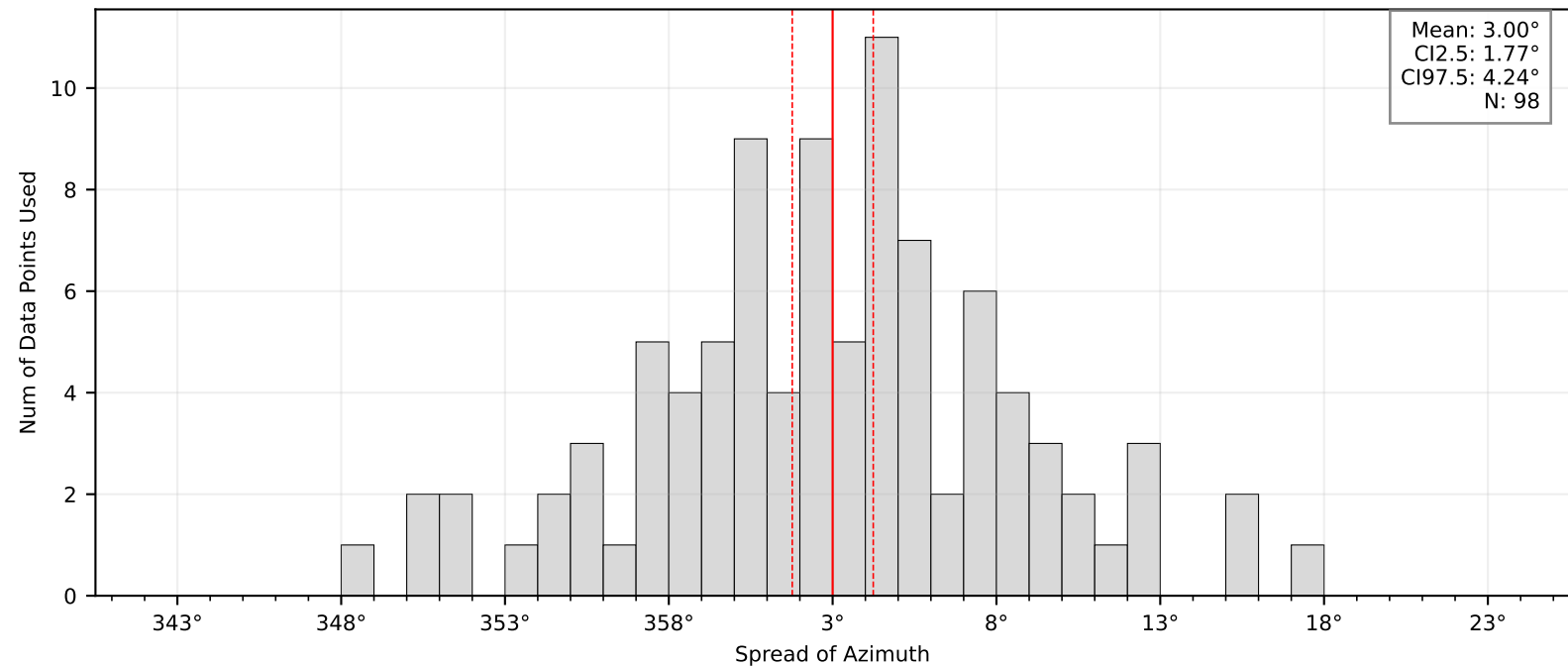
Bootstrap Mean and Confidence Intervals: BK.USAL
