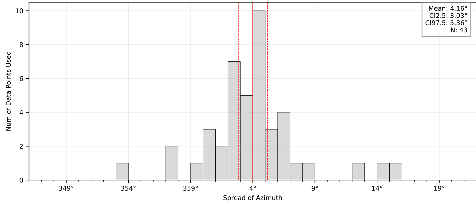
Bootstrap Mean and Confidence Intervals: BK.JRSC
