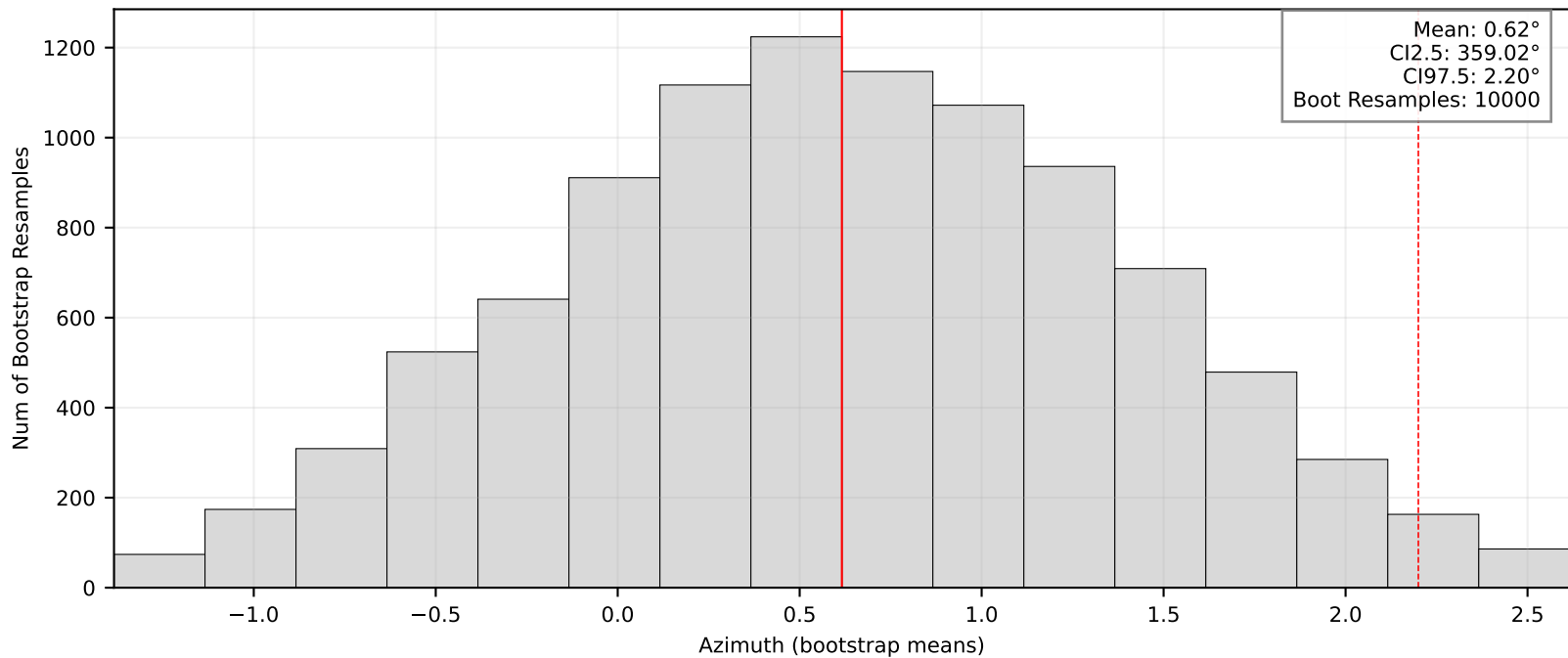
Bootstrap Means/95% CI: BK.TSCN
