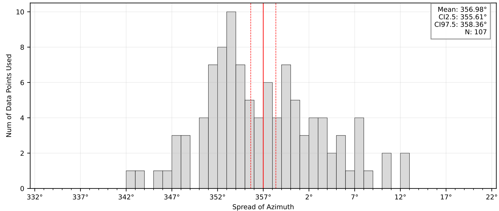
Bootstrap Mean and Confidence Intervals: BK.PESC
