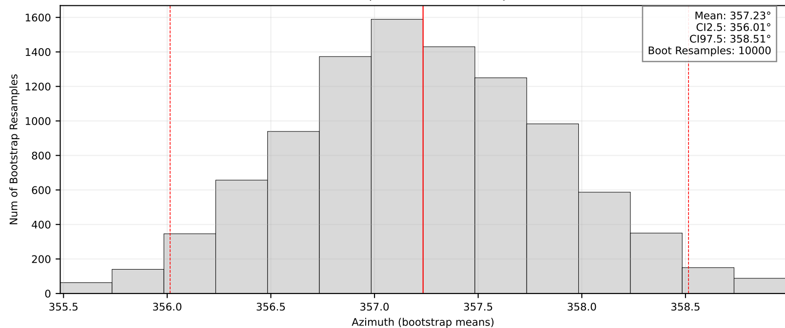
Bootstrap Means/95% CI: BK.JASP
