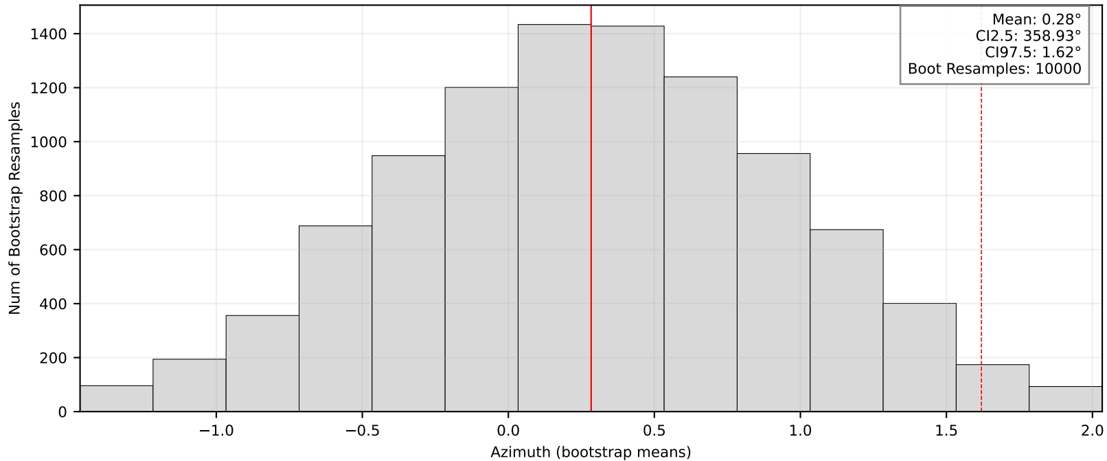
Bootstrap Means/95% CI: BK.HAPY
