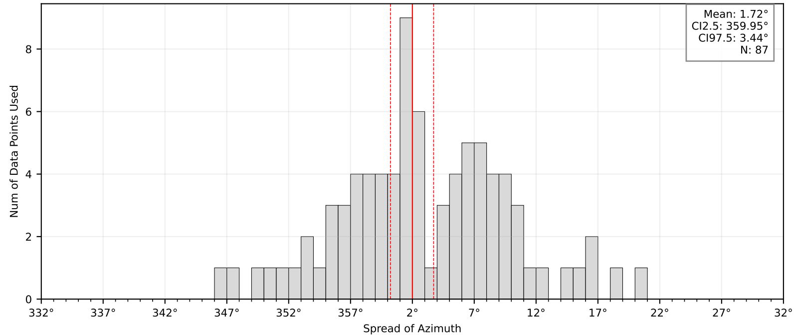
Bootstrap Mean and Confidence Intervals: BK.HALS
