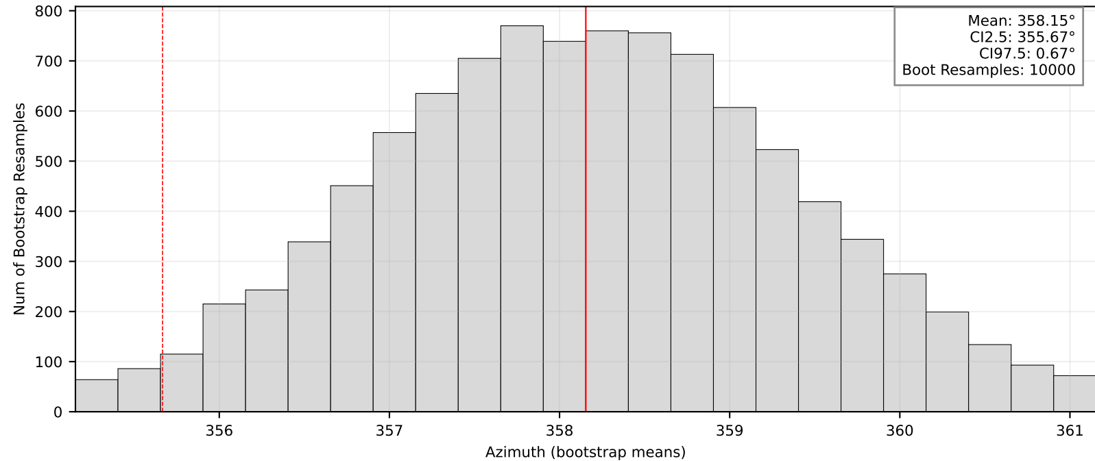
Bootstrap Means/95% CI: BK.GCKB
