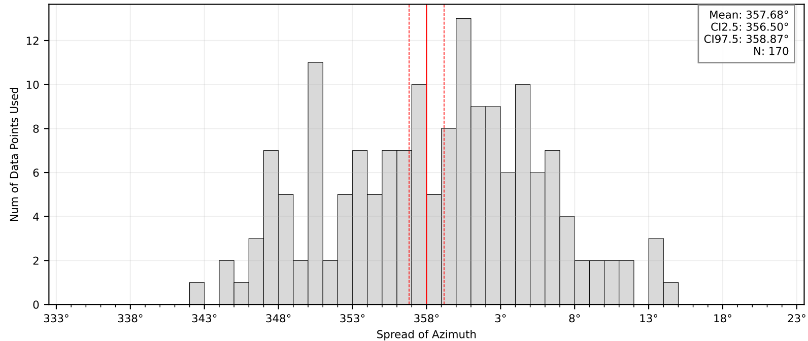
Bootstrap Mean and Confidence Intervals: BK.SPAN
