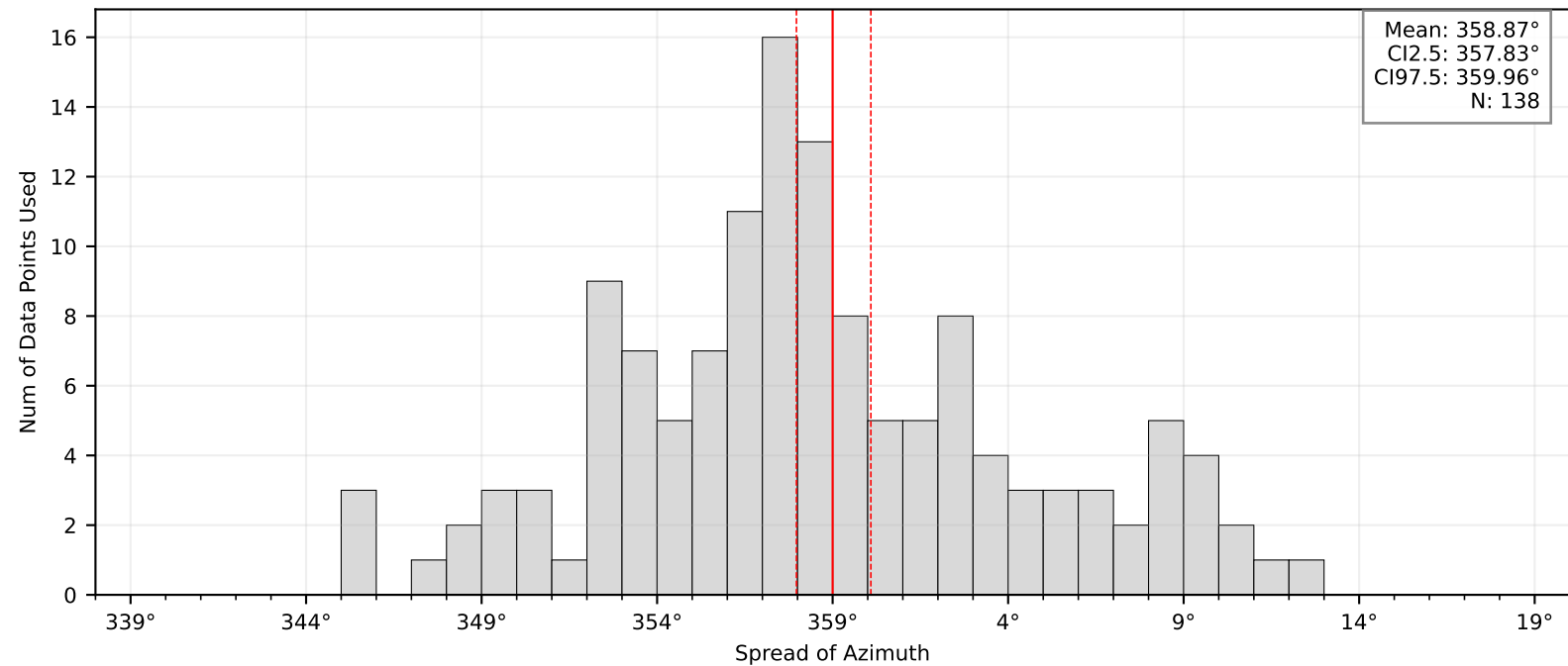
Bootstrap Mean and Confidence Intervals: BK.CLRV
