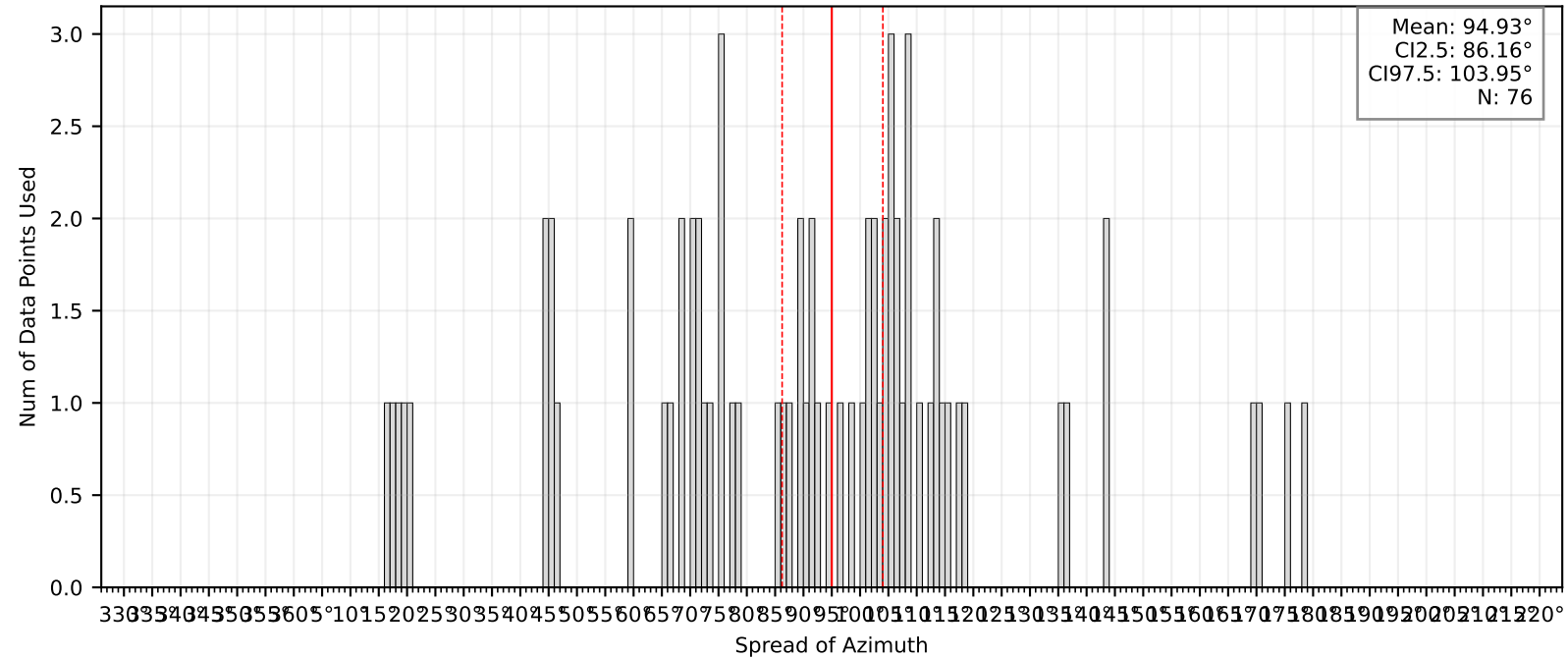
Bootstrap Mean and Confidence Intervals: BK.KCC
