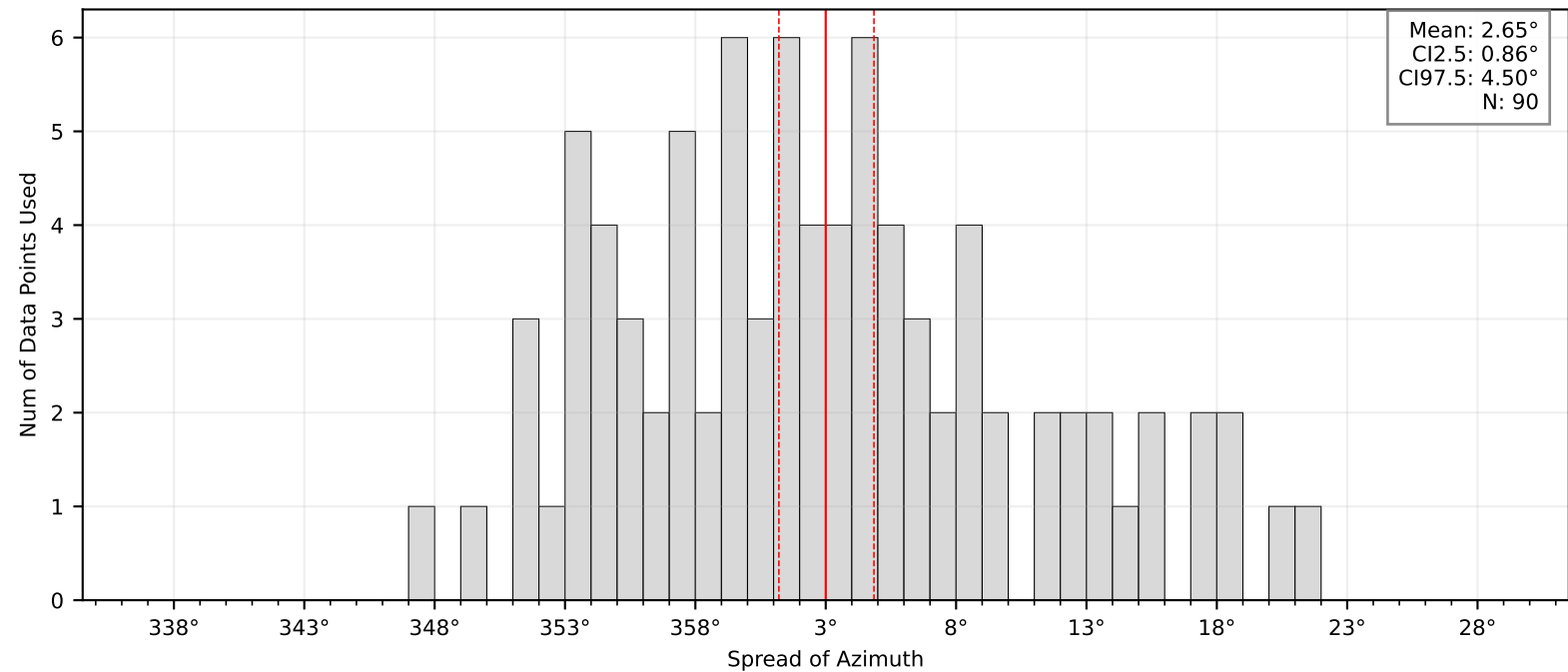
Bootstrap Mean and Confidence Intervals: BK.WHCL
