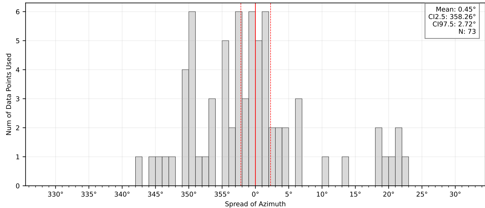
Bootstrap Mean and Confidence Intervals: BK.LAKN
