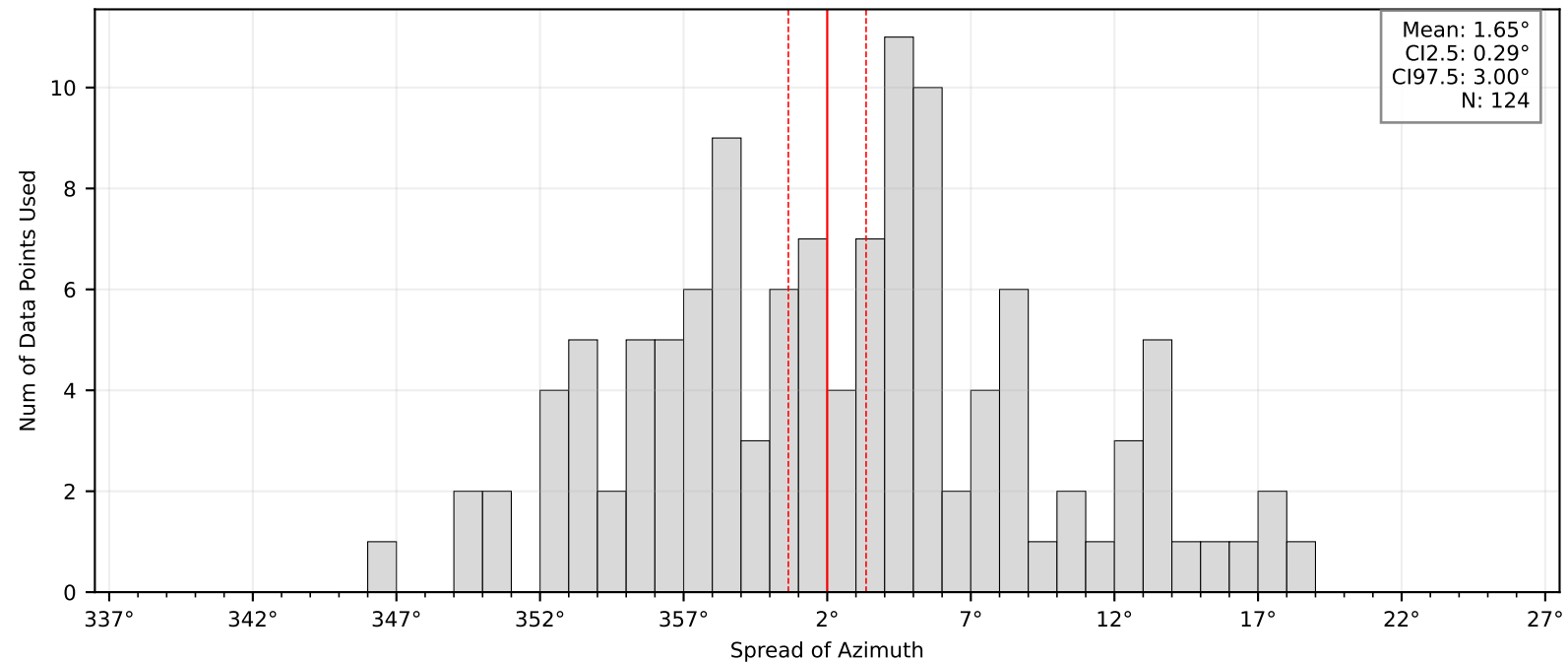
Bootstrap Mean and Confidence Intervals: BK.PRDS
