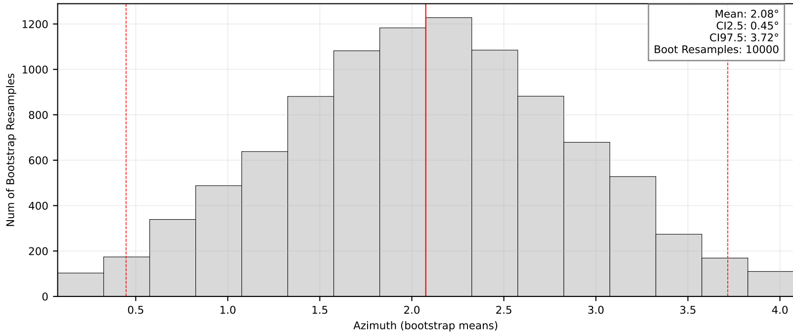
Bootstrap Means/95% CI: BK.PETL
