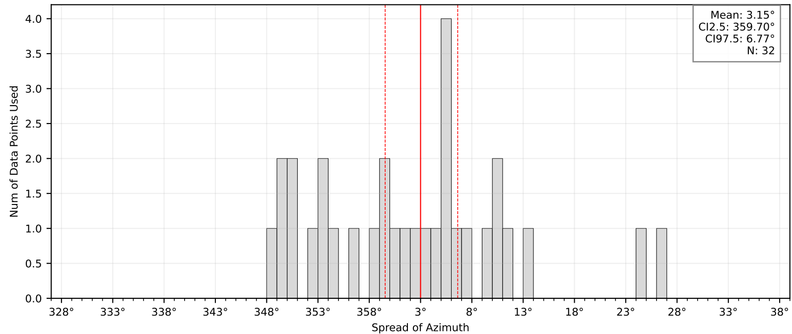
Bootstrap Mean and Confidence Intervals: BK.GRPK
