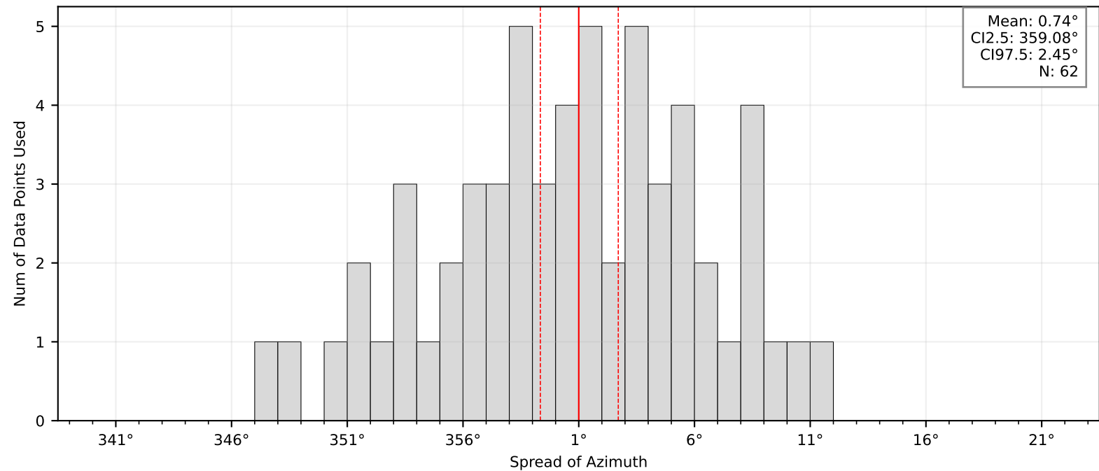
Bootstrap Mean and Confidence Intervals: BK.SFRE
