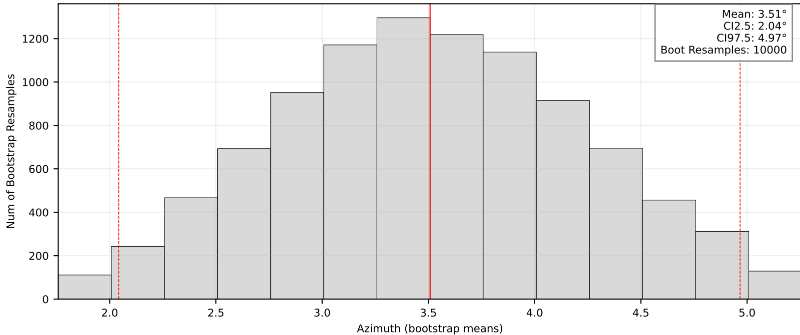
Bootstrap Means/95% CI: BK.SUTB
