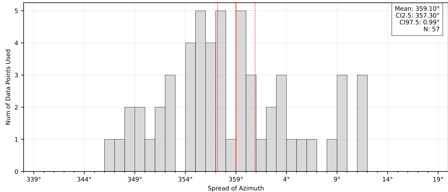
Bootstrap Mean and Confidence Intervals: BK.LSIB
