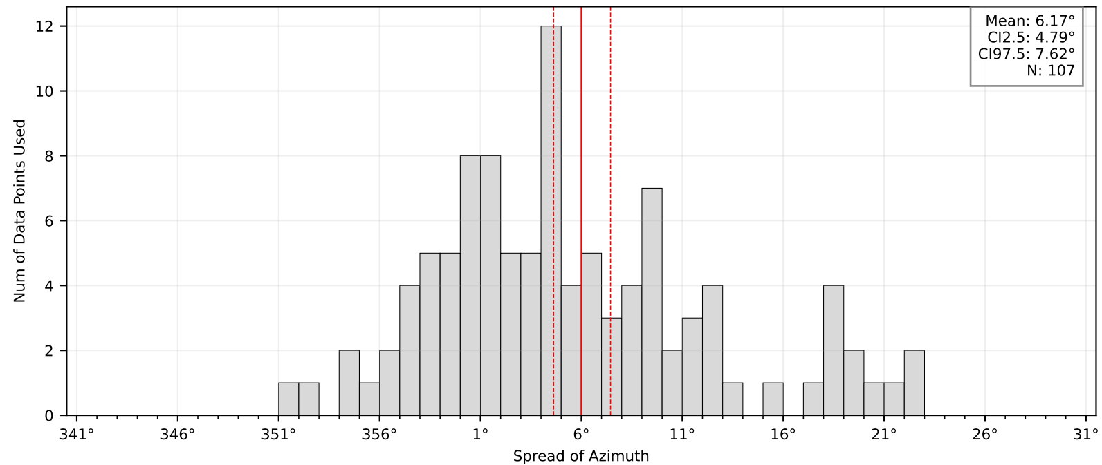
Bootstrap Mean and Confidence Intervals: BK.LCOS
