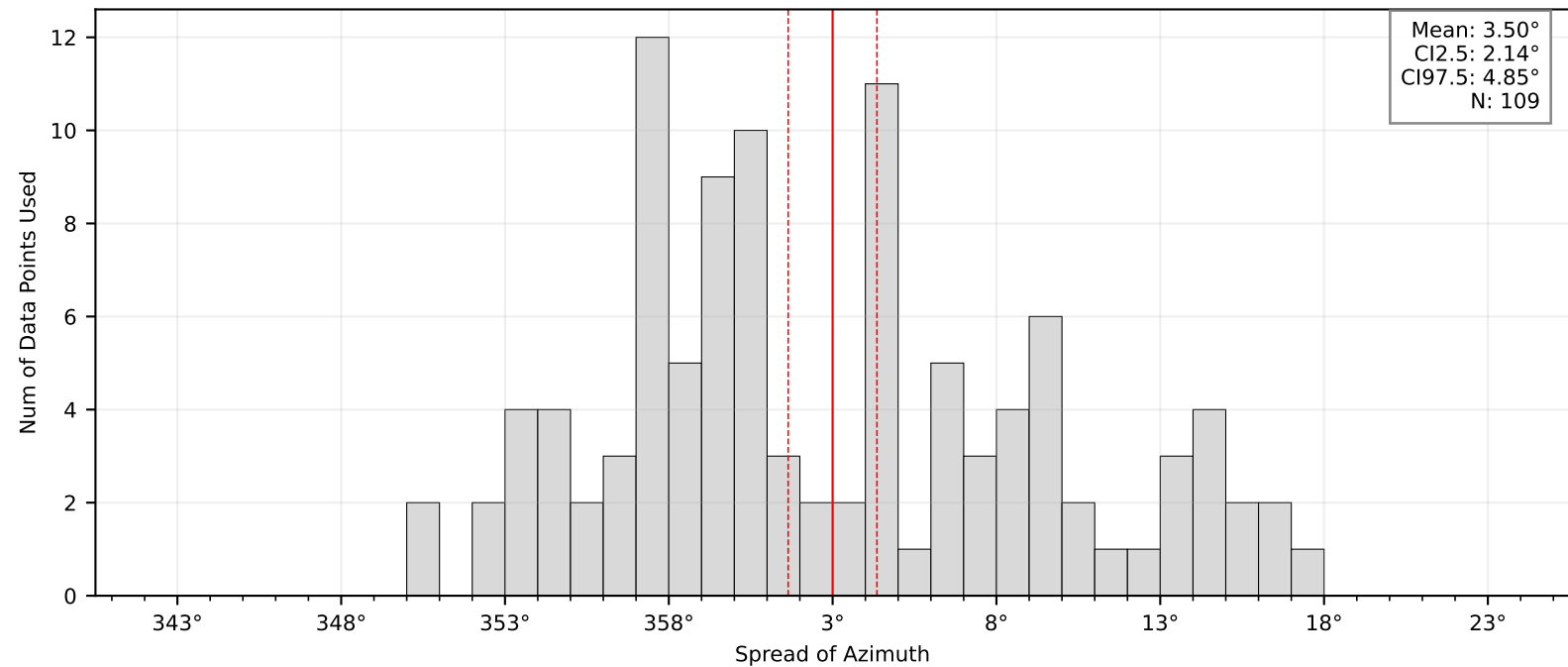
Bootstrap Mean and Confidence Intervals: BK.PBDB
