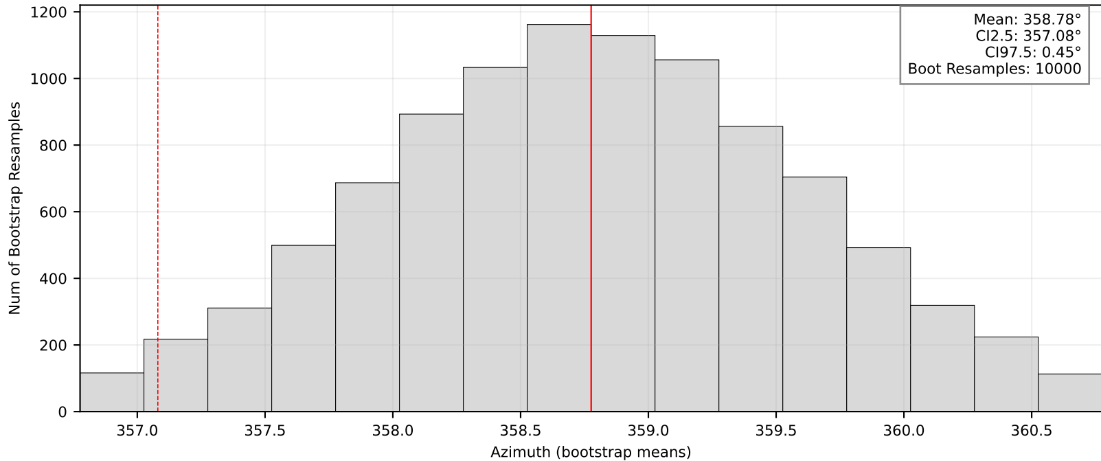
Bootstrap Means/95% CI: BK.BAKR
