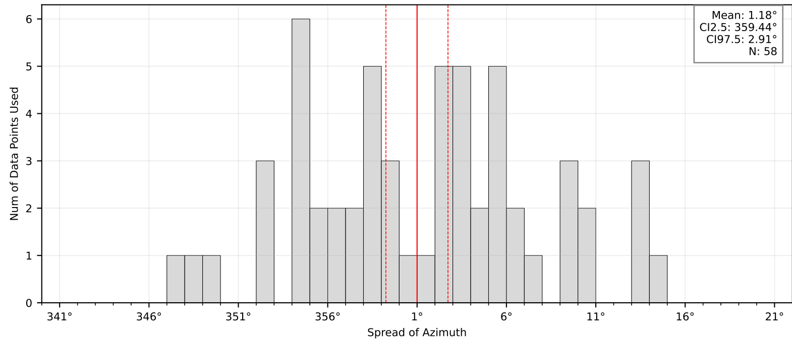
Bootstrap Mean and Confidence Intervals: BK.PACP
