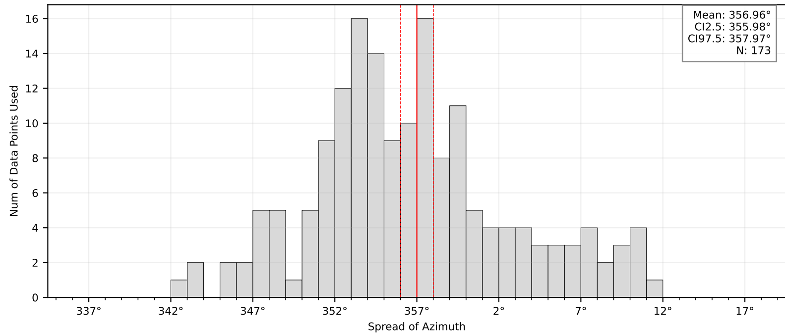
Bootstrap Mean and Confidence Intervals: BK.PESC
