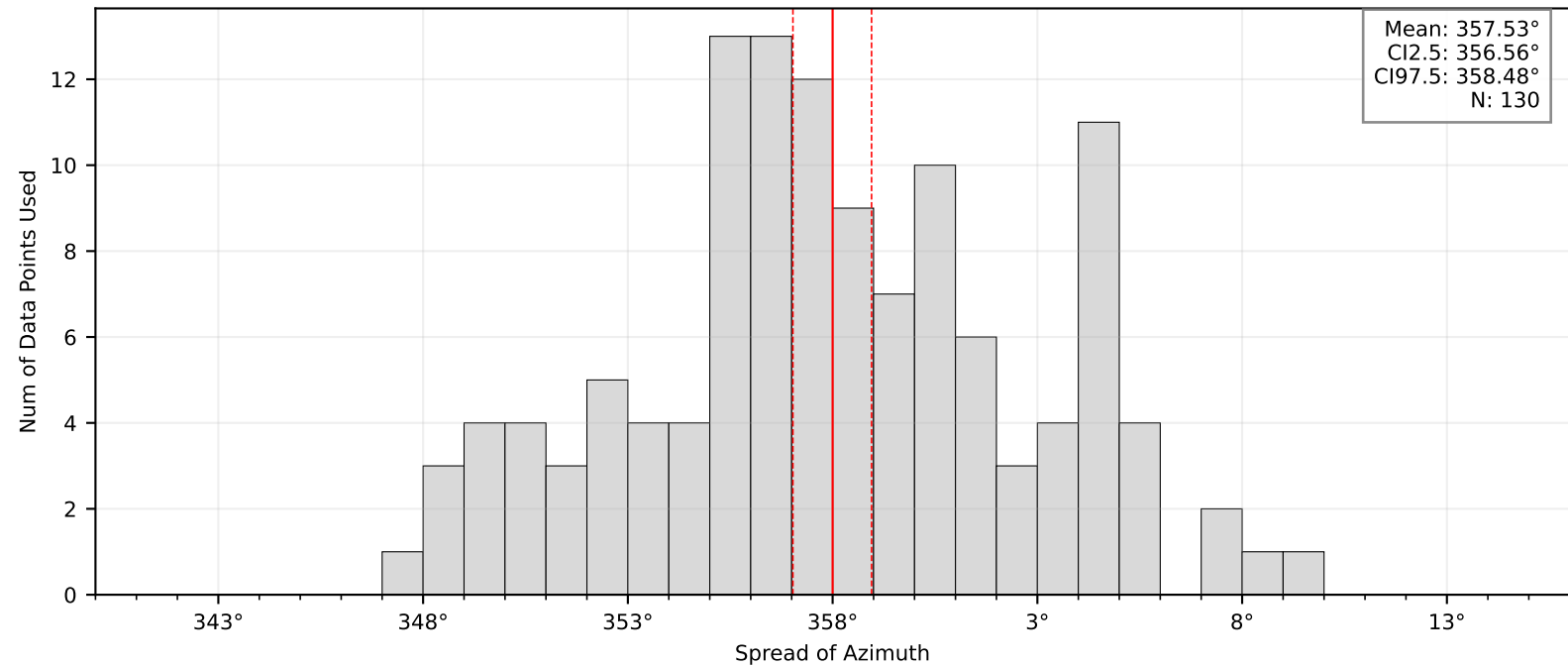
Bootstrap Mean and Confidence Intervals: BK.JEPS
