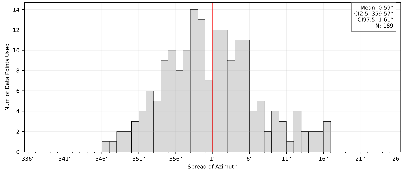
Bootstrap Mean and Confidence Intervals: BK.HRCH
