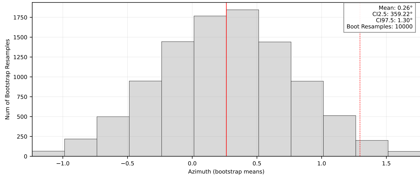
Bootstrap Means/95% CI: BK.WSRE
