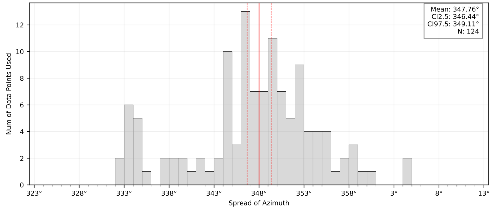
Bootstrap Mean and Confidence Intervals: BK.BIGV
