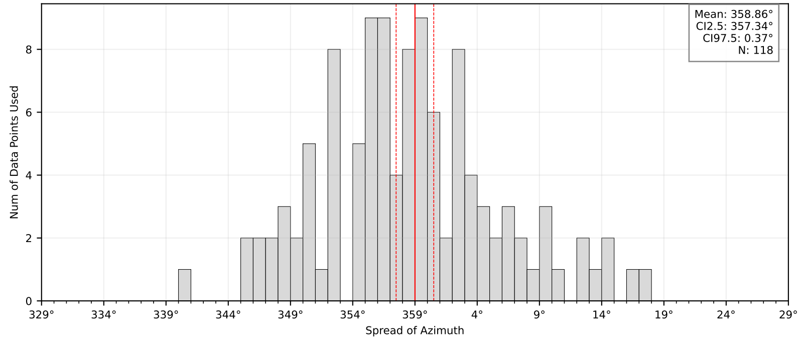
Bootstrap Mean and Confidence Intervals: BK.DIAZ
