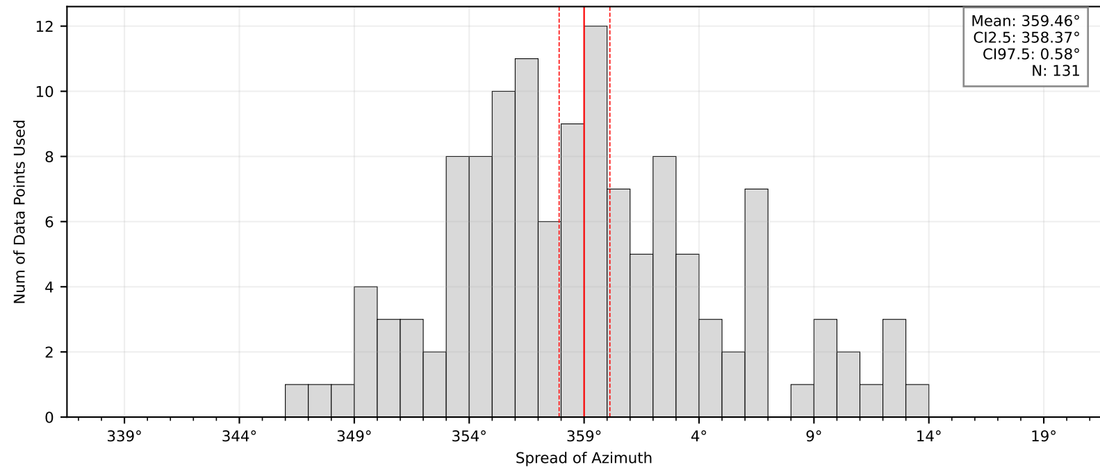
Bootstrap Mean and Confidence Intervals: BK.RVRP
