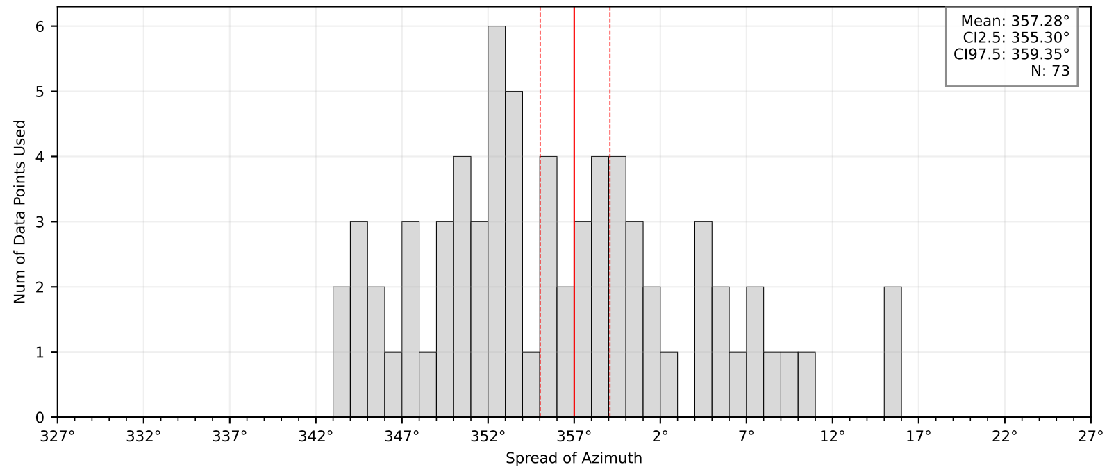
Bootstrap Mean and Confidence Intervals: BK.GTSB
