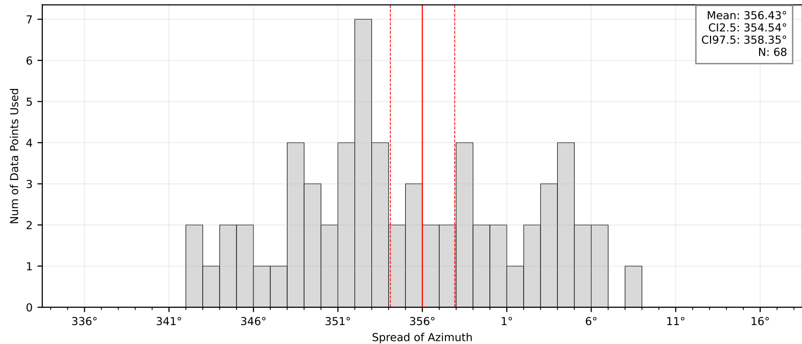
Bootstrap Mean and Confidence Intervals: BK.HULL
