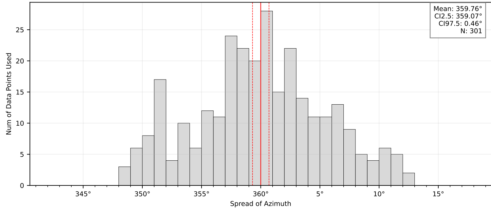
Bootstrap Mean and Confidence Intervals: BK.MTOS
