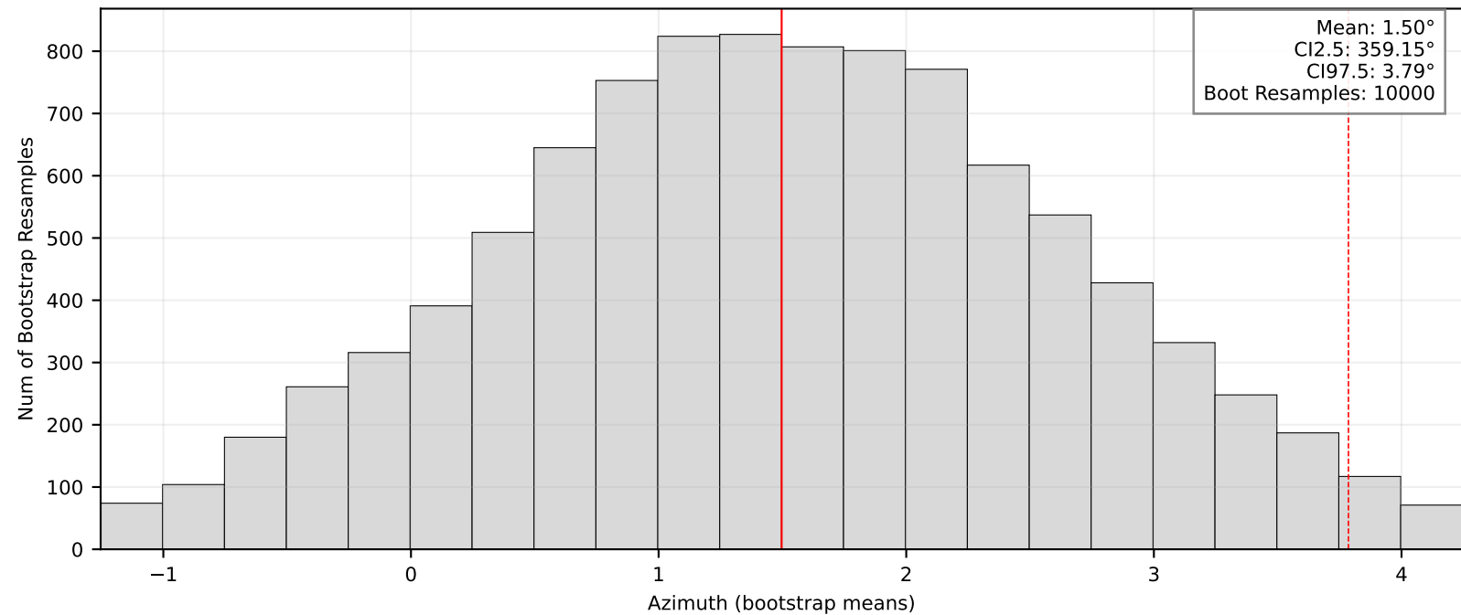
Bootstrap Means/95% CI: BK.DMOR
