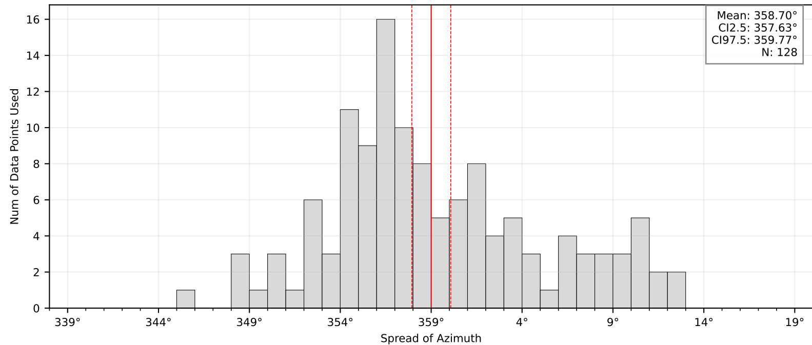
Bootstrap Mean and Confidence Intervals: BK.TESL
