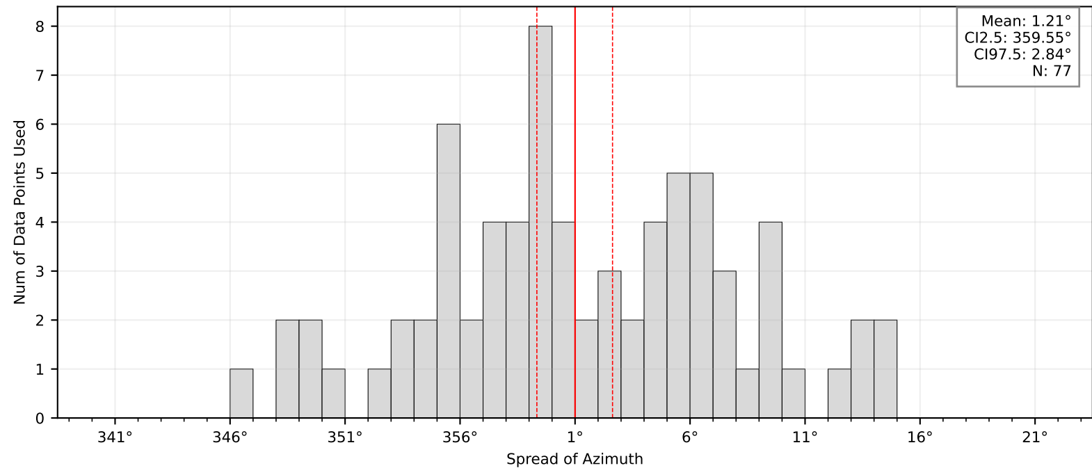
Bootstrap Mean and Confidence Intervals: BK.KRUG
