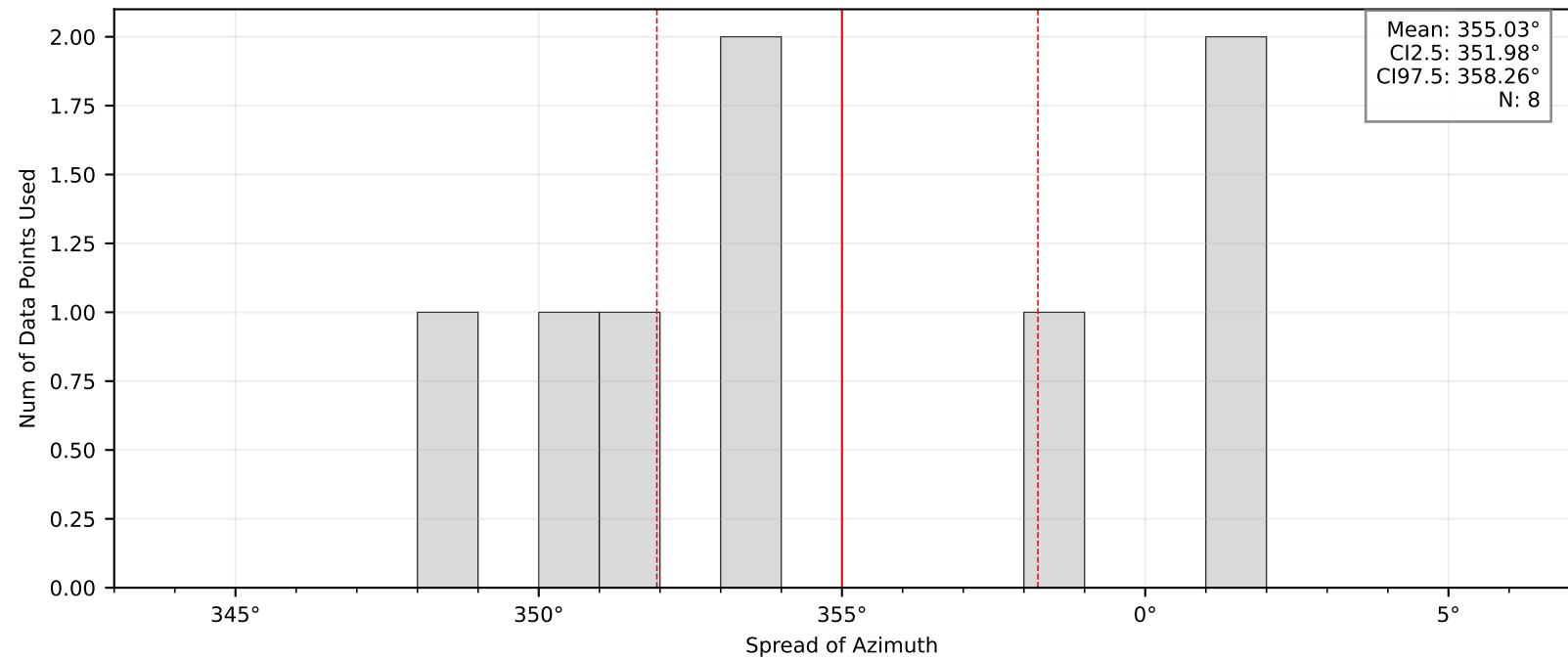
Bootstrap Mean and Confidence Intervals: BK.KRUG
