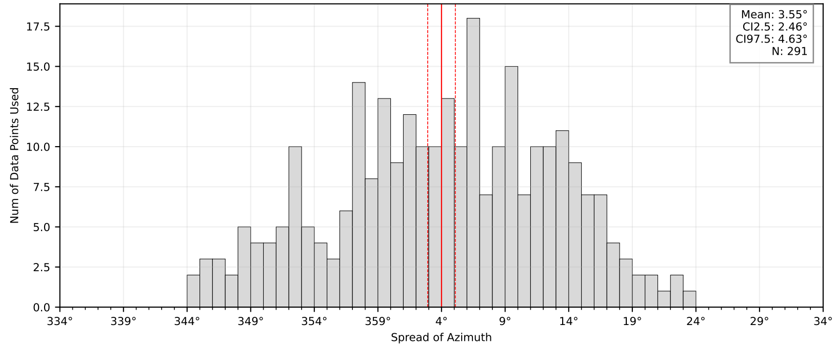
Bootstrap Mean and Confidence Intervals: BK.CVS
