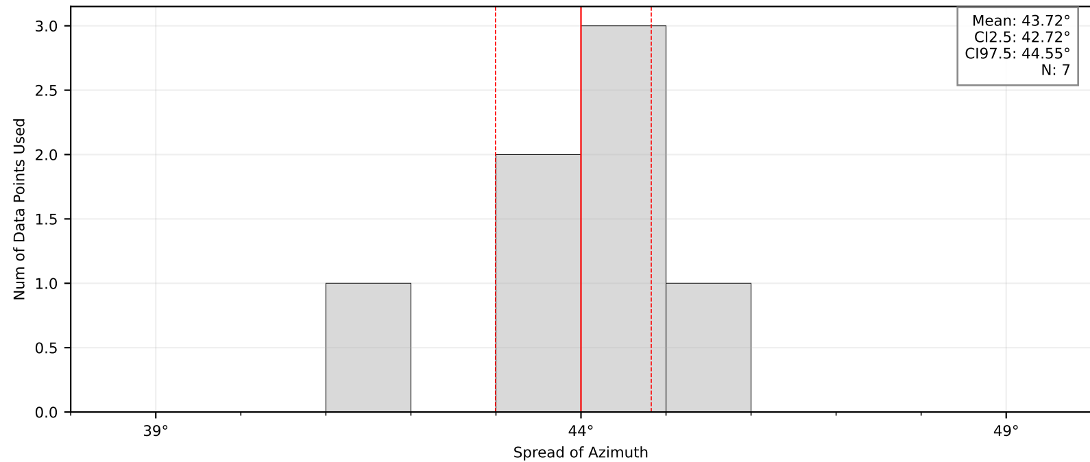
Bootstrap Mean and Confidence Intervals: BK.PORG
