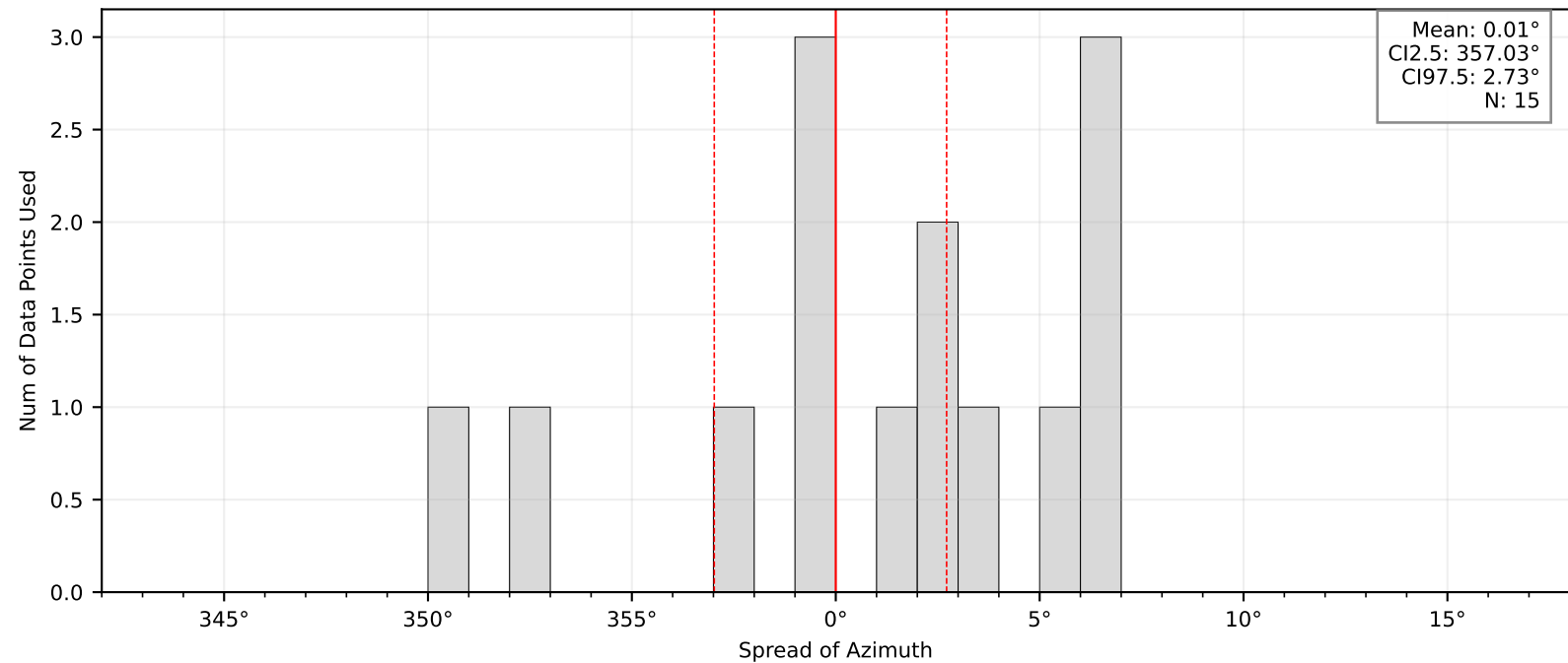
Bootstrap Mean and Confidence Intervals: BK.HRCH
