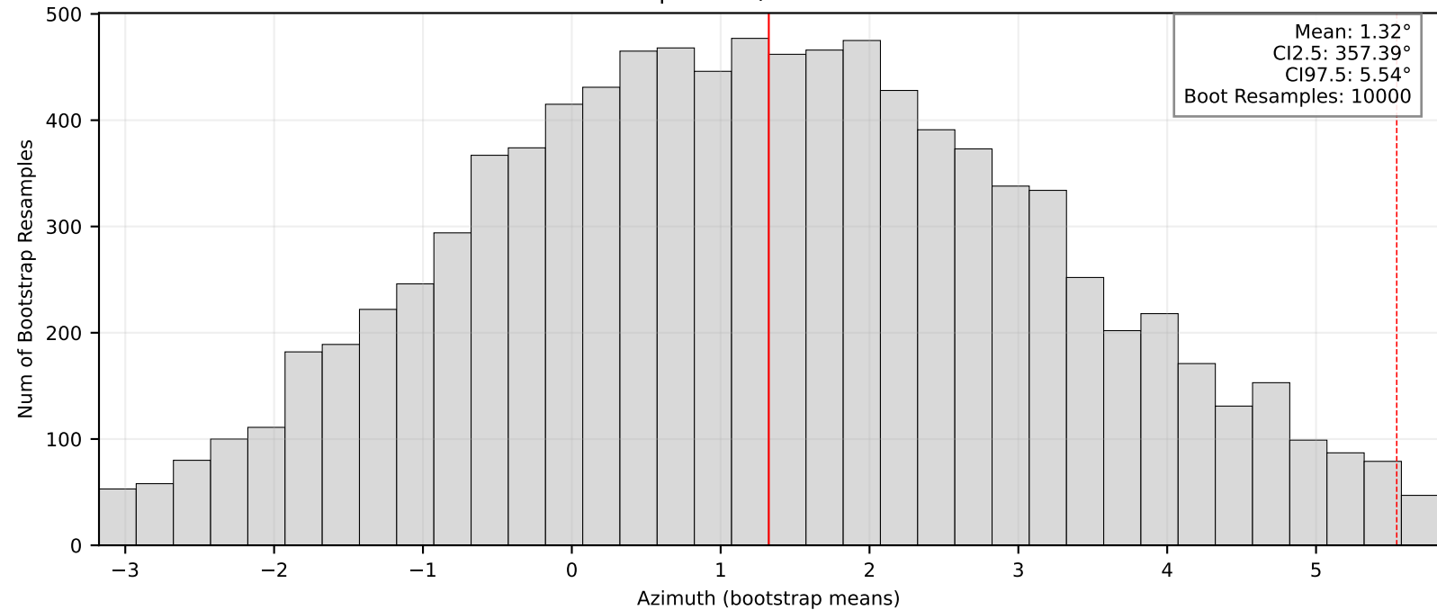
Bootstrap Means/95% CI: BK.THOM
