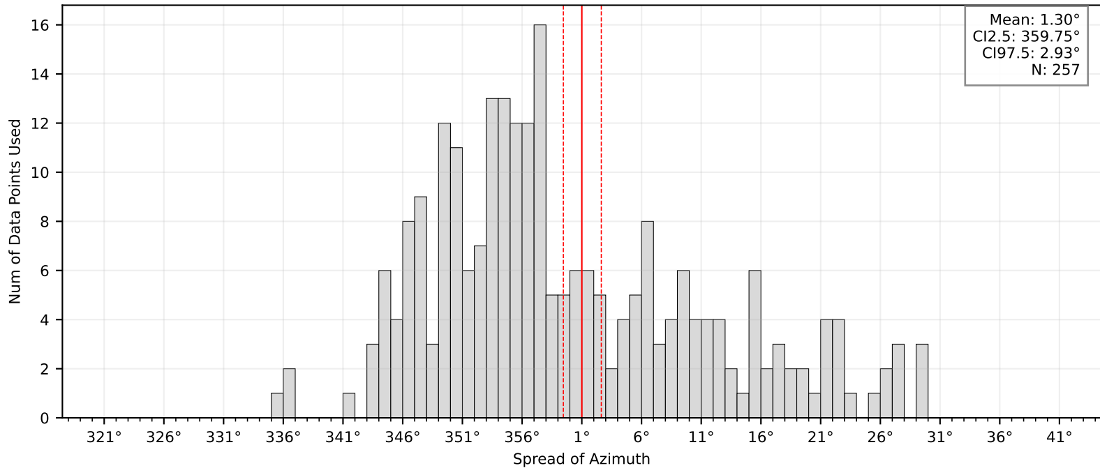
Bootstrap Mean and Confidence Intervals: BK.OVRO
