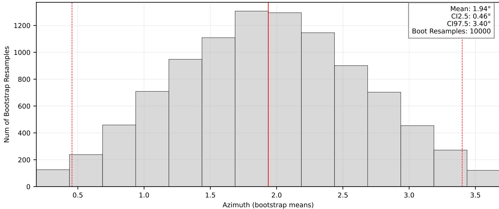
Bootstrap Means/95% CI: BK.CCOR
