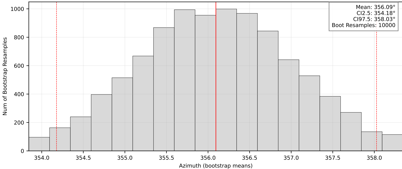
Bootstrap Means/95% CI: BK.GHOP
