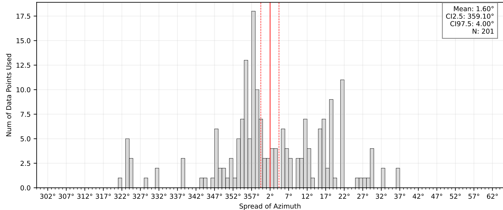
Bootstrap Mean and Confidence Intervals: BK.BUCR
