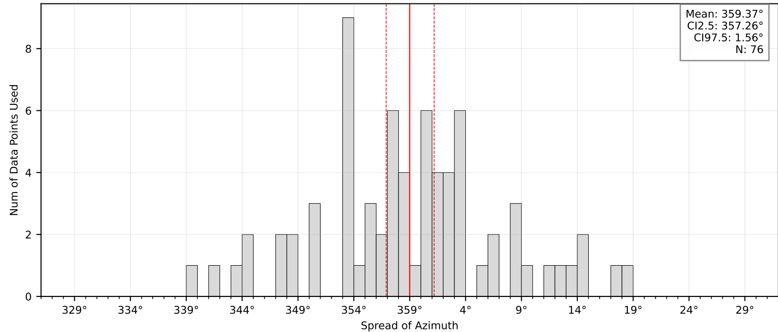
Bootstrap Mean and Confidence Intervals: BK.SBAR
