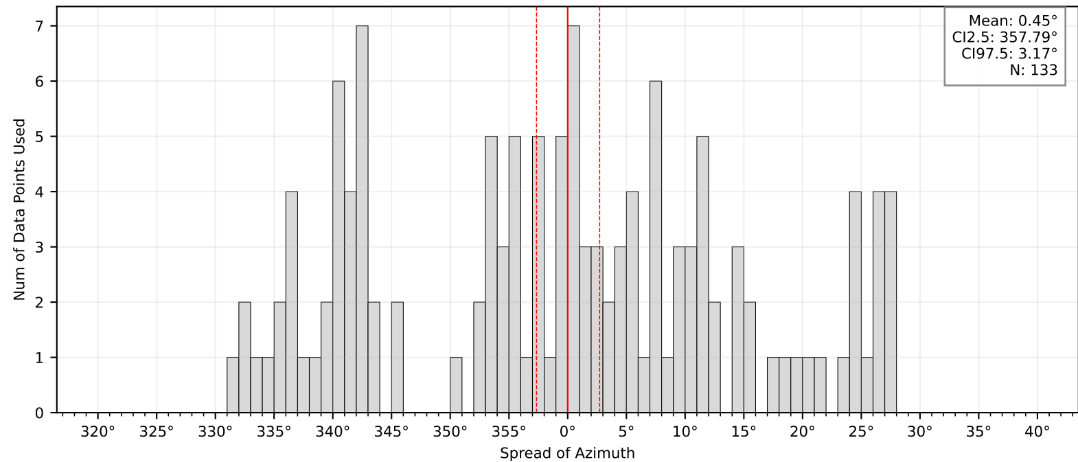
Bootstrap Mean and Confidence Intervals: BK.RAMR
