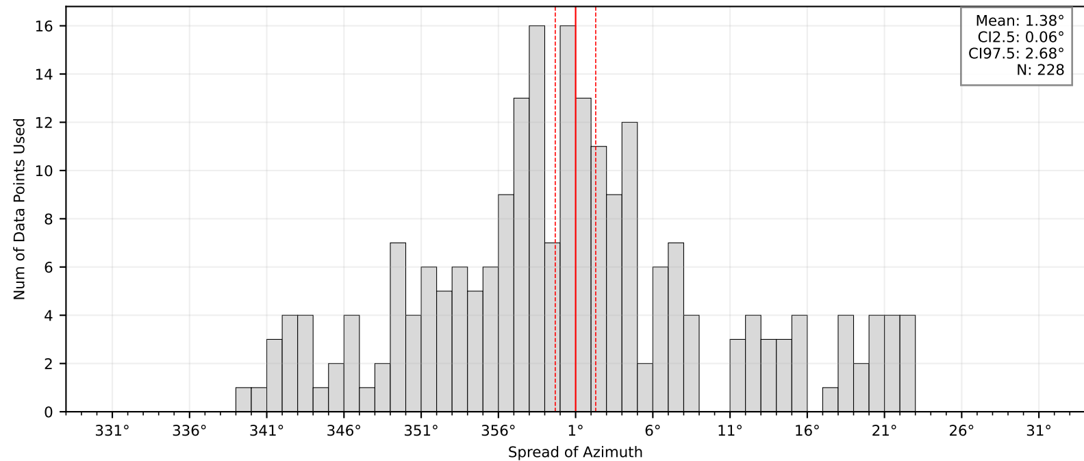
Bootstrap Mean and Confidence Intervals: BK.BLUE
