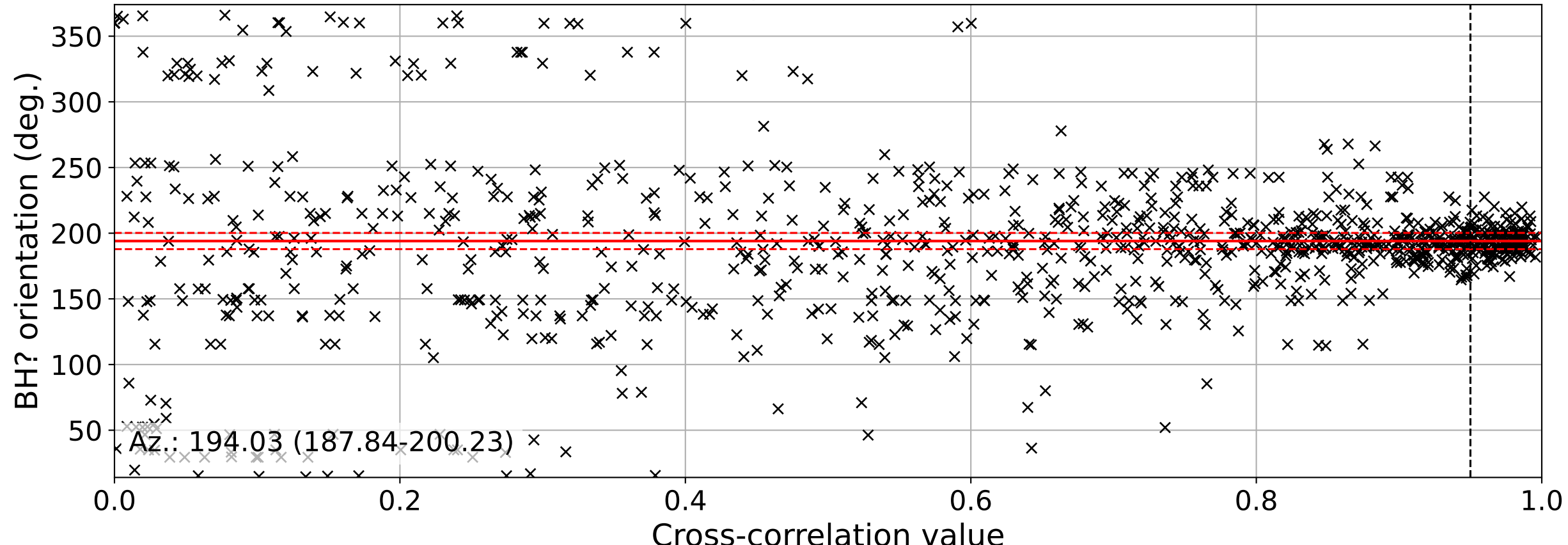
DLOPy result BK.LCUV
