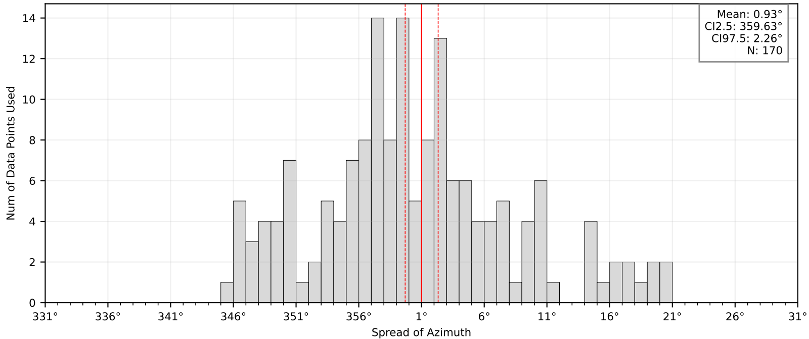
Bootstrap Mean and Confidence Intervals: BK.TSCN
