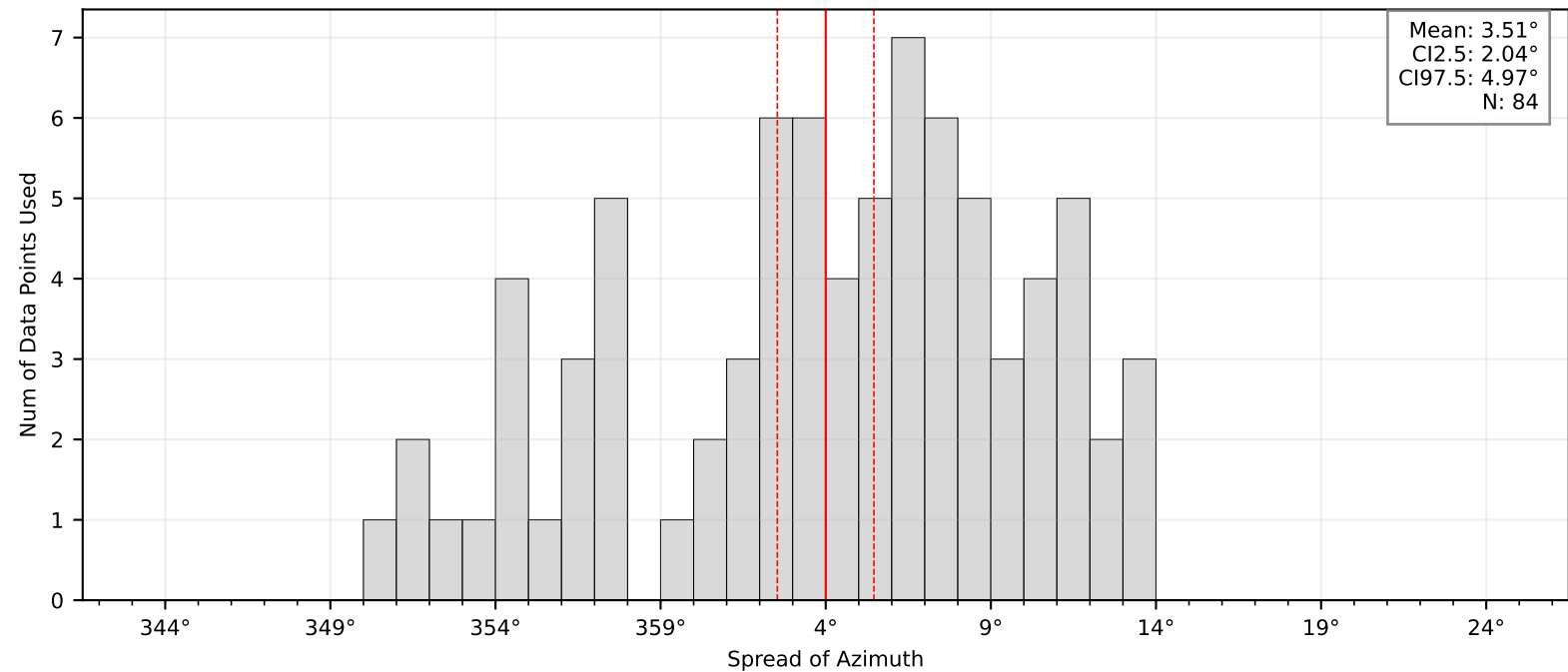
Bootstrap Mean and Confidence Intervals: BK.SUTB
