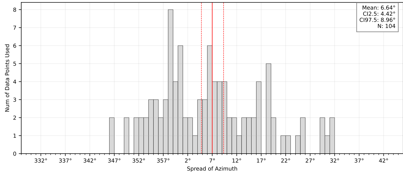
Bootstrap Mean and Confidence Intervals: BK.KARE
