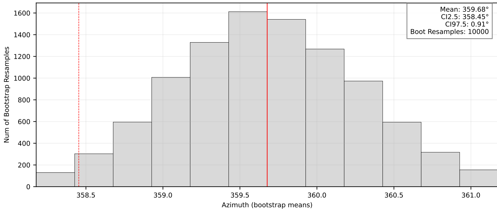
Bootstrap Means/95% CI: BK.TESL
