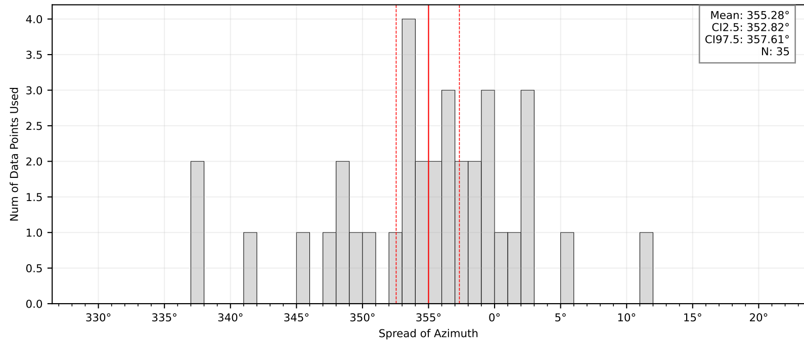
Bootstrap Mean and Confidence Intervals: BK.MKOF
