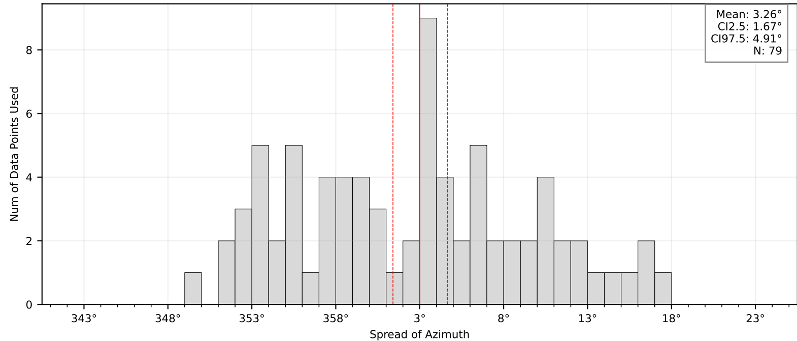
Bootstrap Mean and Confidence Intervals: BK.SKGS
