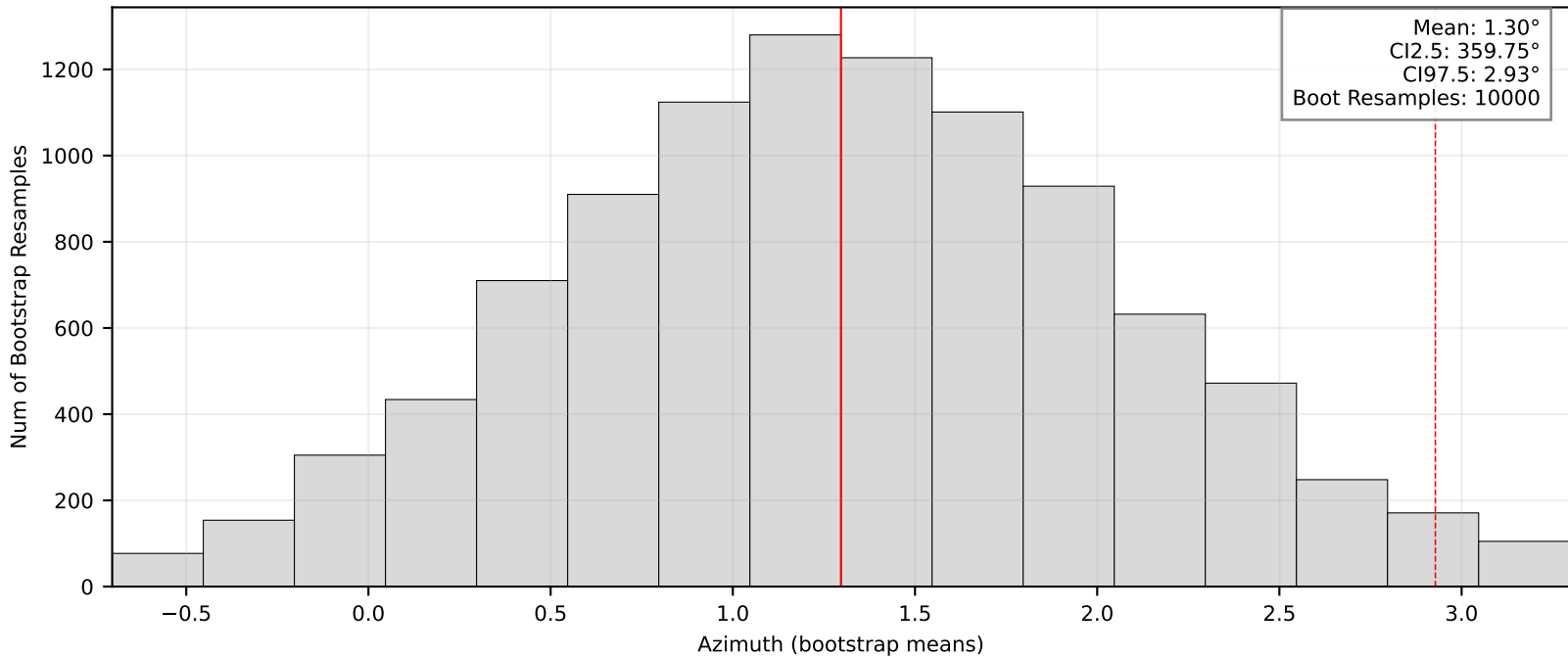
Bootstrap Means/95% CI: BK.OVRO
