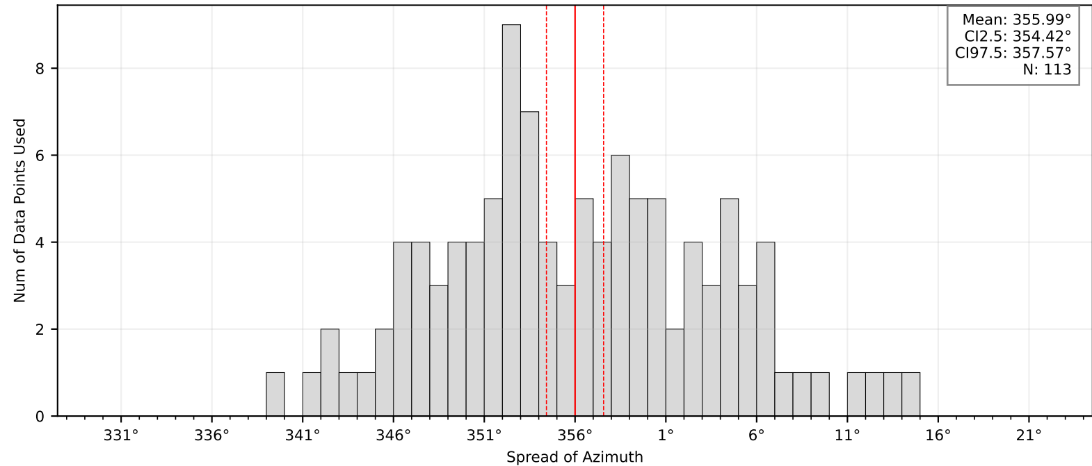
Bootstrap Mean and Confidence Intervals: BK.AZUL
