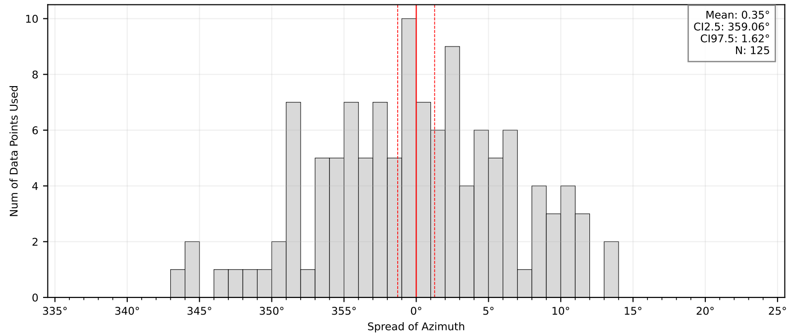
Bootstrap Mean and Confidence Intervals: BK.WHMT
