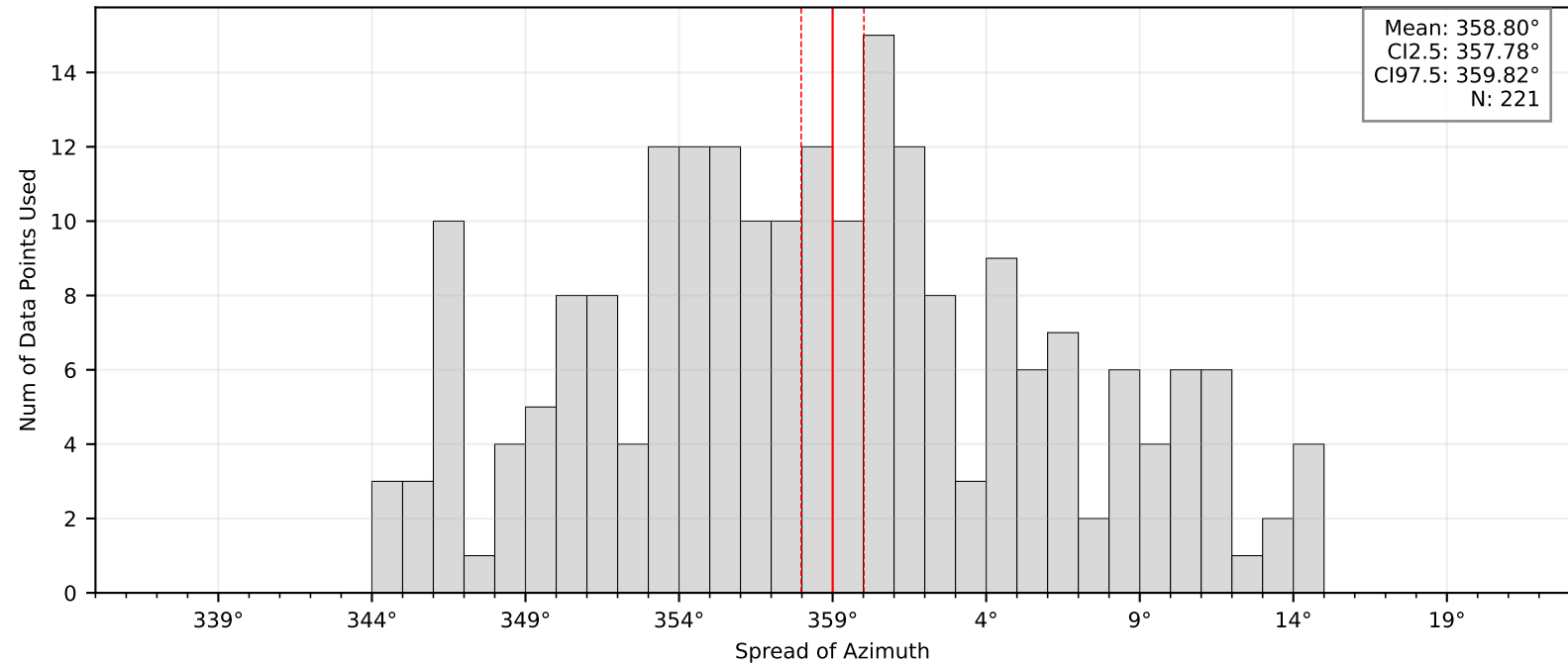
Bootstrap Mean and Confidence Intervals: BK.HAS2
