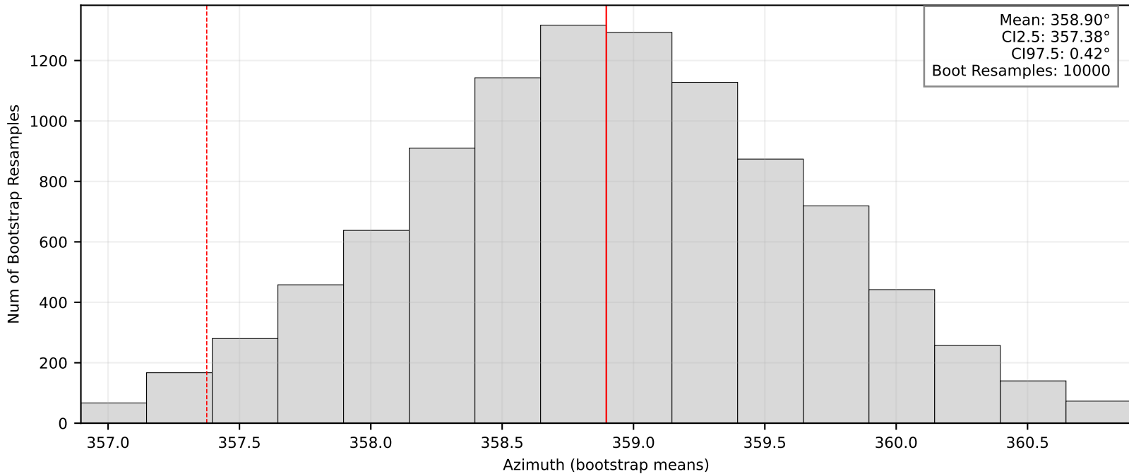
Bootstrap Means/95% CI: BK.AVSP
