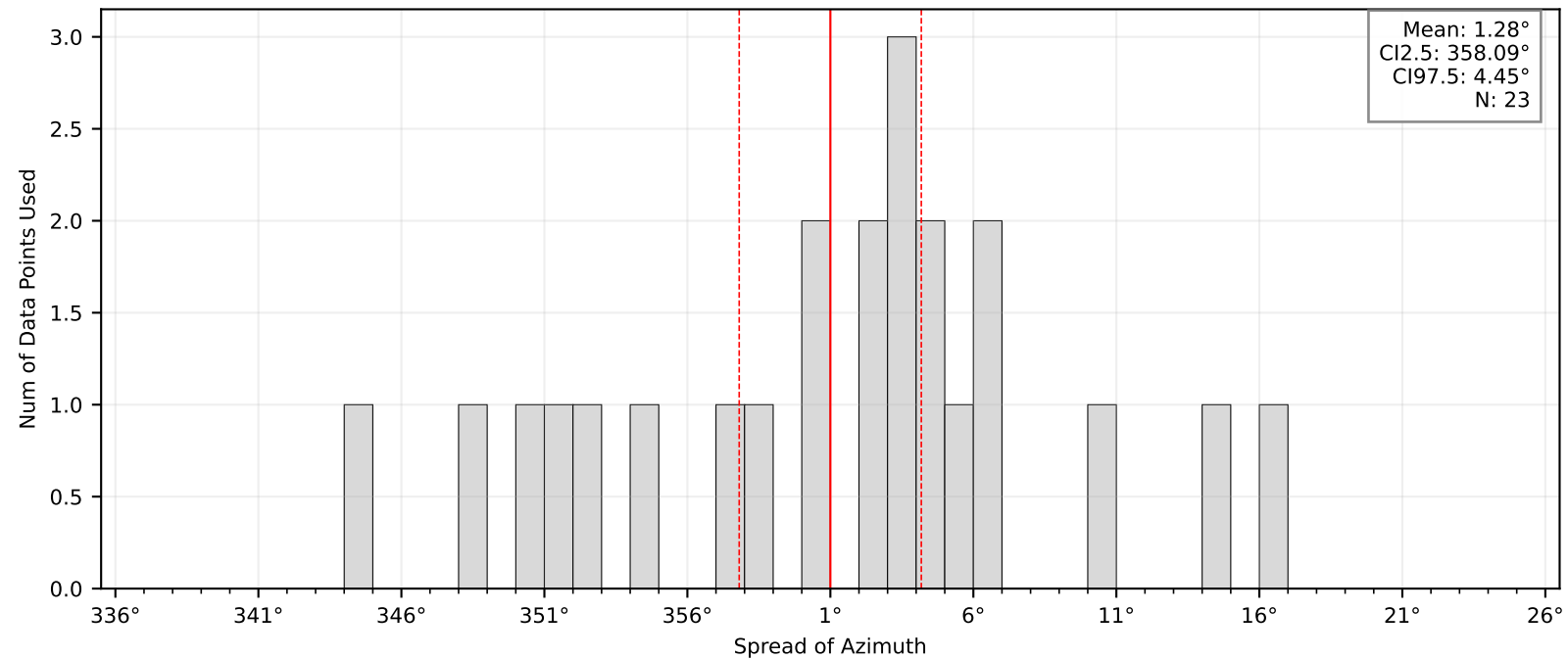
Bootstrap Mean and Confidence Intervals: BK.BJES
