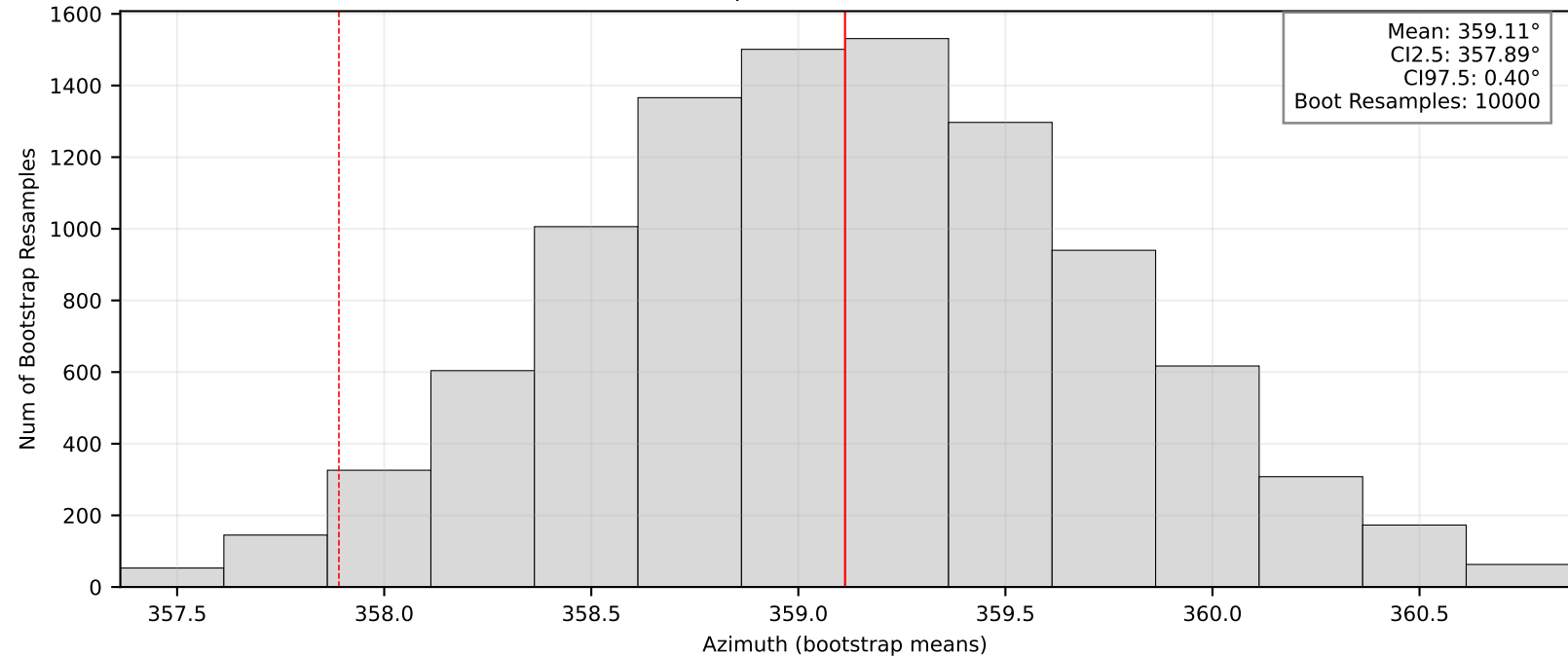
Bootstrap Means/95% CI: BK.BUCI
