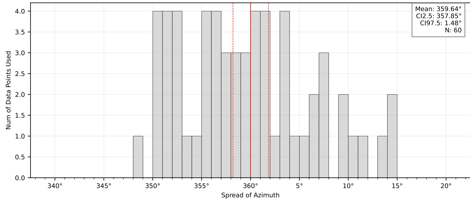
Bootstrap Mean and Confidence Intervals: BK.PETY
