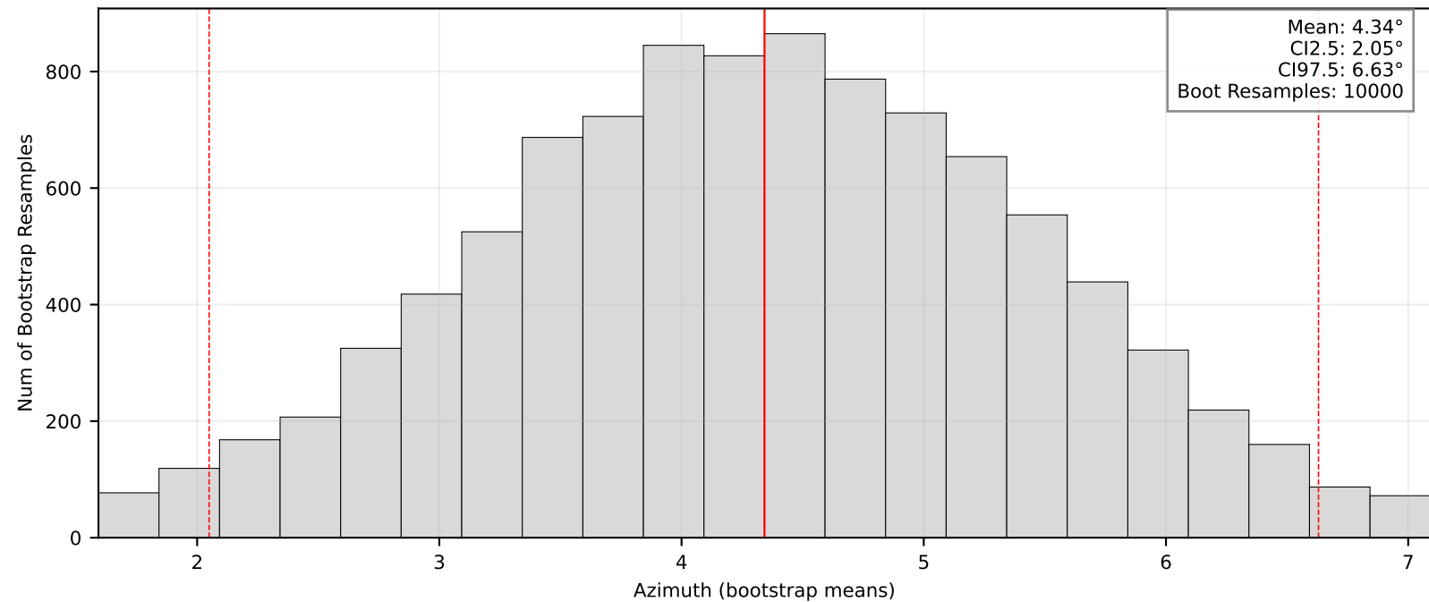
Bootstrap Means/95% CI: BK.LEGD
