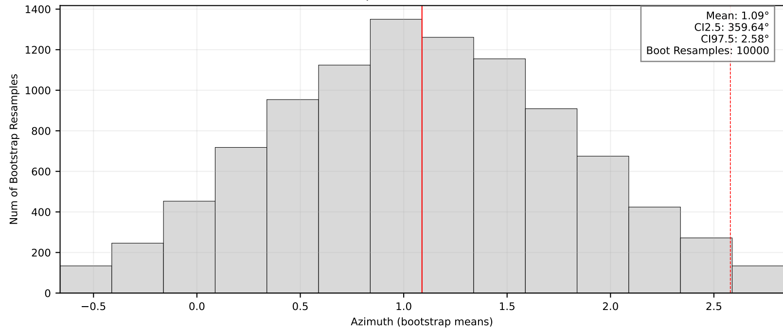
Bootstrap Means/95% CI: BK.RIMR
