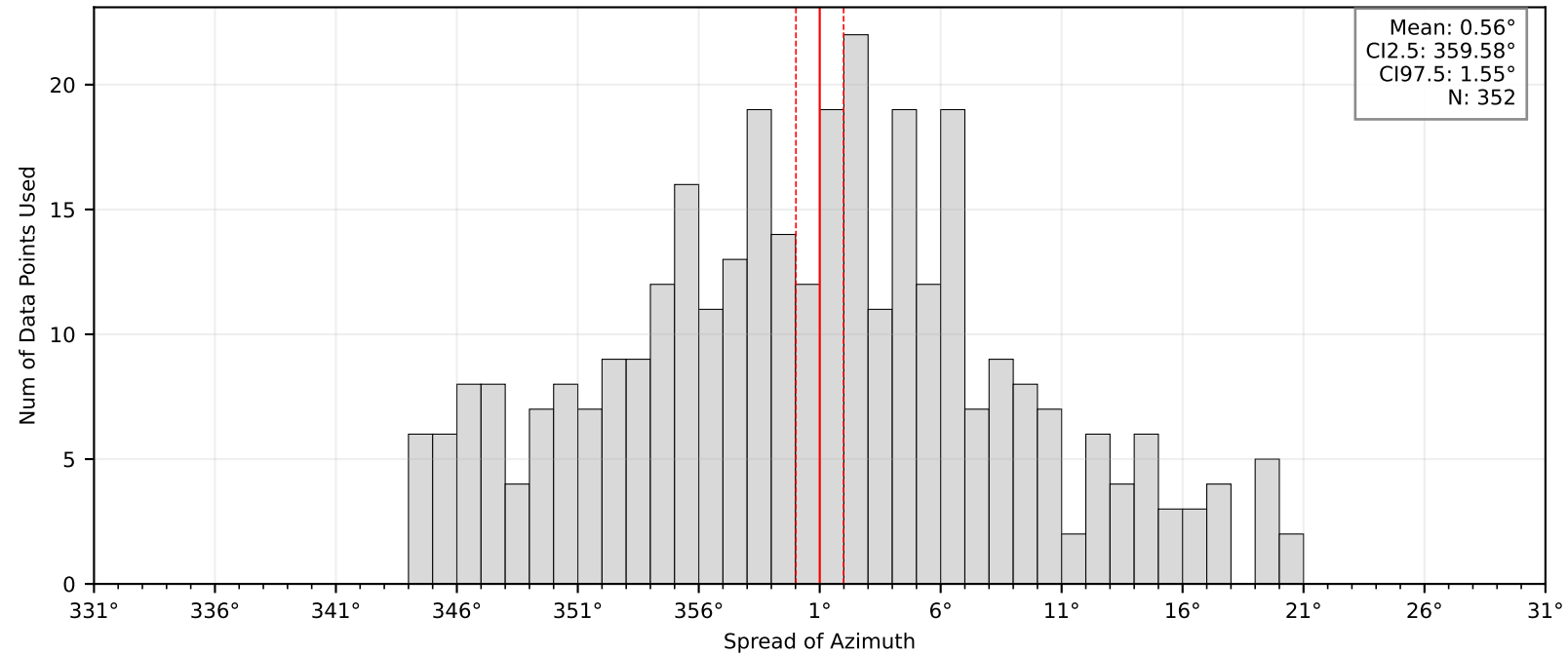
Bootstrap Mean and Confidence Intervals: BK.CMB
