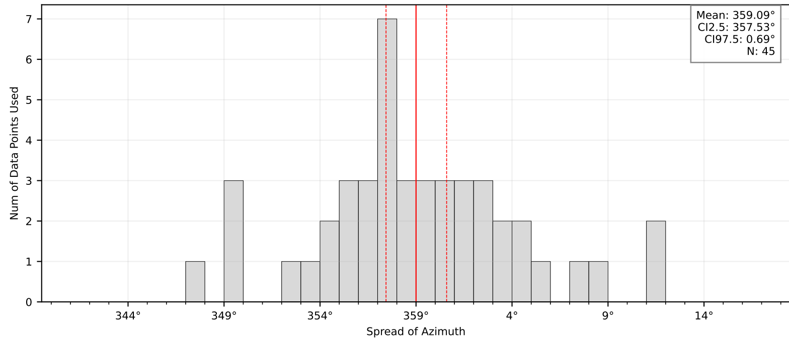
Bootstrap Mean and Confidence Intervals: BK.SIGP
