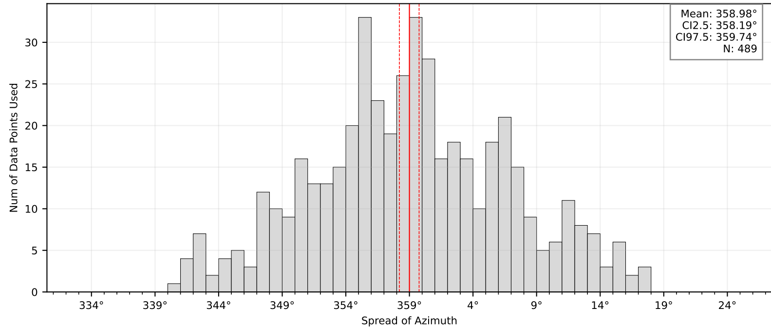
Bootstrap Mean and Confidence Intervals: BK.MCCM
