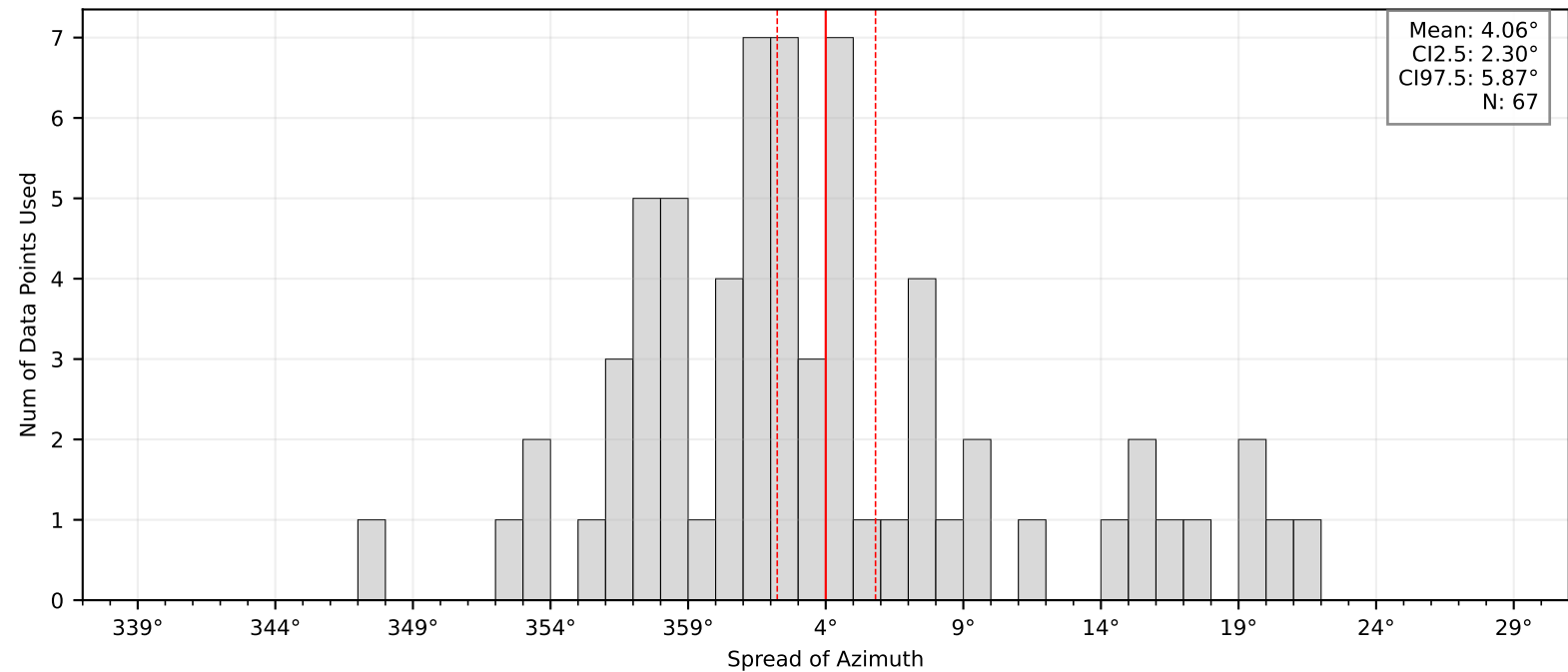
Bootstrap Mean and Confidence Intervals: BK.SNCR
