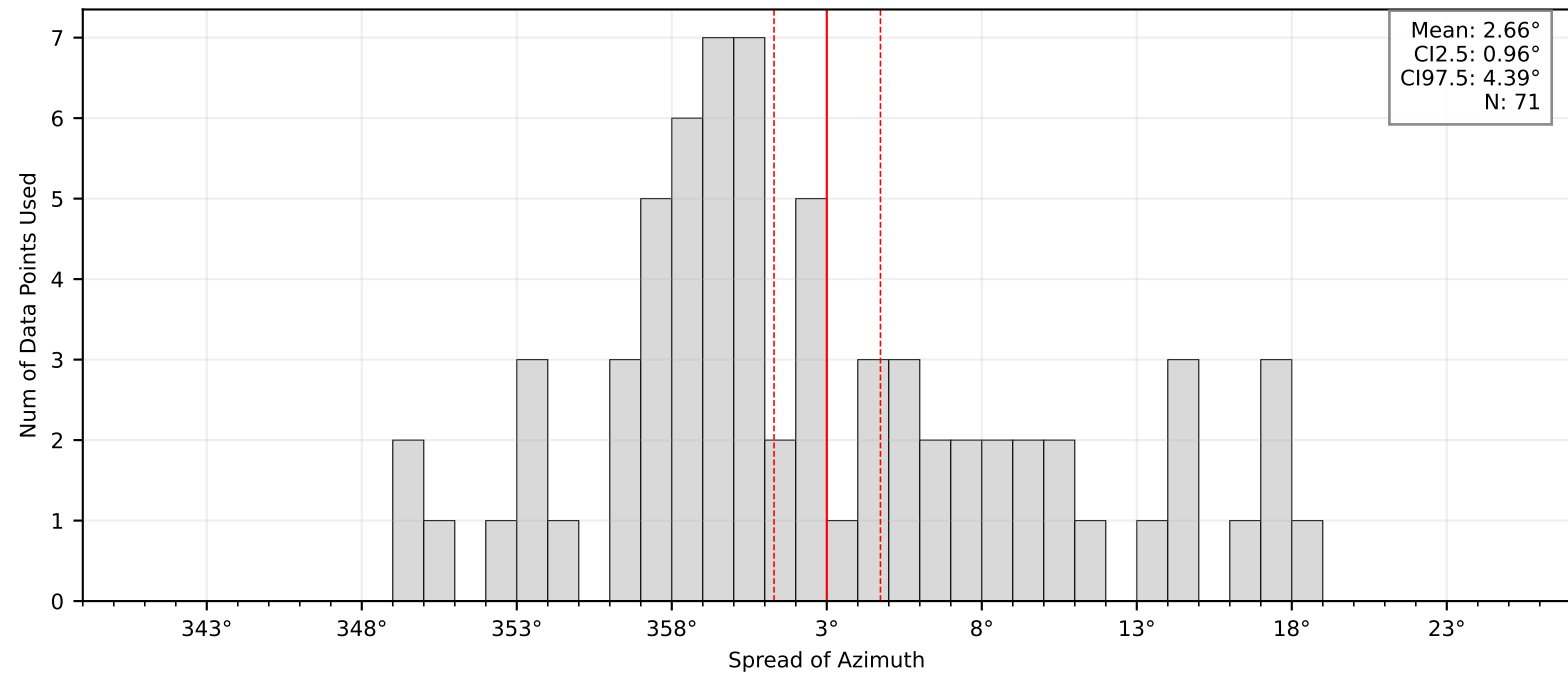
Bootstrap Mean and Confidence Intervals: BK.SUGR
