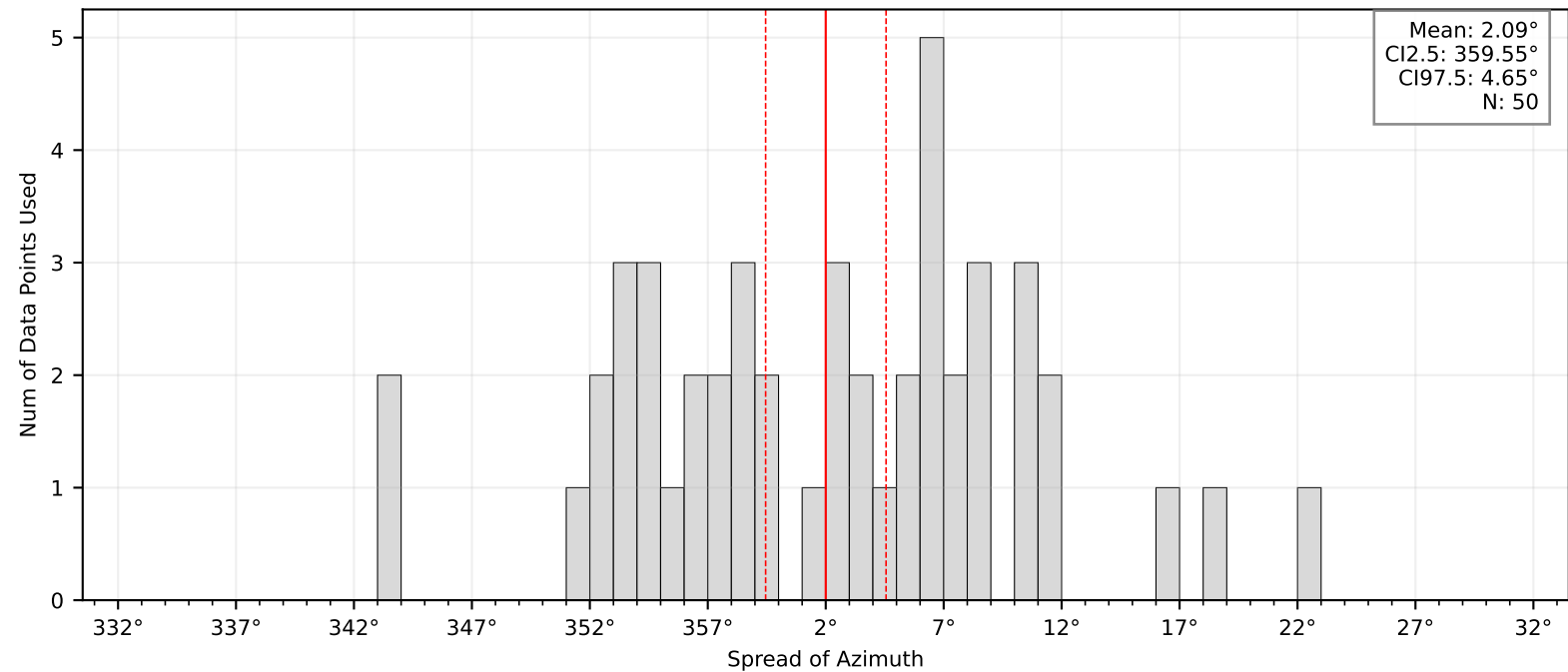
Bootstrap Mean and Confidence Intervals: BK.HUNT
