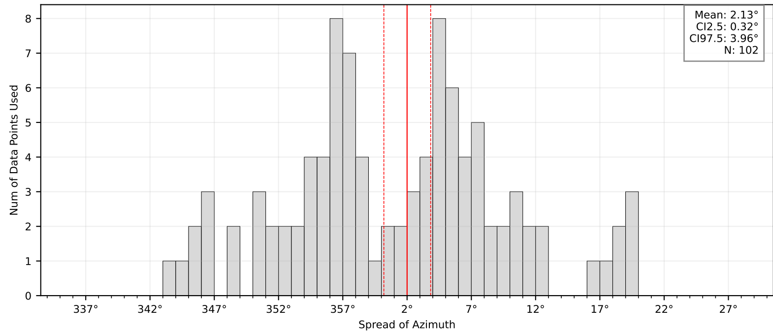
Bootstrap Mean and Confidence Intervals: BK.CMB
