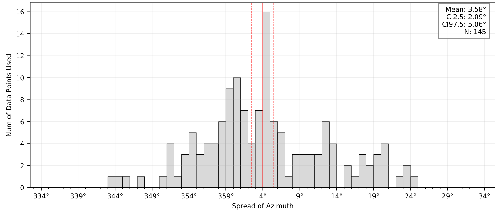
Bootstrap Mean and Confidence Intervals: BK.OAKV
