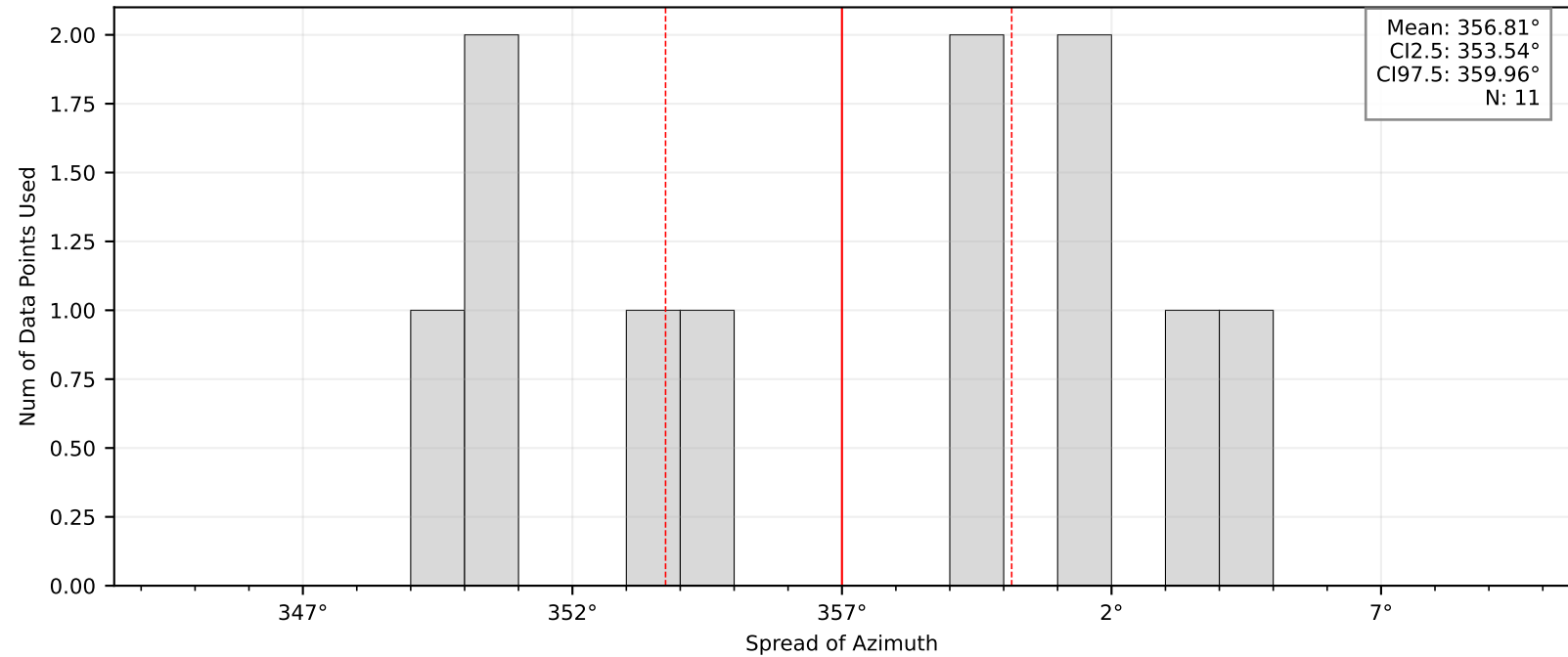
Bootstrap Mean and Confidence Intervals: BK.HAST
