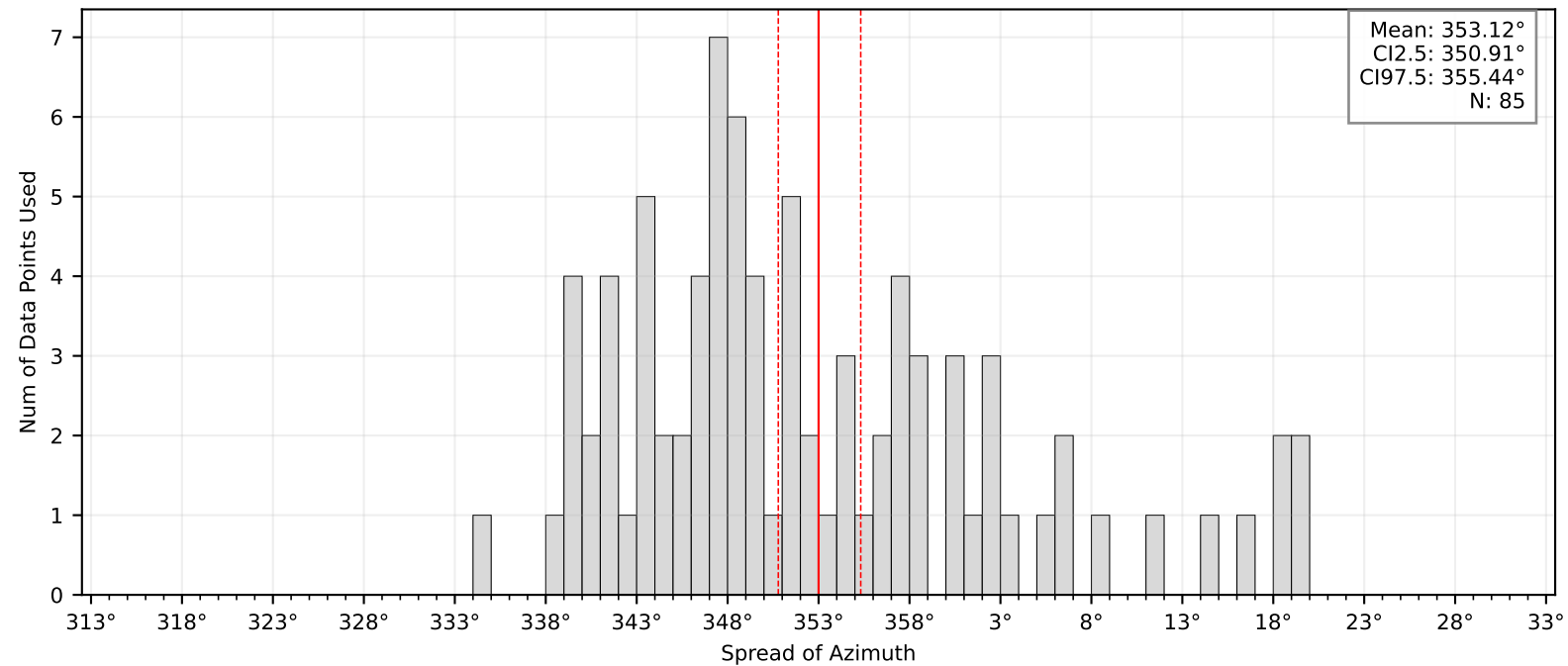
Bootstrap Mean and Confidence Intervals: BK.BIGV
