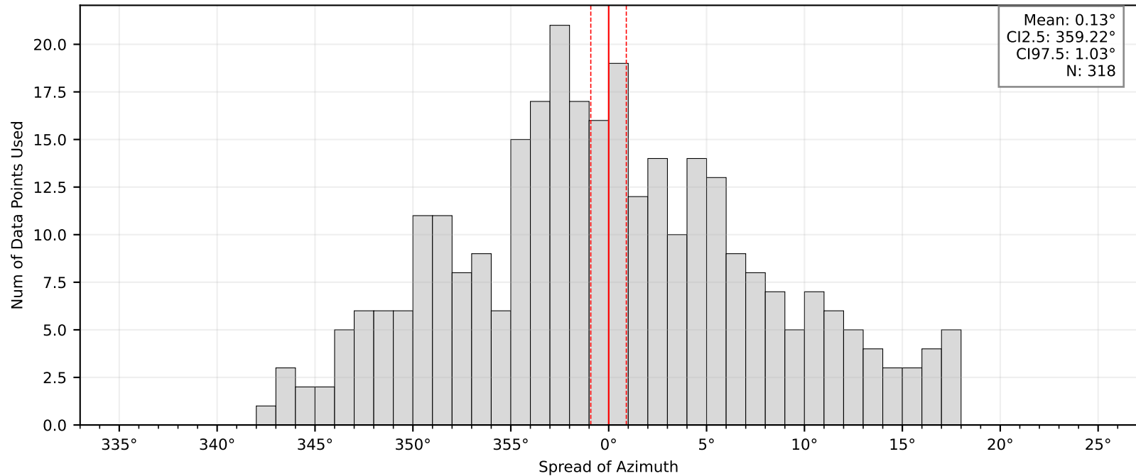
Bootstrap Mean and Confidence Intervals: BK.VAK
