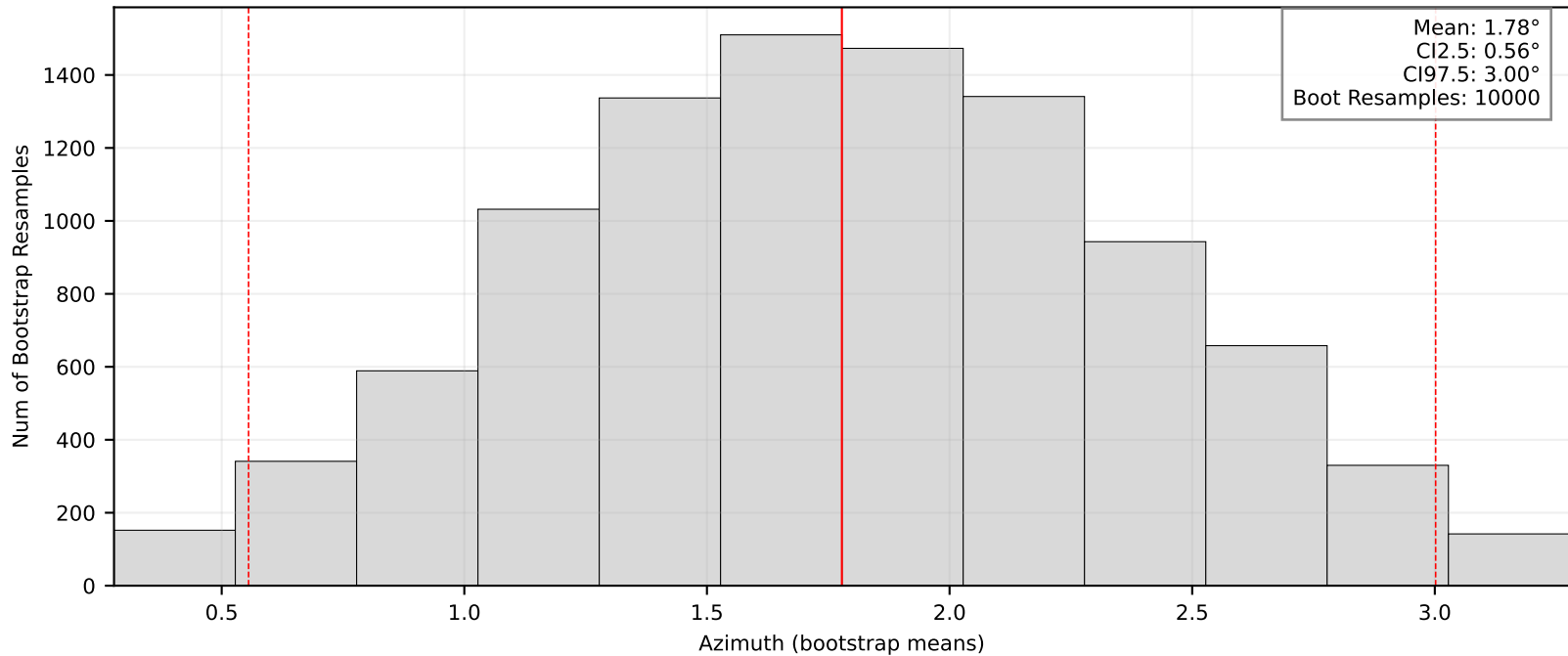
Bootstrap Means/95% CI: BK.ROMB
