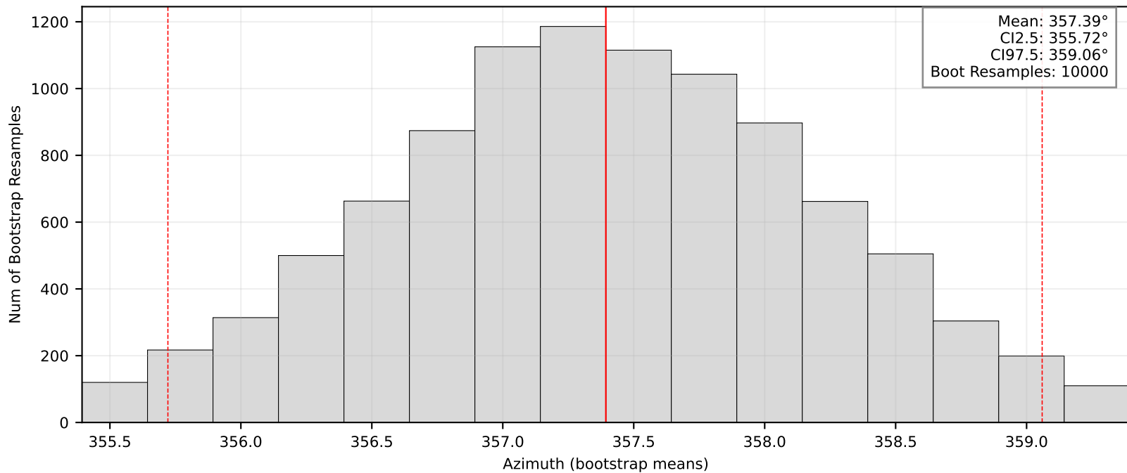
Bootstrap Means/95% CI: BK.WLKR
