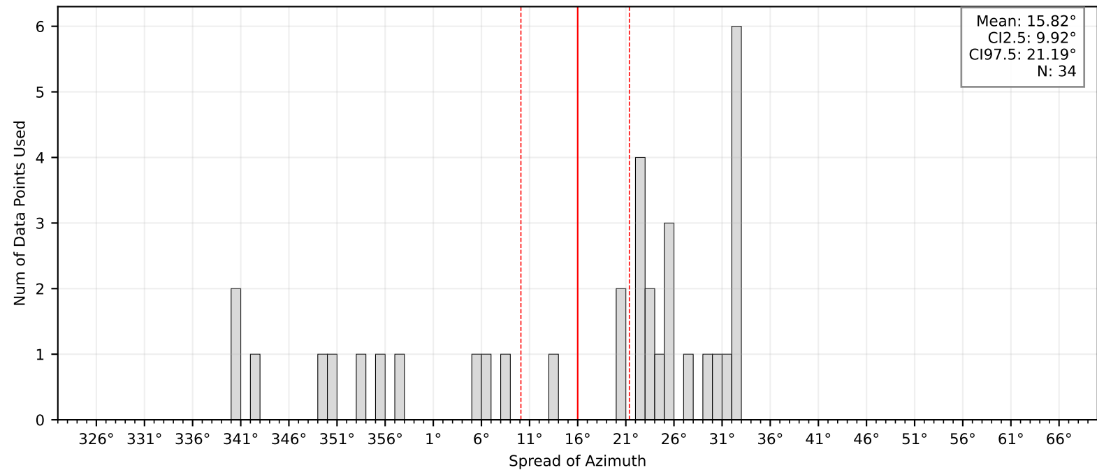
Bootstrap Mean and Confidence Intervals: BK.SCZ
