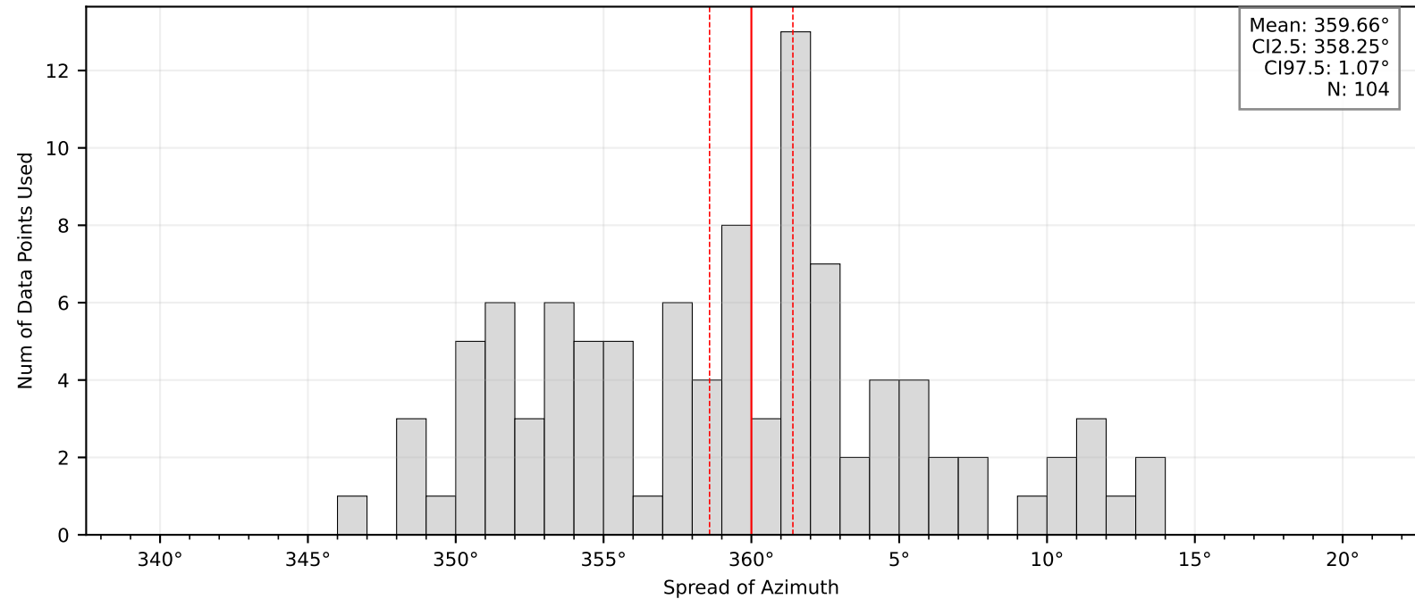
Bootstrap Mean and Confidence Intervals: BK.KNEE
