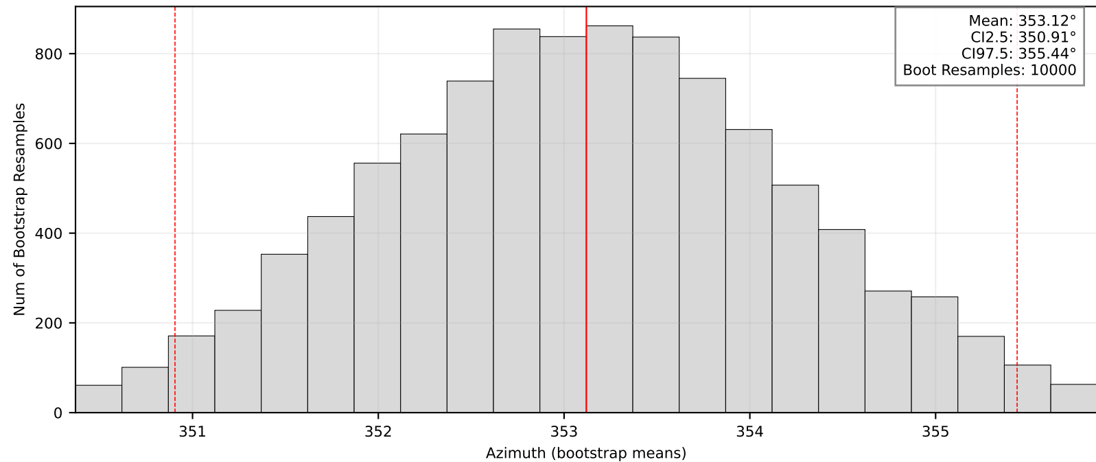
Bootstrap Means/95% CI: BK.BIGV
