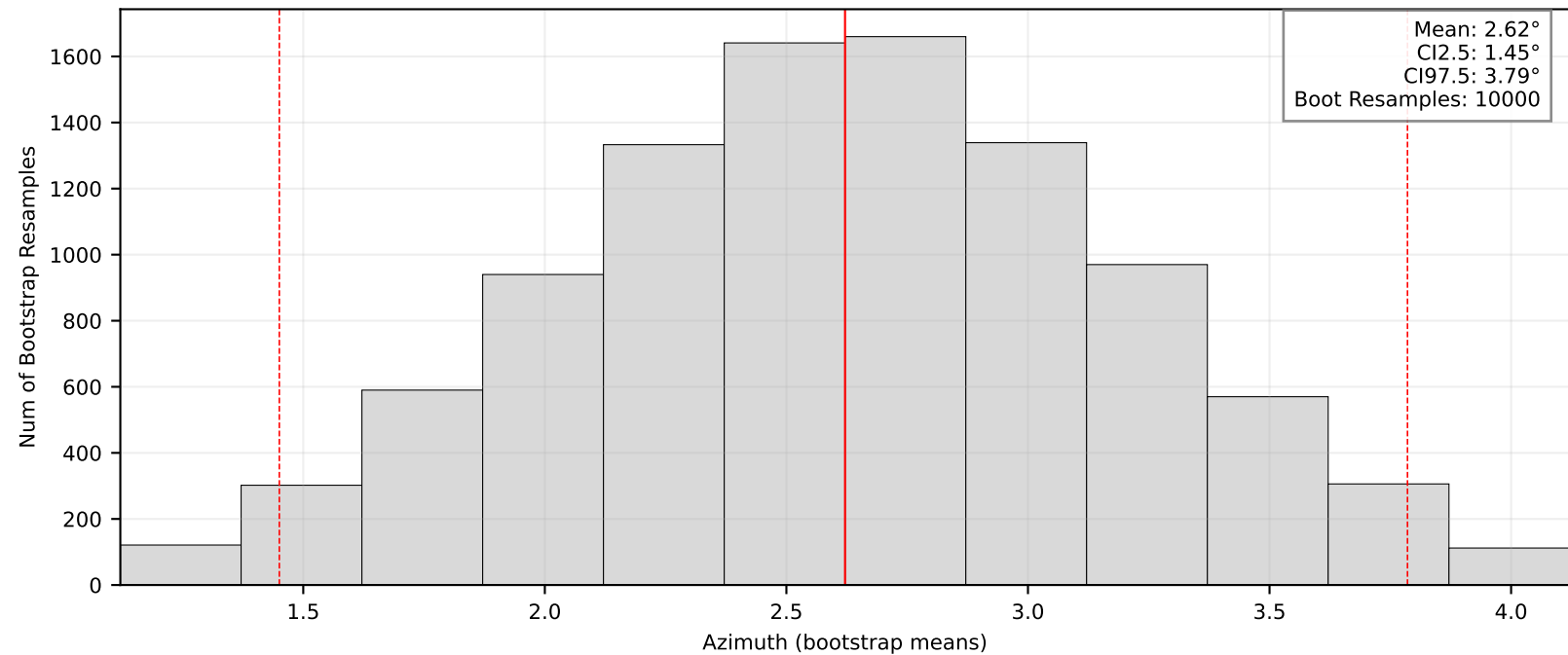
Bootstrap Means/95% CI: BK.AONC
