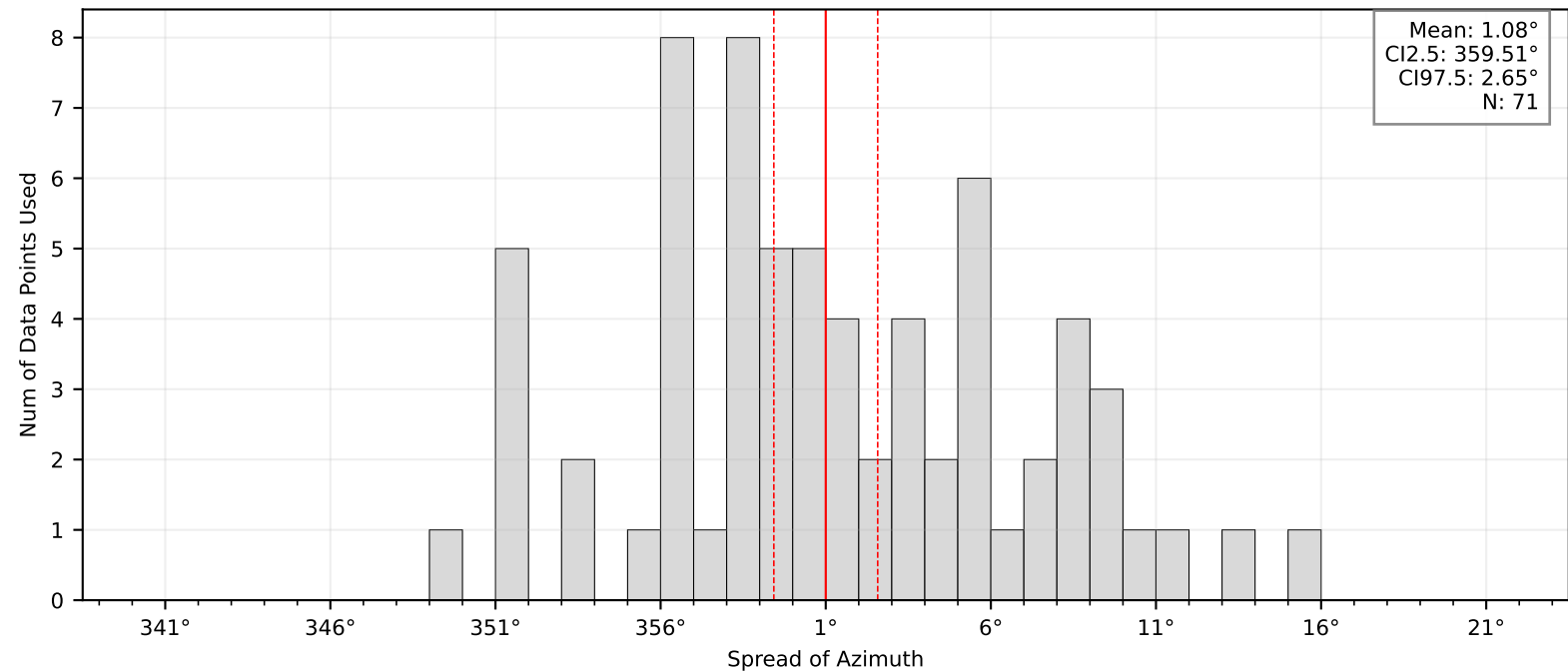
Bootstrap Mean and Confidence Intervals: BK,JCC
