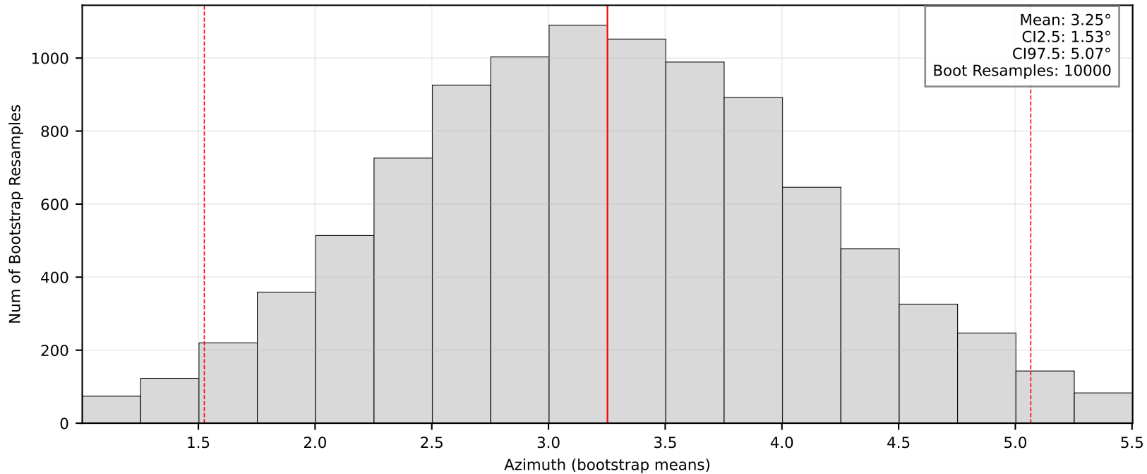
Bootstrap Means/95% CI: BK.MBARI
