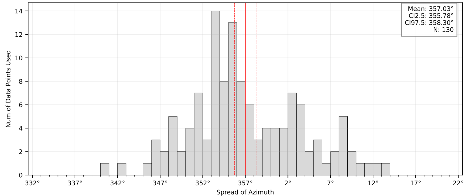
Bootstrap Mean and Confidence Intervals: BK.WLKR
