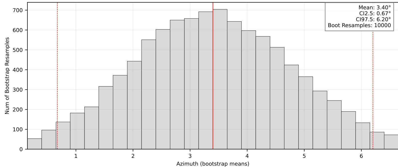
Bootstrap Means/95% CI: BK.BLUE
