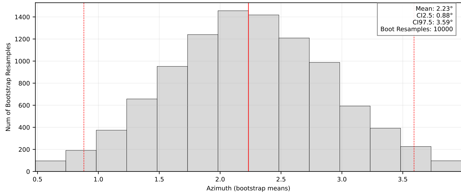
Bootstrap Means/95% CI: BK.ATP
