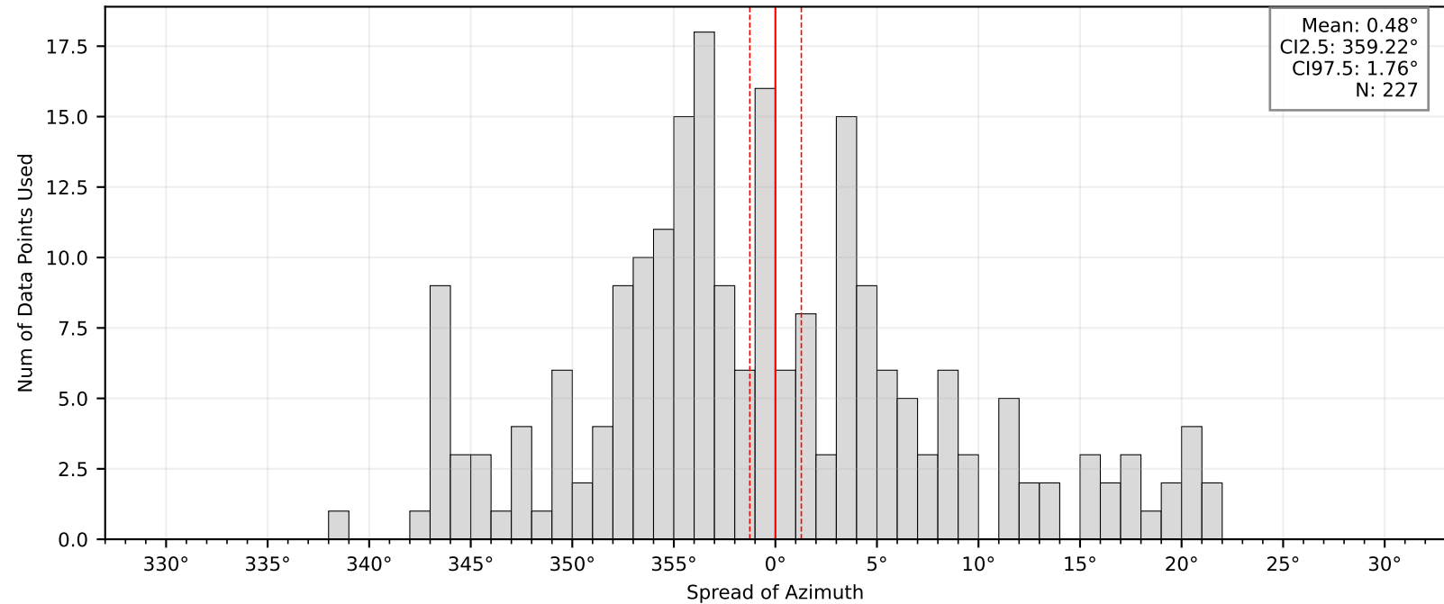
Bootstrap Mean and Confidence Intervals: BK.HATC
