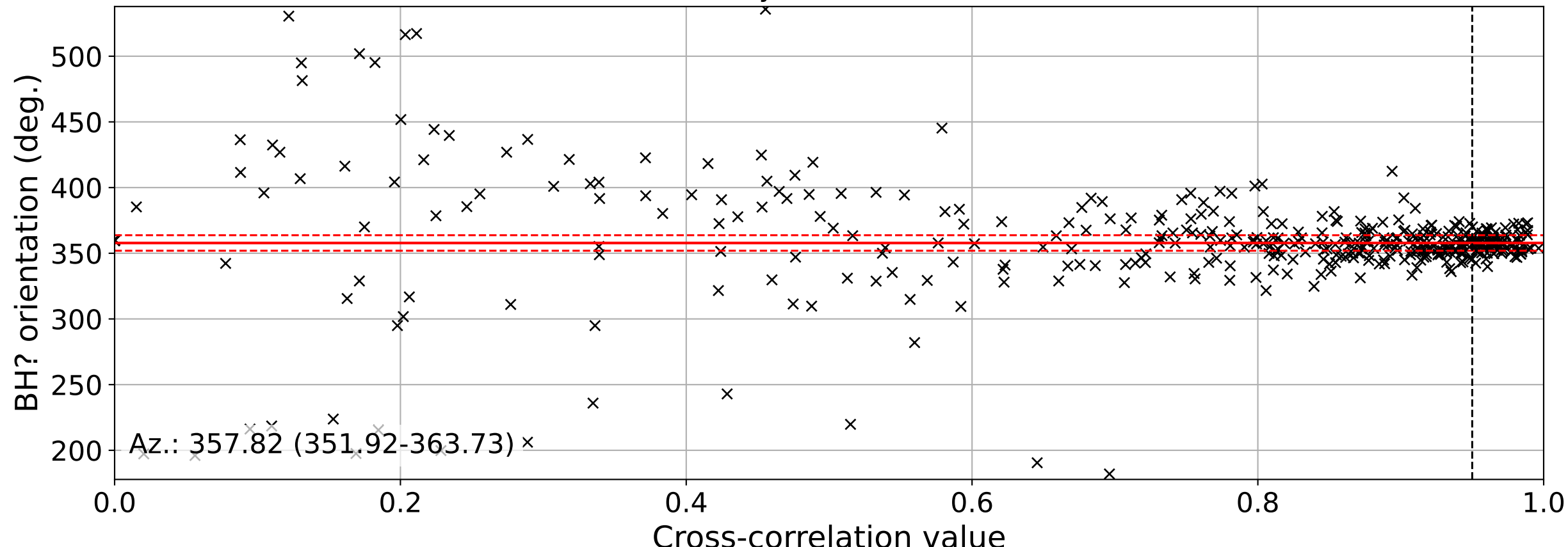
DLOPy result BK.SAO
