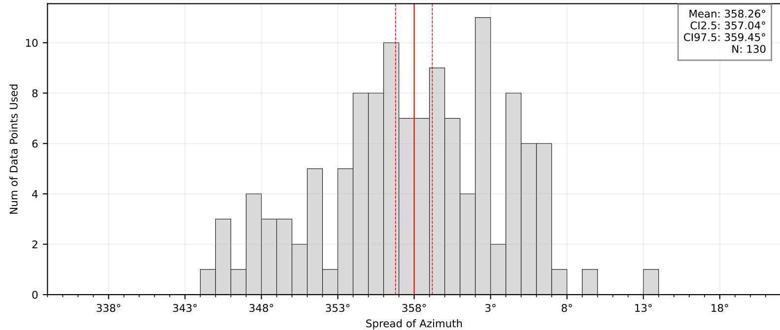
Bootstrap Mean and Confidence Intervals: BK.KETL
