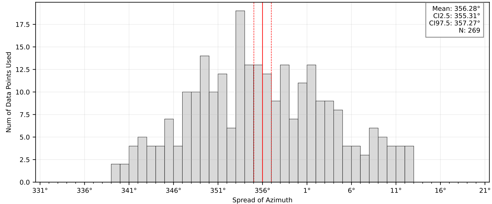
Bootstrap Mean and Confidence Intervals: BK.SAO
