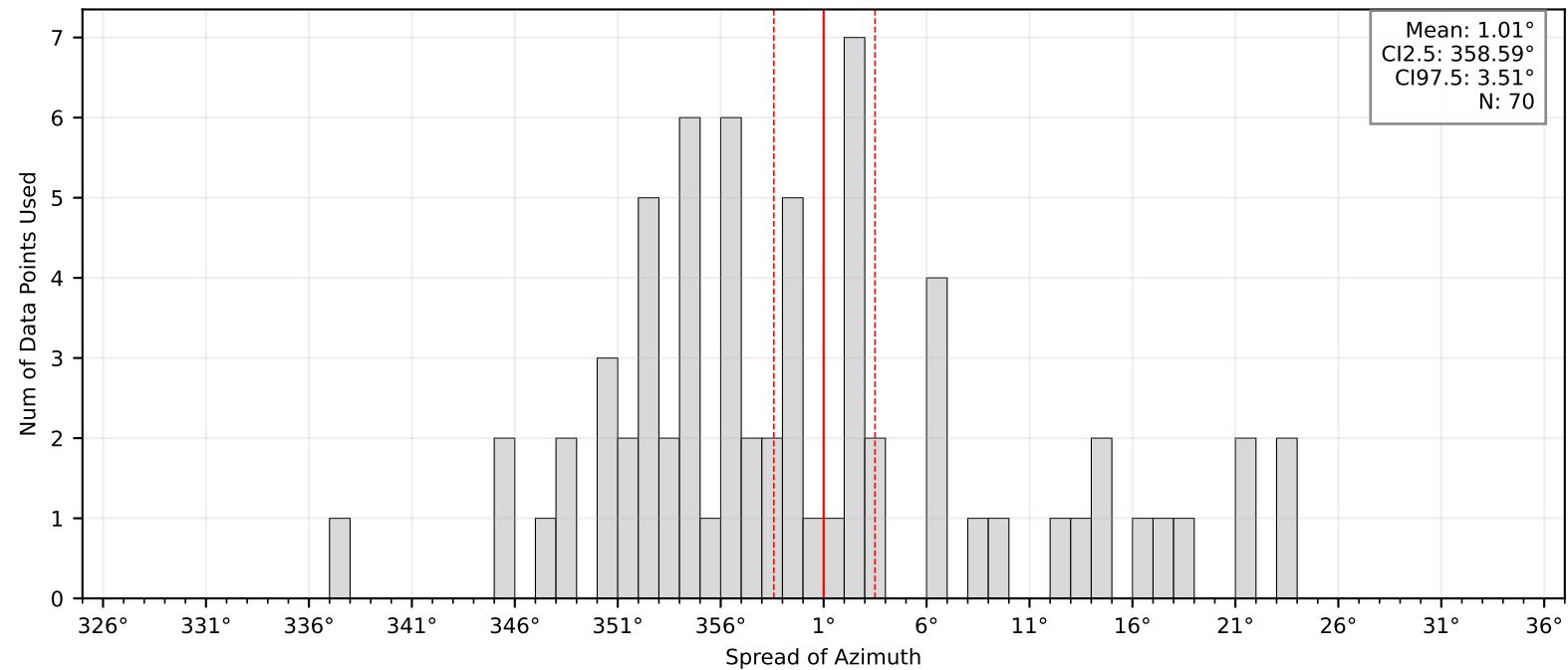
Bootstrap Mean and Confidence Intervals: BK.DIAZ
