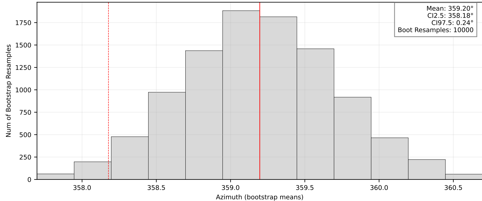
Bootstrap Means/95% CI: BK.UMUN
