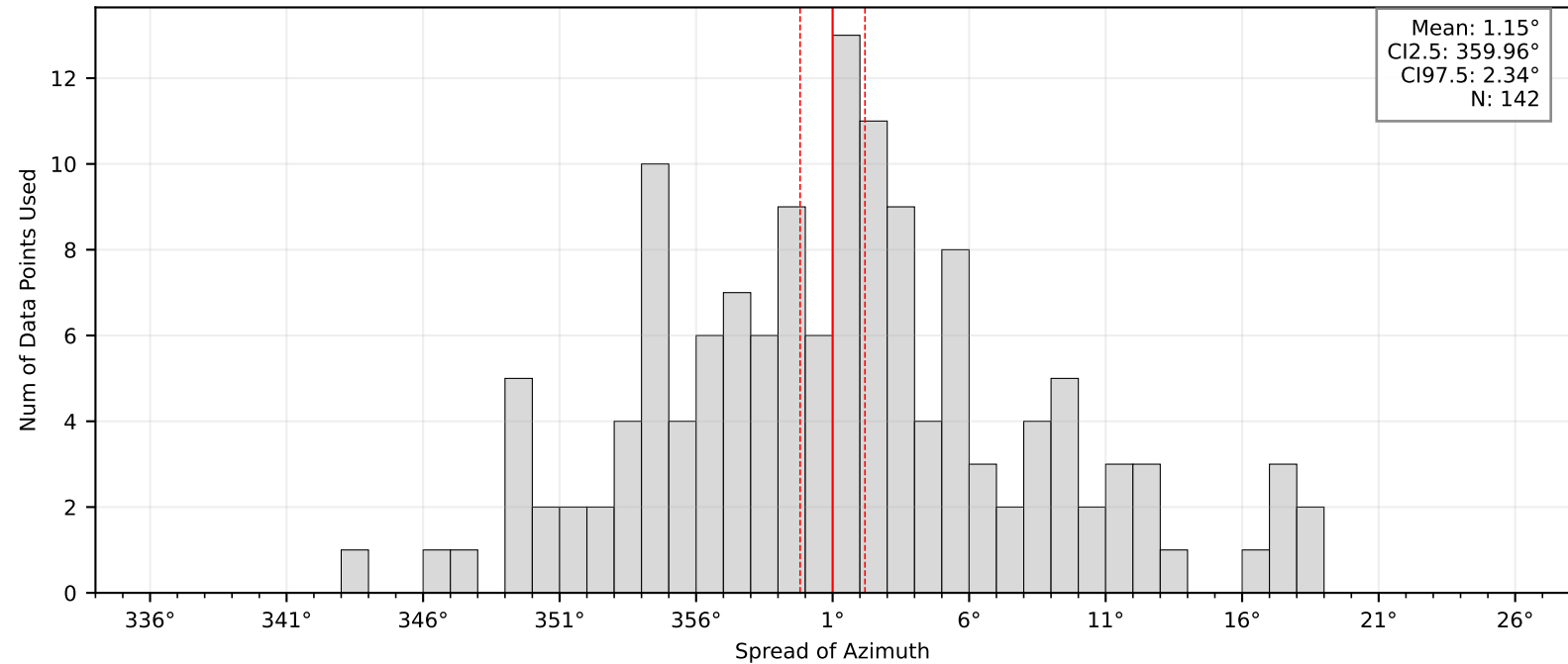
Bootstrap Mean and Confidence Intervals: BK.SPRL
