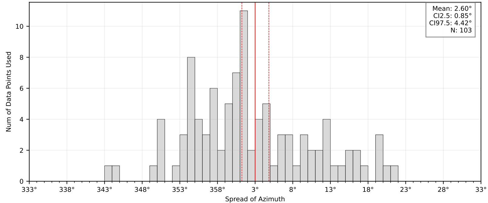
Bootstrap Mean and Confidence Intervals: BK.CCOR
