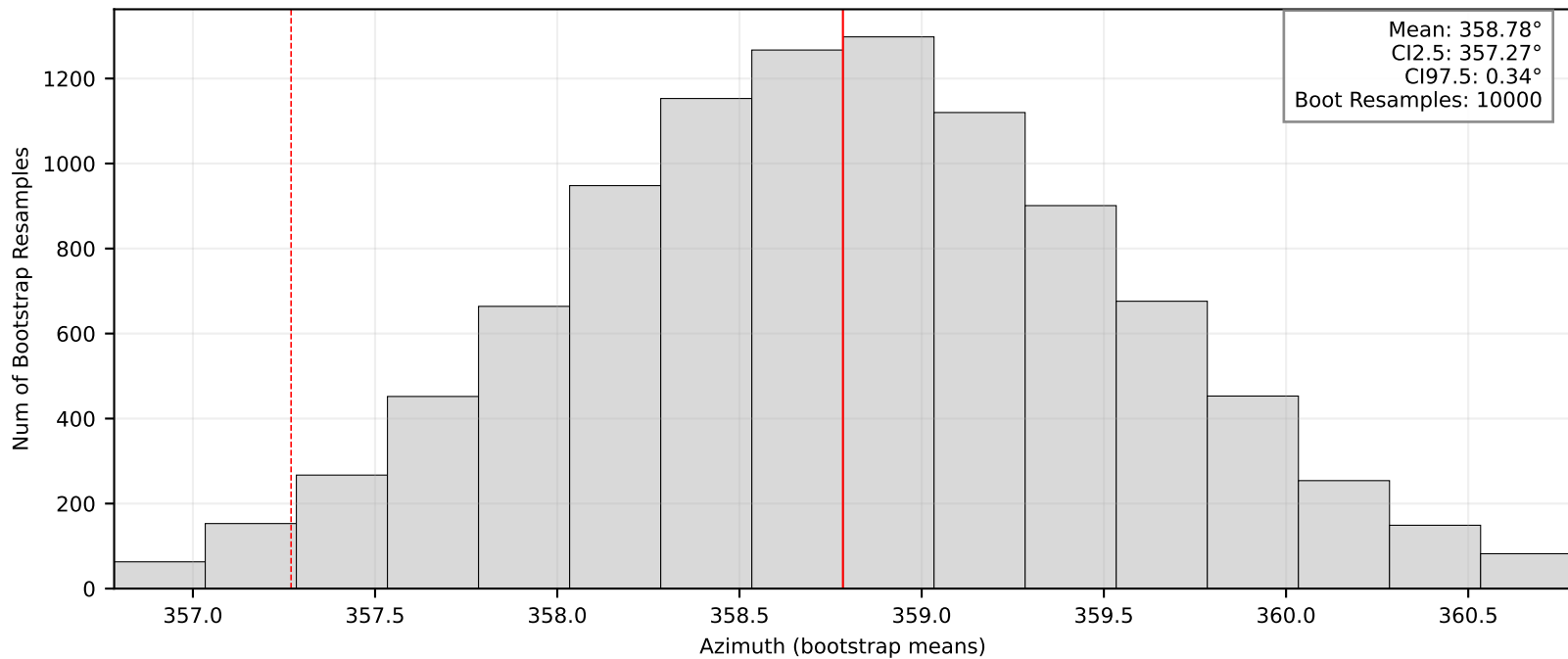
Bootstrap Means/95% CI: BK.GASB
