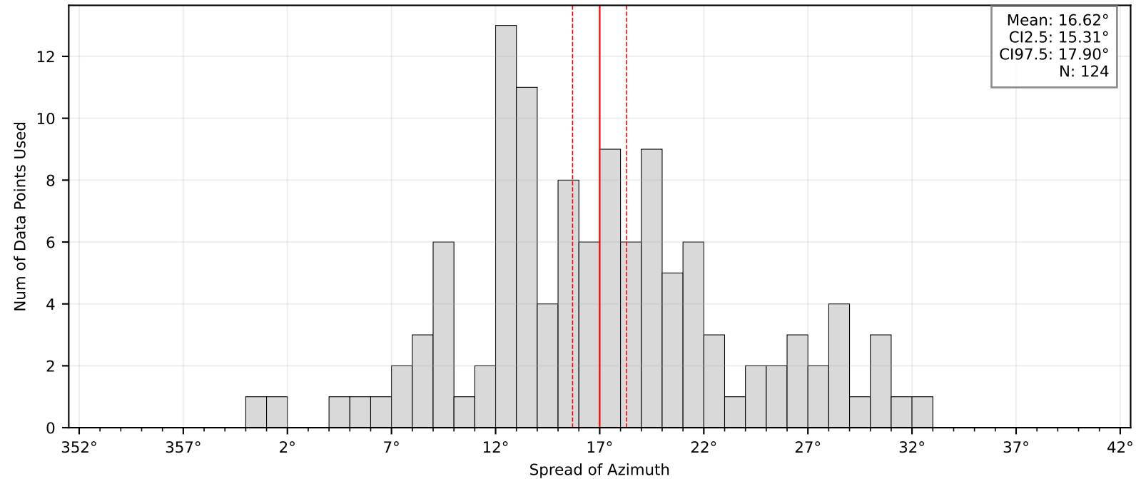
Bootstrap Mean and Confidence Intervals: BK.YUBA
