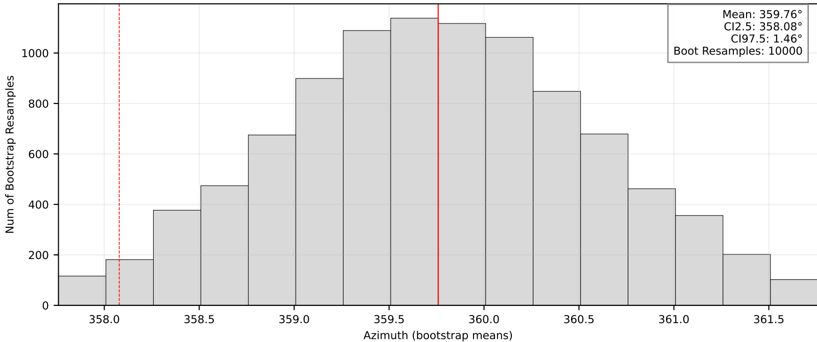
Bootstrap Means/95% CI: BK.LSIB
