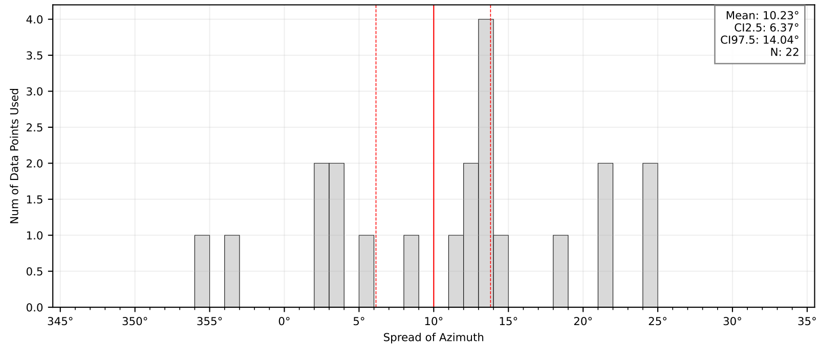
Bootstrap Mean and Confidence Intervals: BK.MORK
