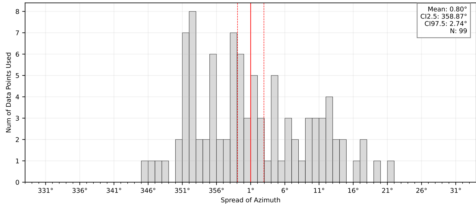
Bootstrap Mean and Confidence Intervals: BK.ALVW
