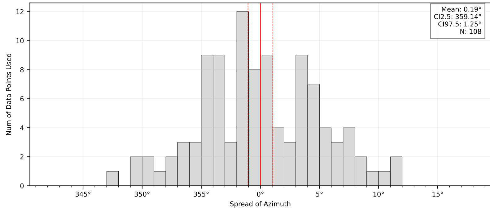
Bootstrap Mean and Confidence Intervals: BK.WEBR
