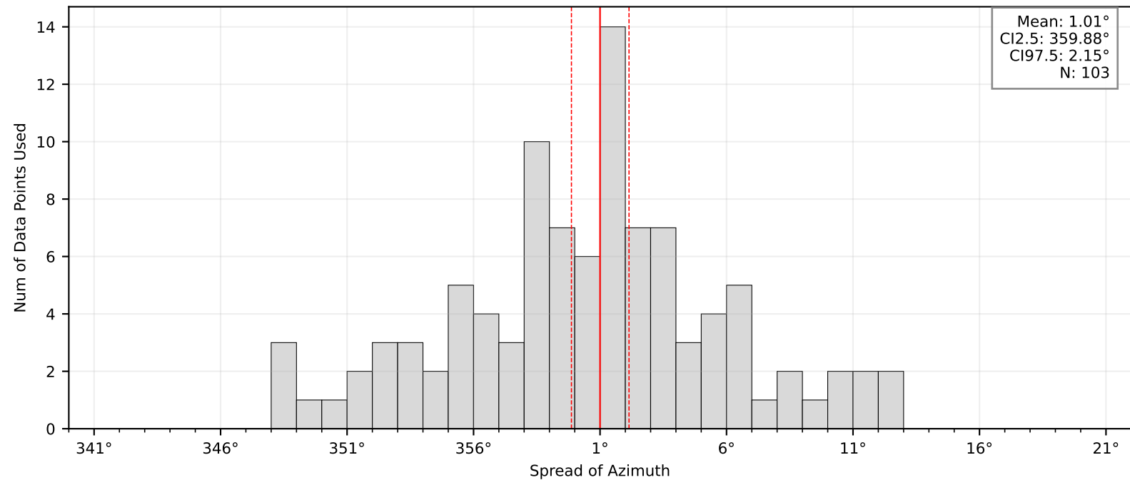
Bootstrap Mean and Confidence Intervals: BK.BLCR
