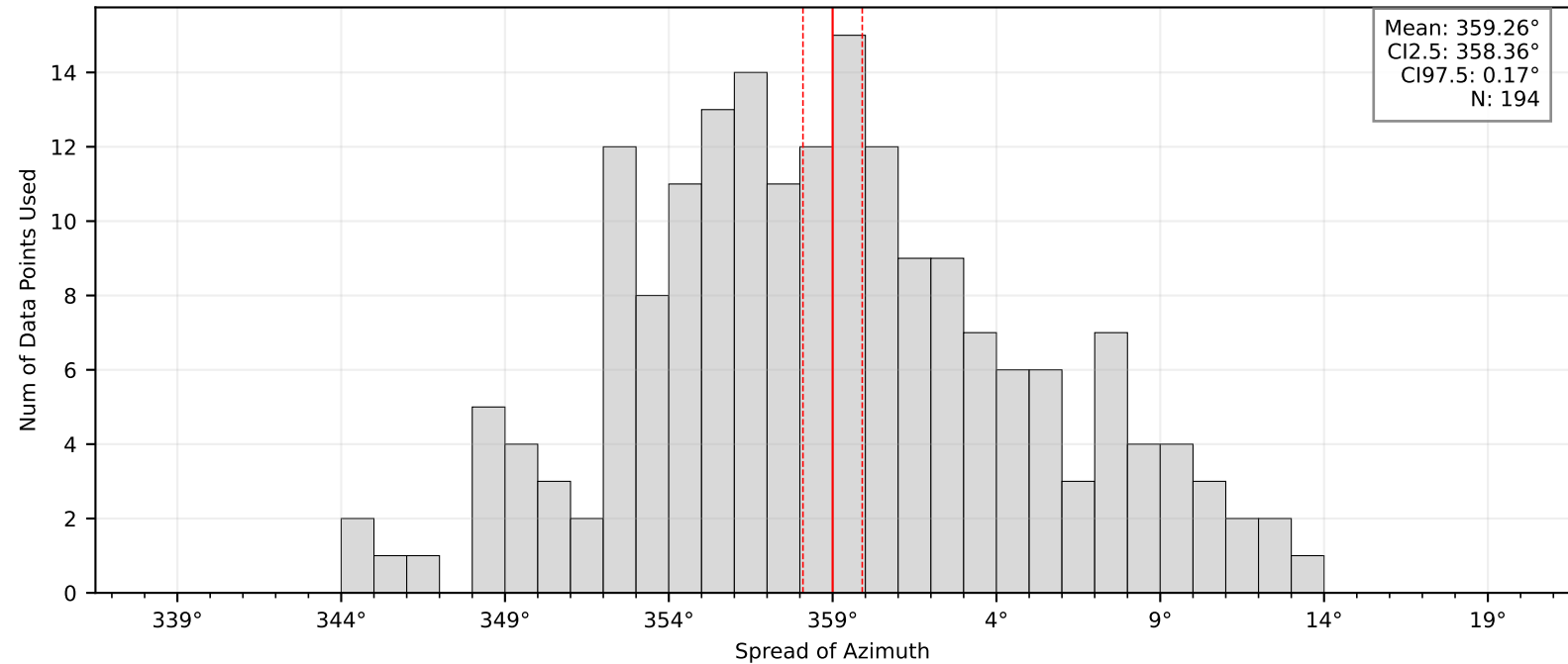
Bootstrap Mean and Confidence Intervals: BK.MHC
