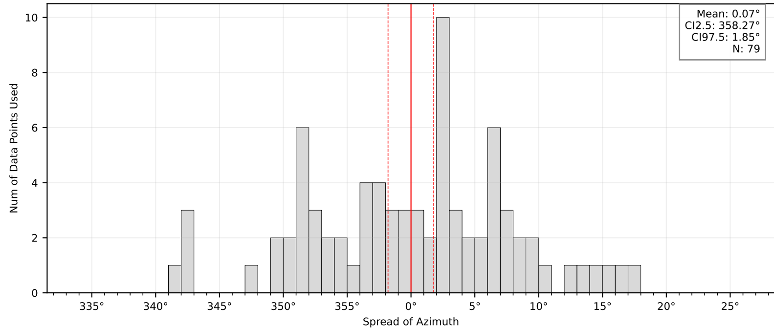
Bootstrap Mean and Confidence Intervals: BK.MOGU
