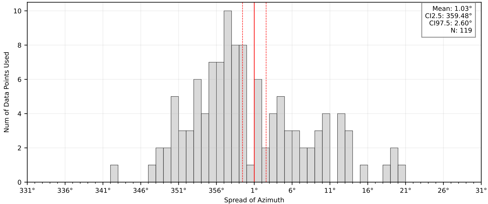
Bootstrap Mean and Confidence Intervals: BK.PORC
