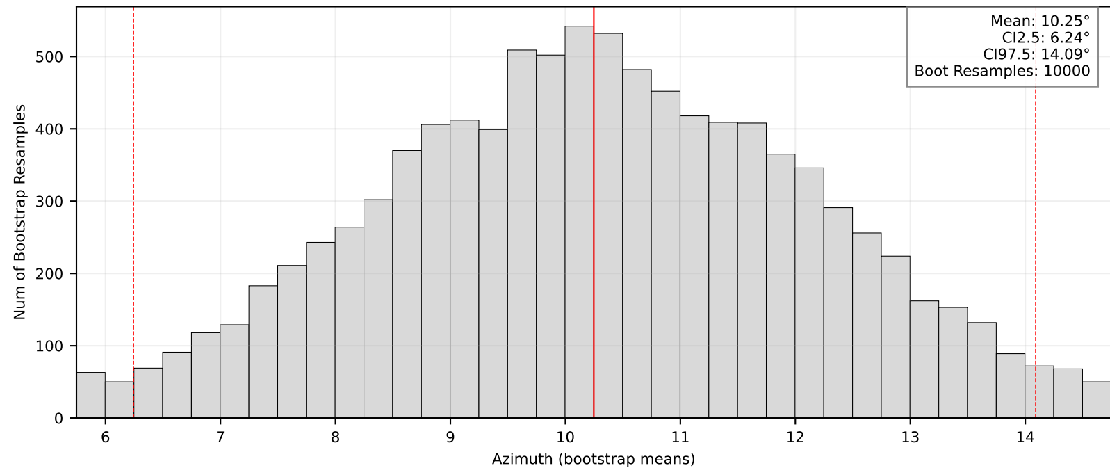
Bootstrap Means/95% CI: BK.MORK
