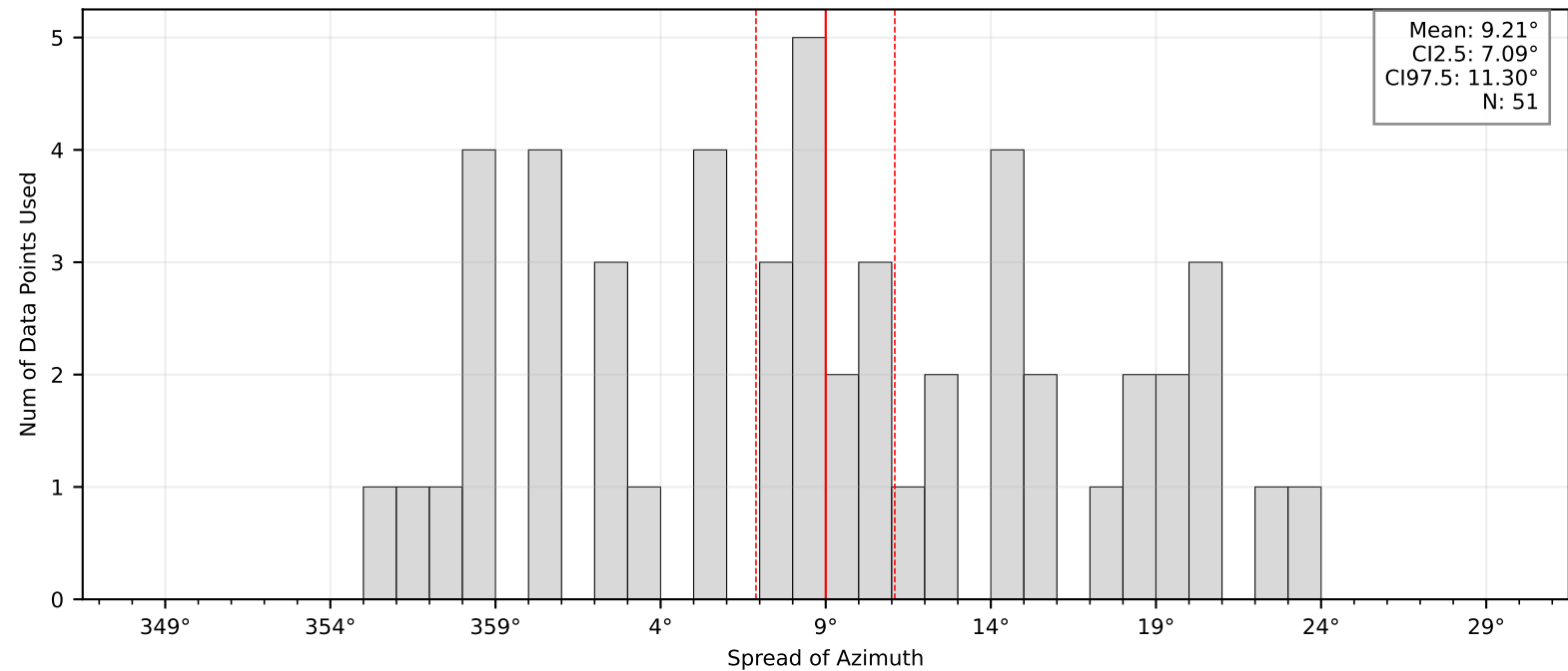
Bootstrap Mean and Confidence Intervals: BK.MBARI
