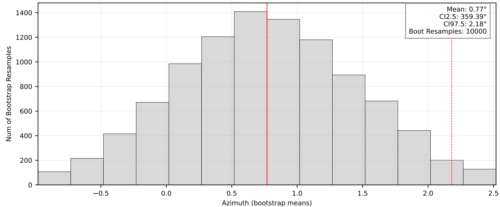
Bootstrap Means/95% CI: BK.AASB
