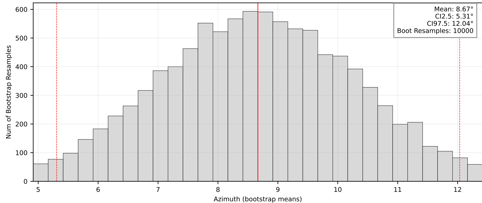
Bootstrap Means/95% CI: BK.SCZ
