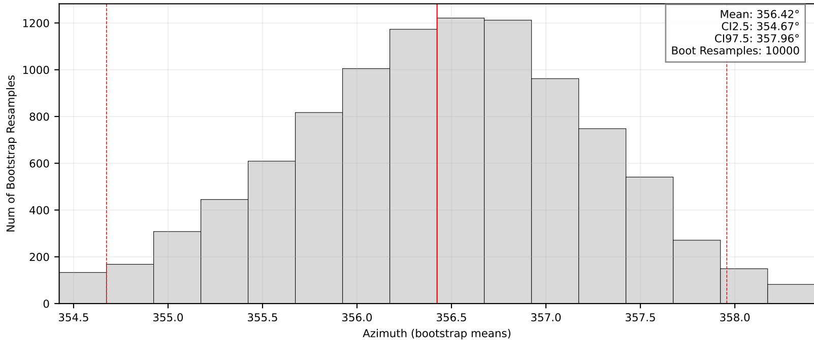
Bootstrap Means/95% CI: BK.JEWT
