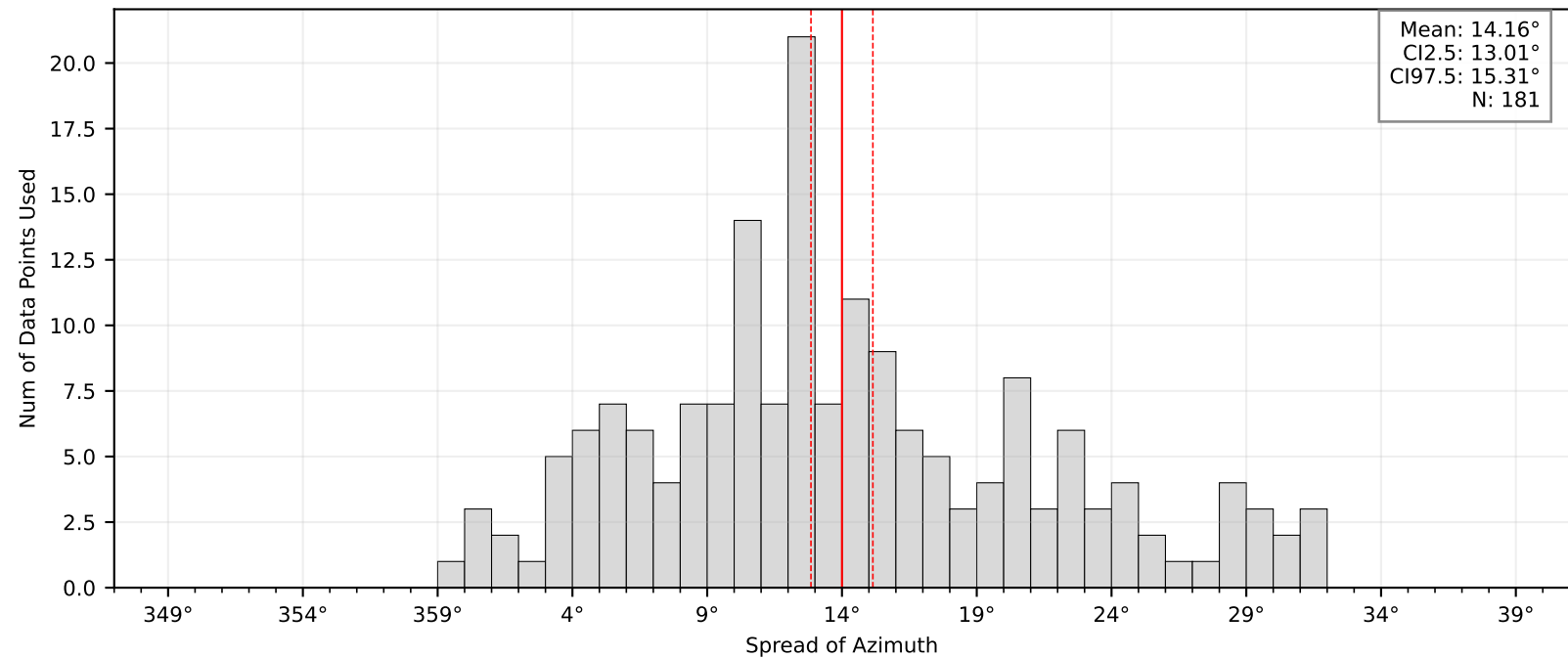
Bootstrap Mean and Confidence Intervals: BK.BRAD
