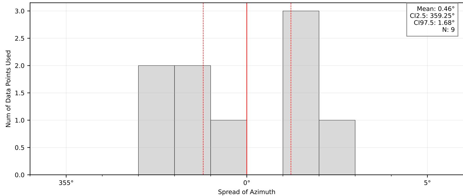
Bootstrap Mean and Confidence Intervals: BK.SPAN
