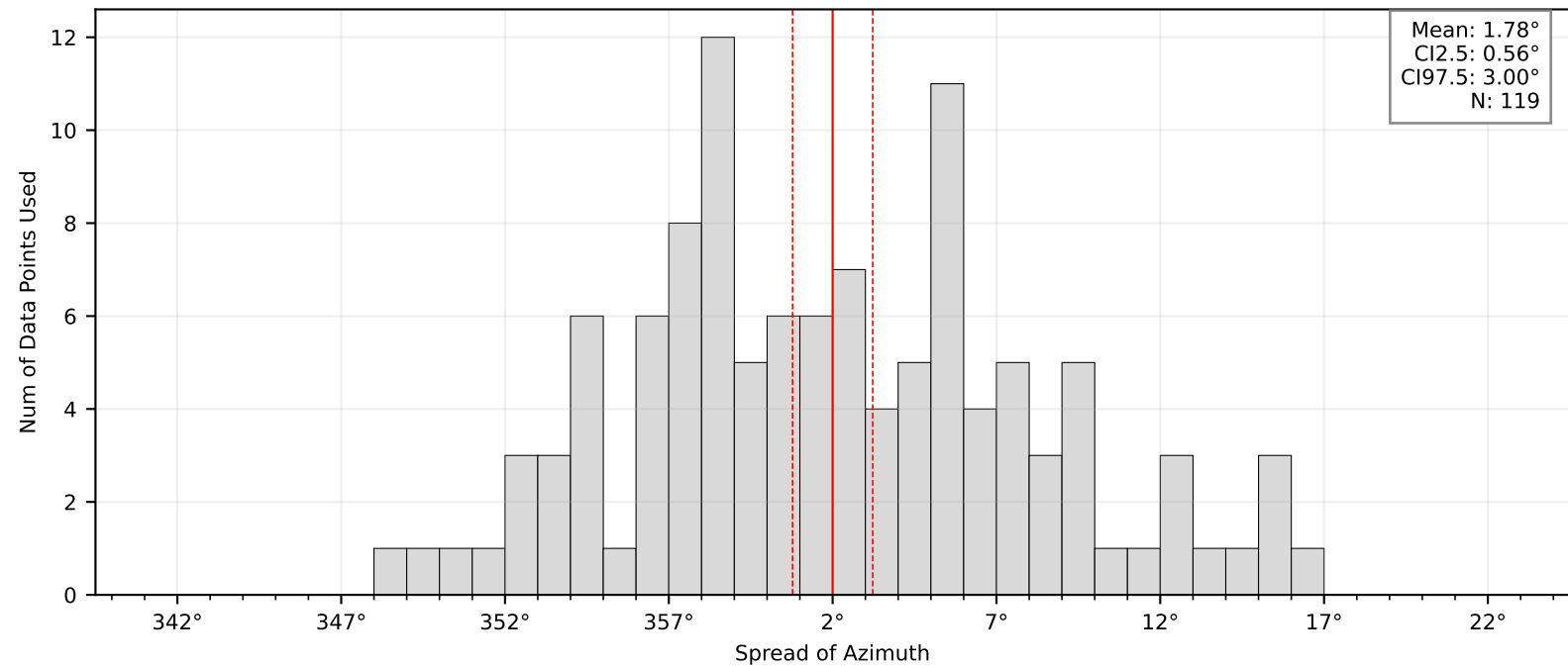
Bootstrap Mean and Confidence Intervals: BK.ROMB
