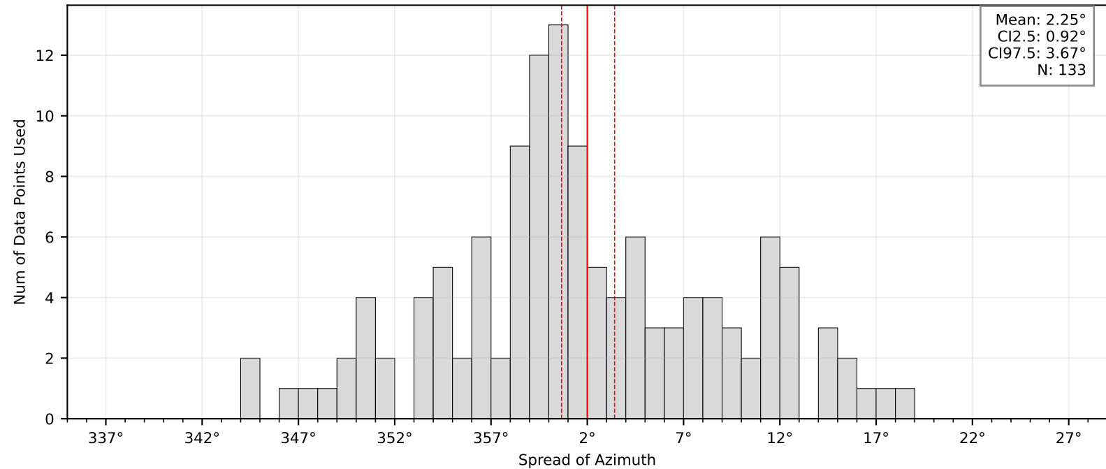
Bootstrap Mean and Confidence Intervals: BK.PETL
