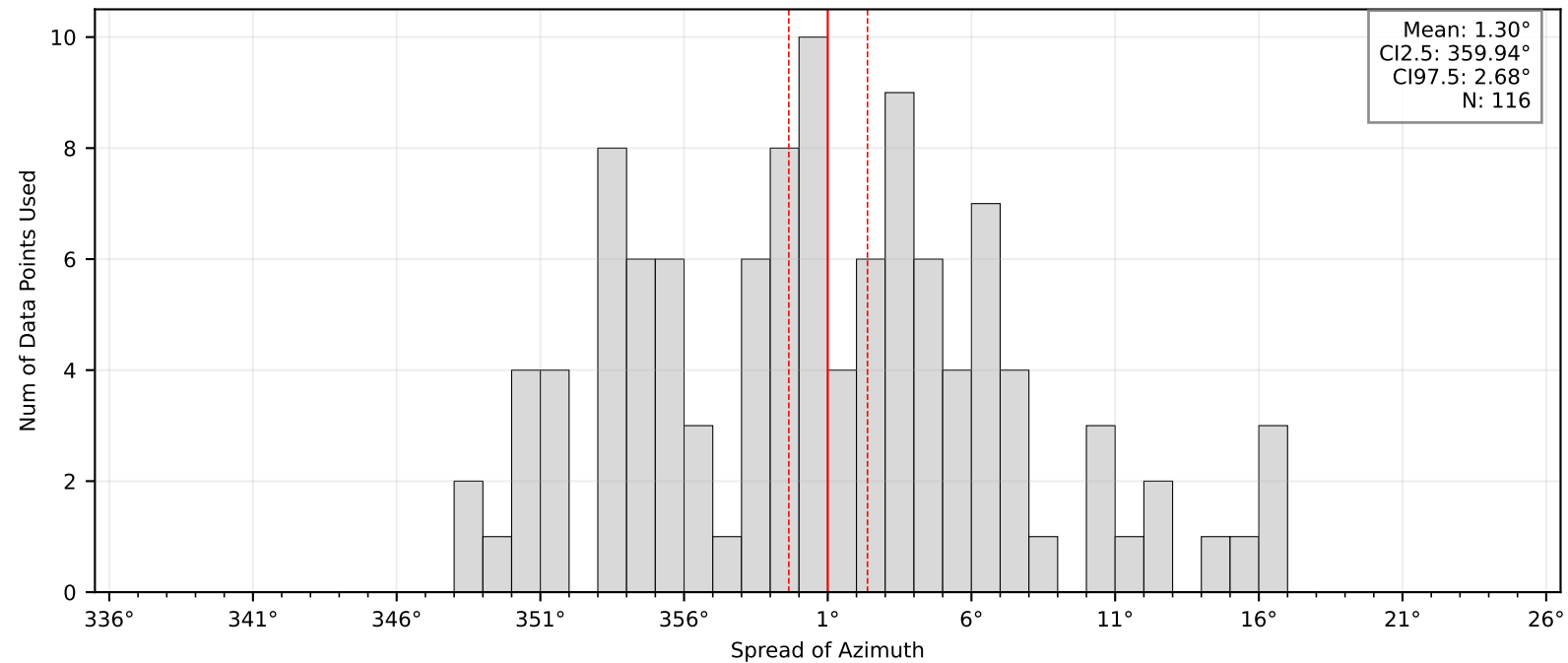
Bootstrap Mean and Confidence Intervals: BK.LGMB
