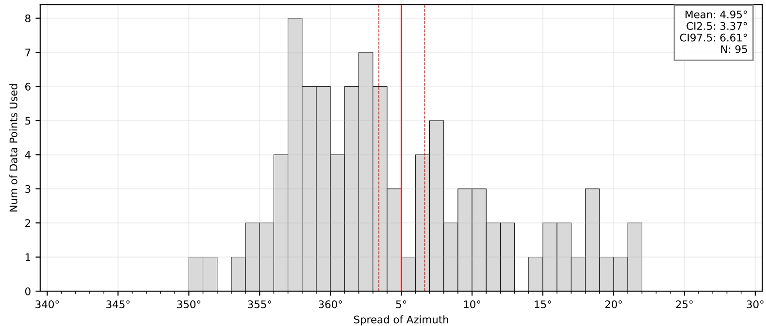
Bootstrap Mean and Confidence Intervals: BK.LCUV
