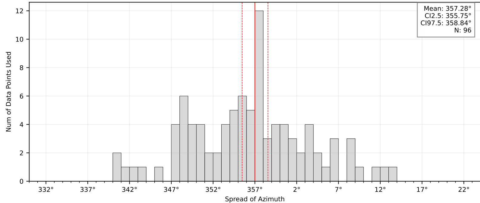
Bootstrap Mean and Confidence Intervals: BK.HAYF
