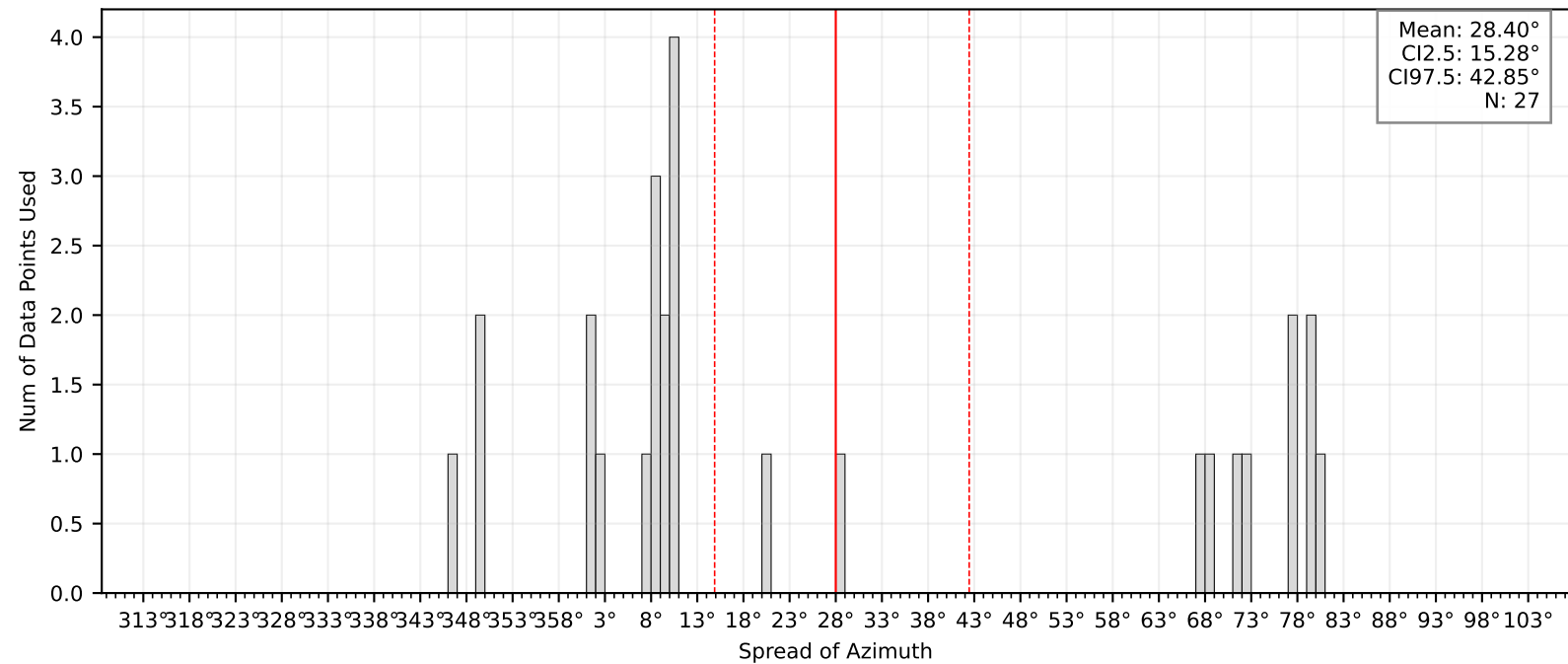
Bootstrap Mean and Confidence Intervals: BK.WTWN
