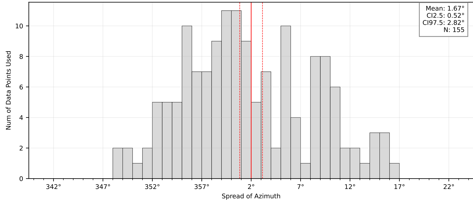
Bootstrap Mean and Confidence Intervals: BK.HULI
