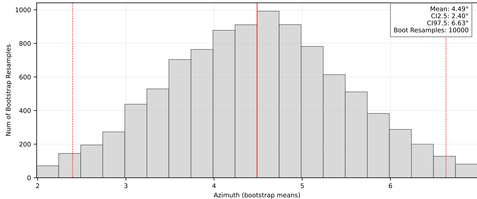
Bootstrap Means/95% CI: BK.DANT
