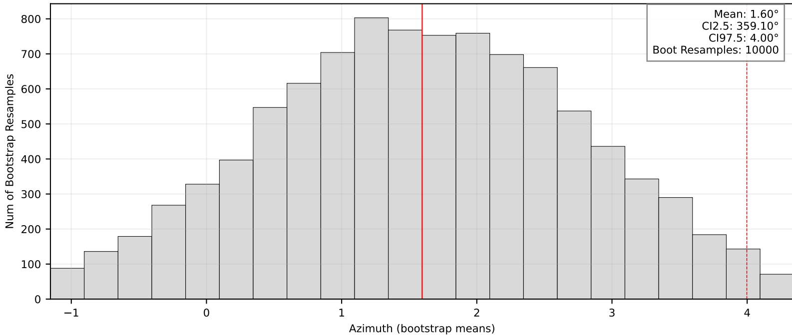
Bootstrap Means/95% CI: BK.BUCR
