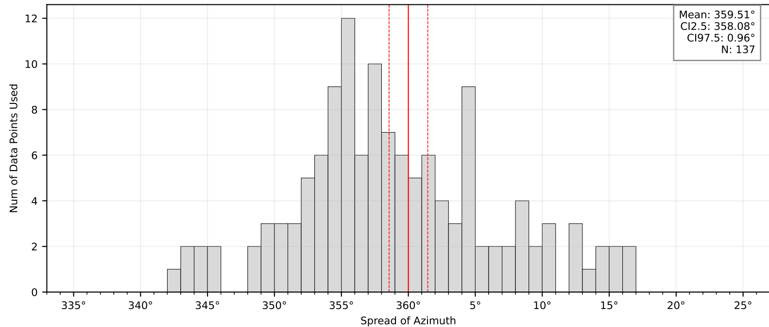
Bootstrap Mean and Confidence Intervals: BK.PORC
