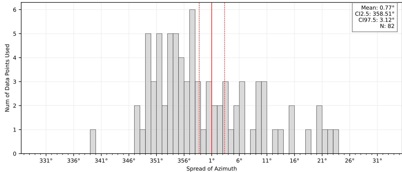
Bootstrap Mean and Confidence Intervals: BK.LITV
