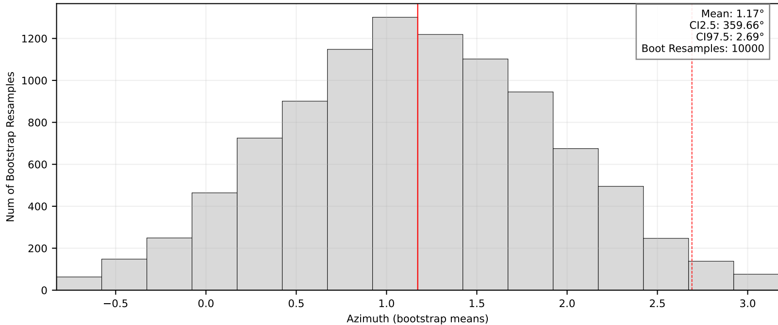
Bootstrap Means/95% CI: BK.SPRL
