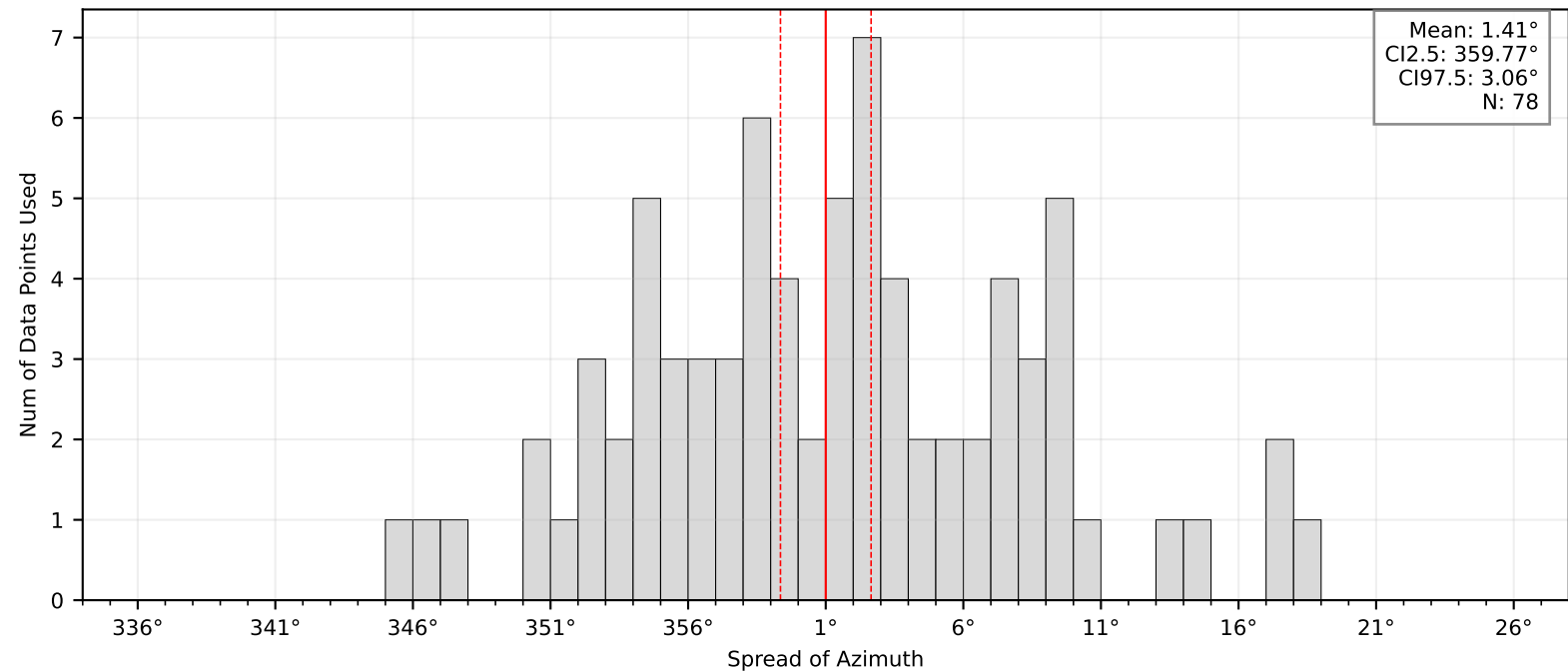
Bootstrap Mean and Confidence Intervals: BK.PWAY
