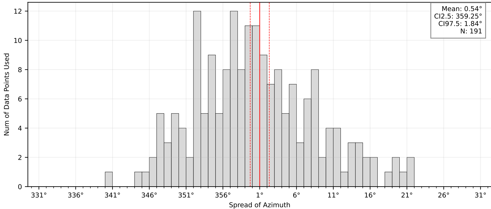
Bootstrap Mean and Confidence Intervals: BK.DLIK
