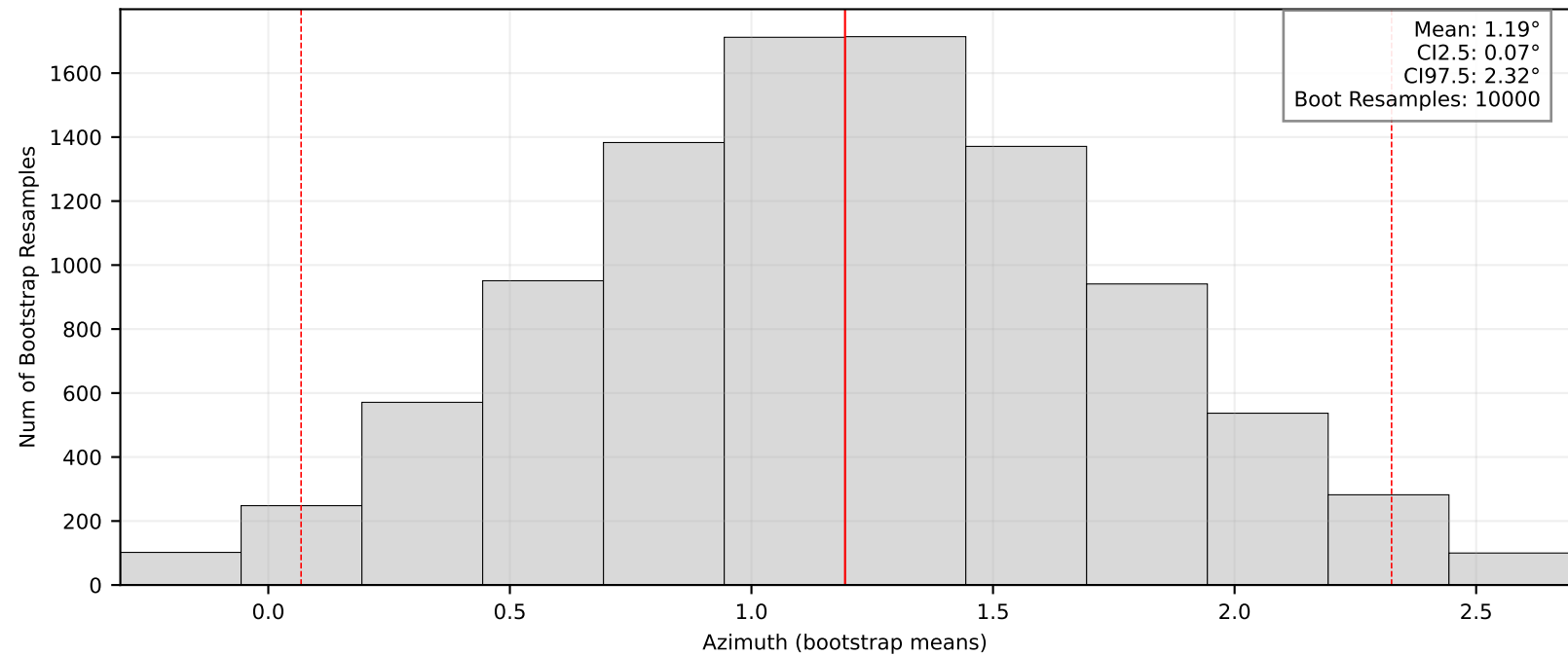
Bootstrap Means/95% CI: BK.SHWD
