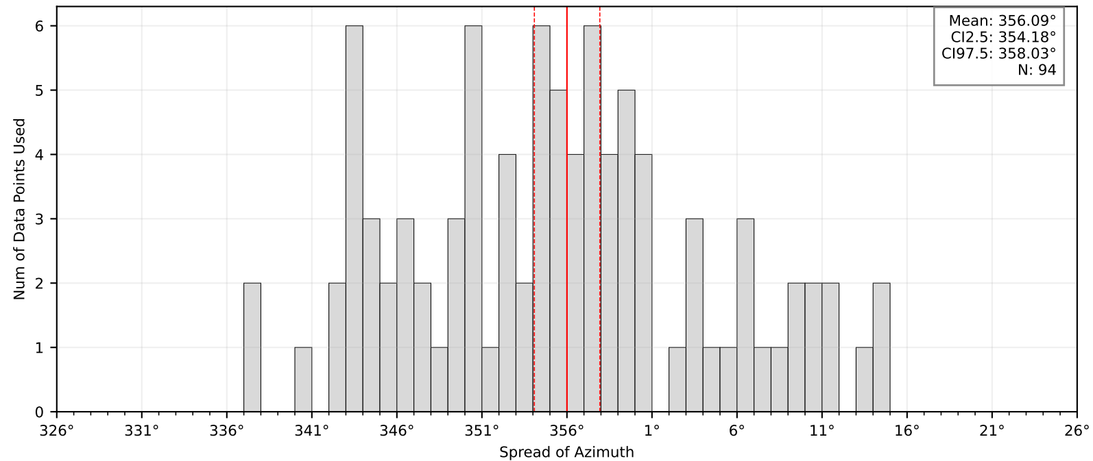
Bootstrap Mean and Confidence Intervals: BK.GHOP
