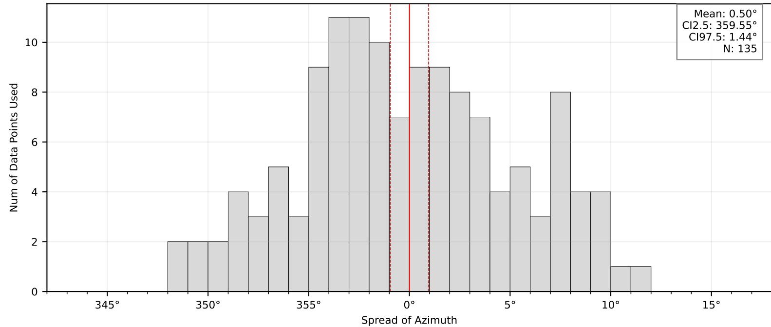
Bootstrap Mean and Confidence Intervals: BK.ORV
