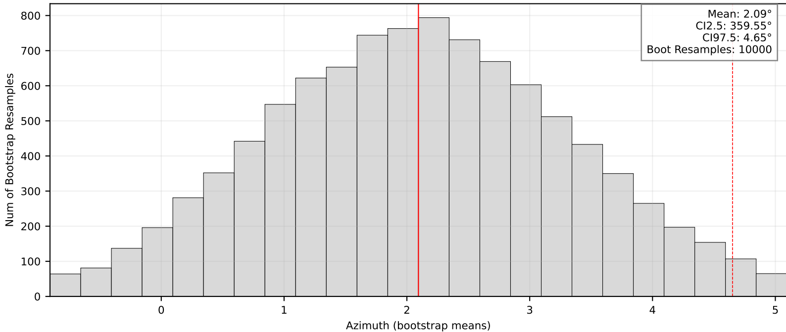
Bootstrap Means/95% CI: BK.HUNT
