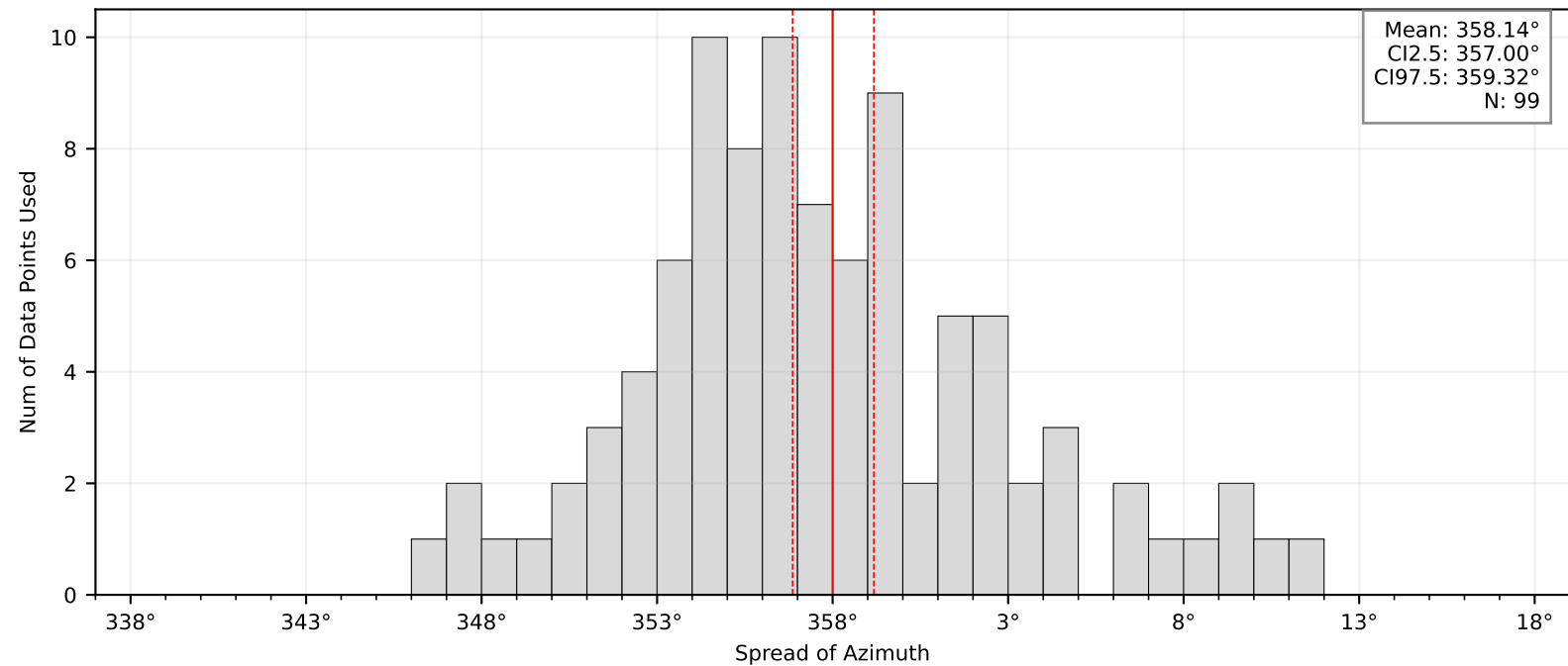
Bootstrap Mean and Confidence Intervals: BK.BRK
