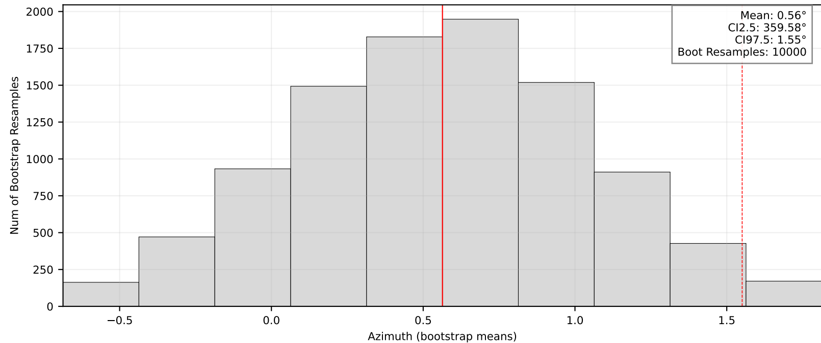
Bootstrap Means/95% CI: BK.CMB
