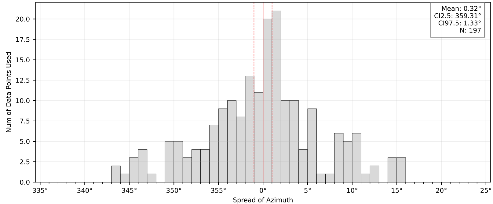
Bootstrap Mean and Confidence Intervals: BK.AASB
