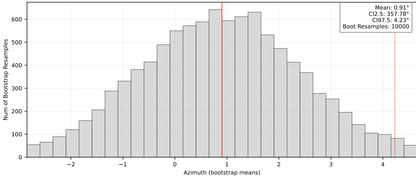
Bootstrap Means/95% CI: BK.TULE
