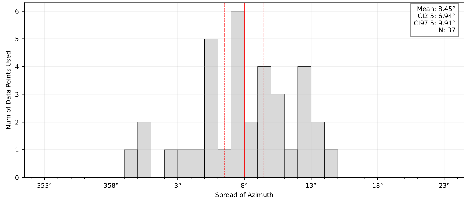
Bootstrap Mean and Confidence Intervals: BK.TWIT
