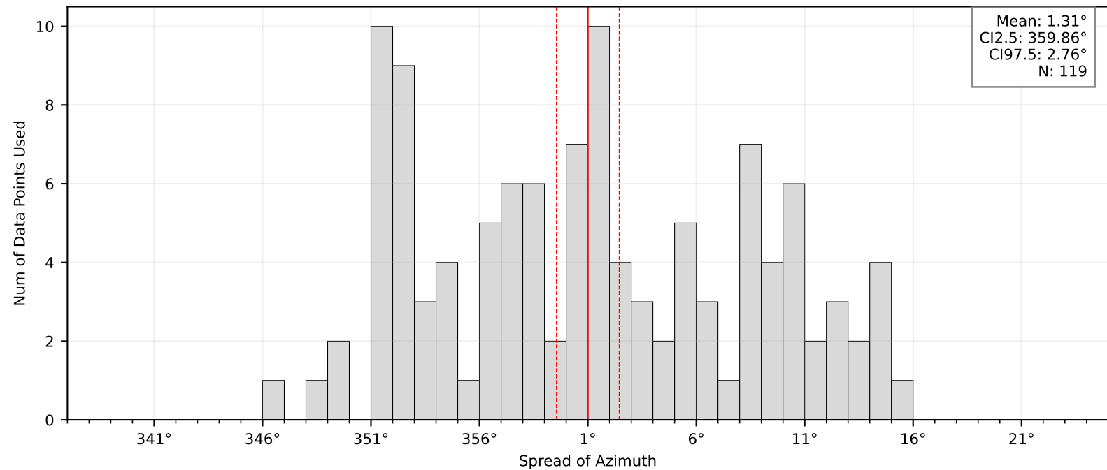
Bootstrap Mean and Confidence Intervals: BK.RUSS
