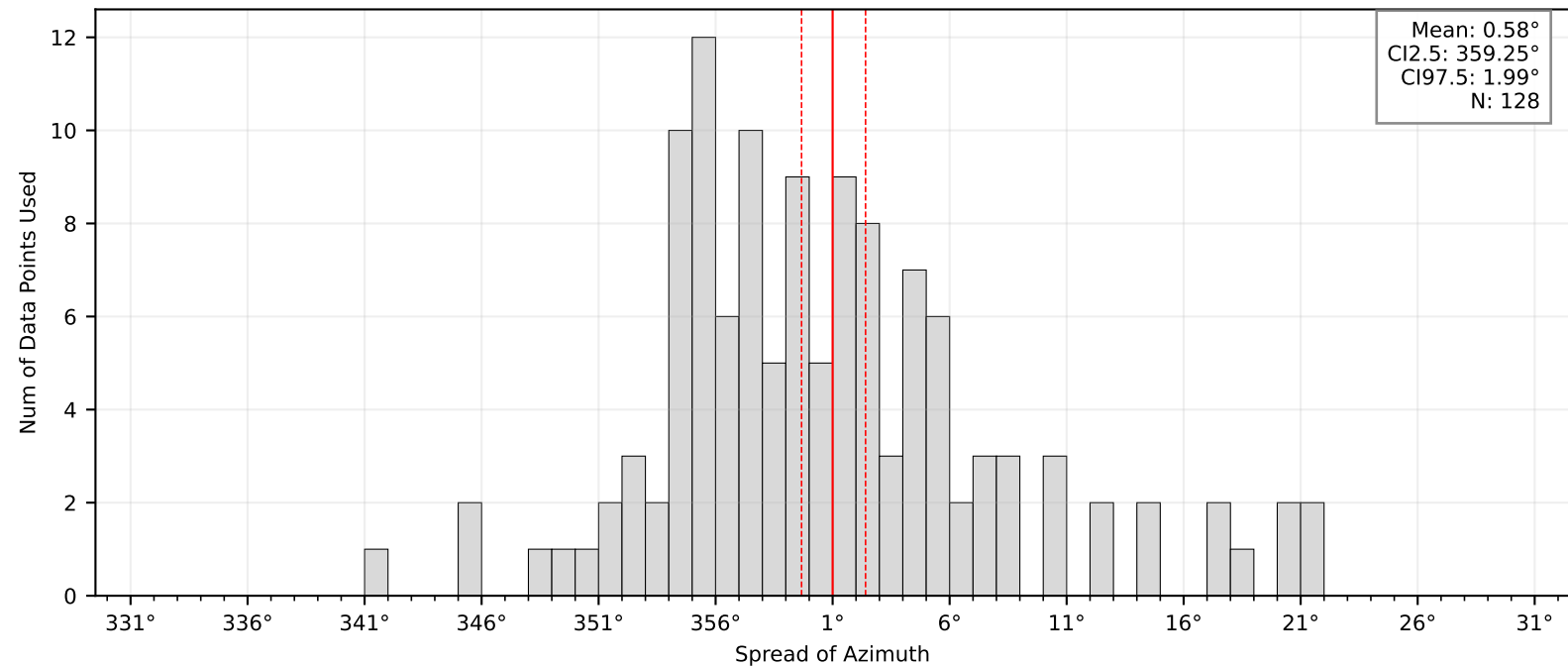
Bootstrap Mean and Confidence Intervals: BK.MZTA
