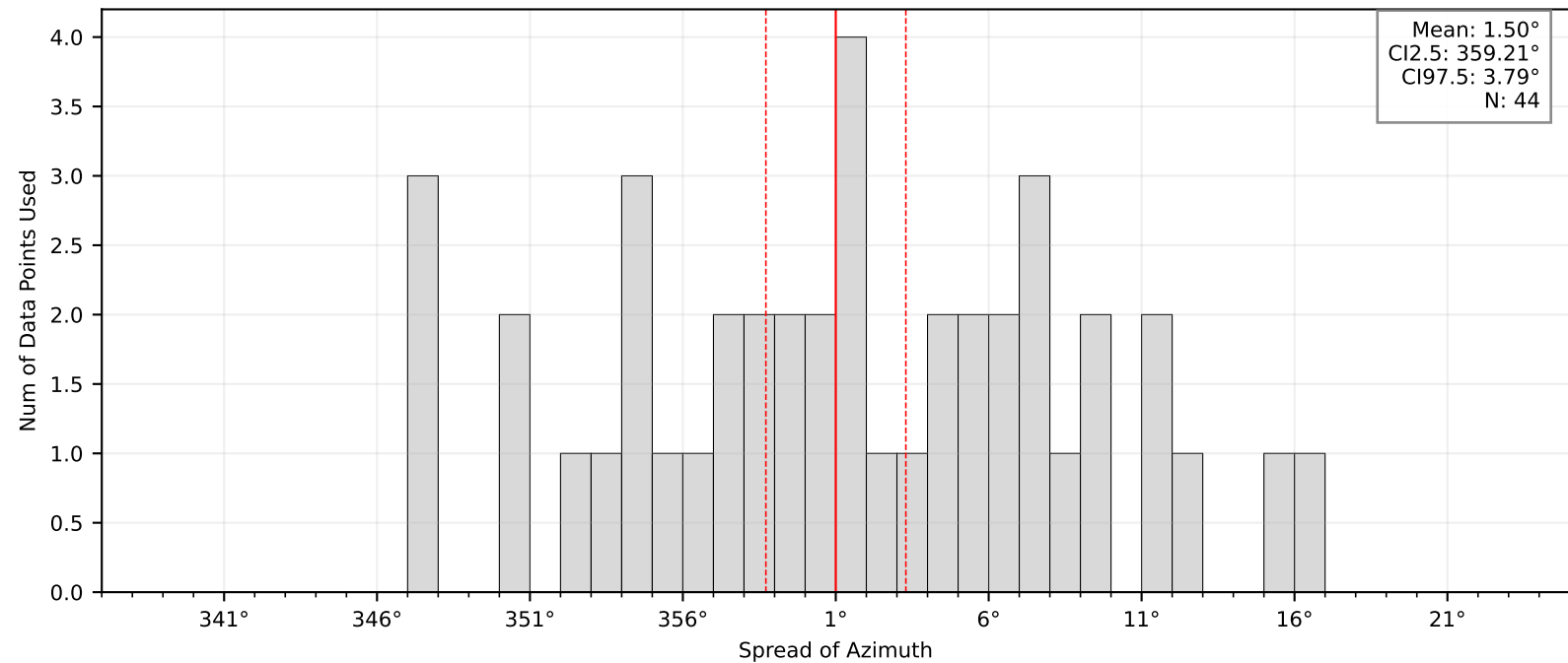
Bootstrap Mean and Confidence Intervals: BK.DMOR
