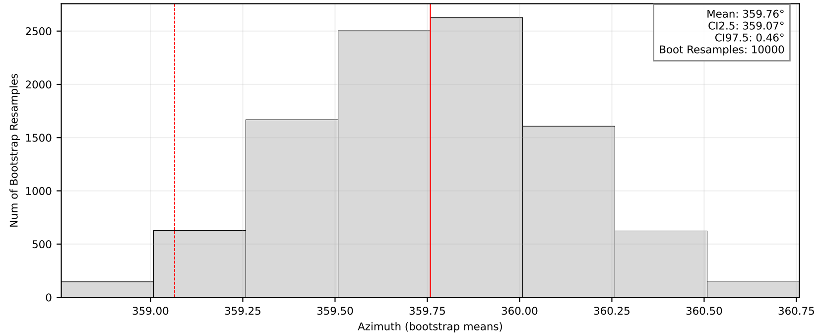
Bootstrap Means/95% CI: BK.MTOS
