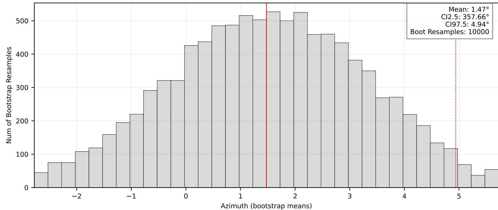
Bootstrap Means/95% CI: BK.BIGM
