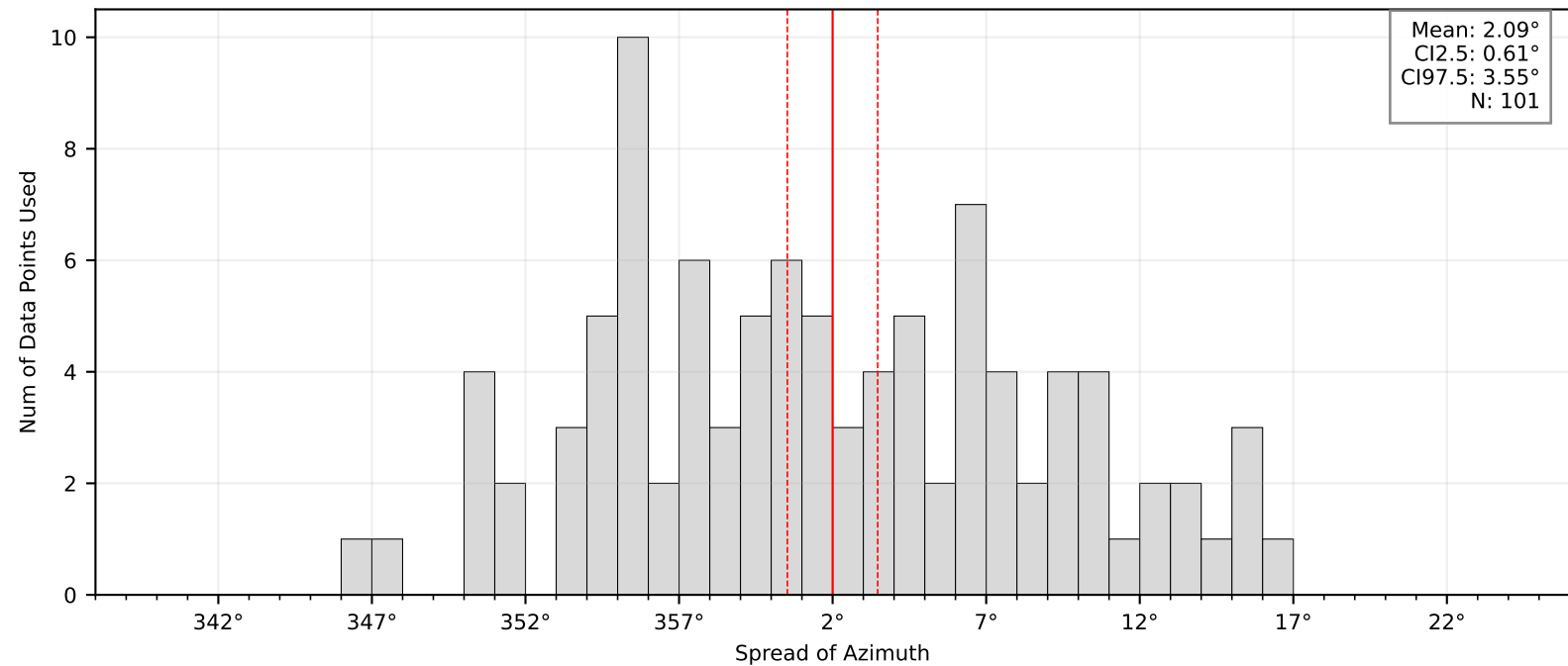
Bootstrap Mean and Confidence Intervals: BK.FORD
