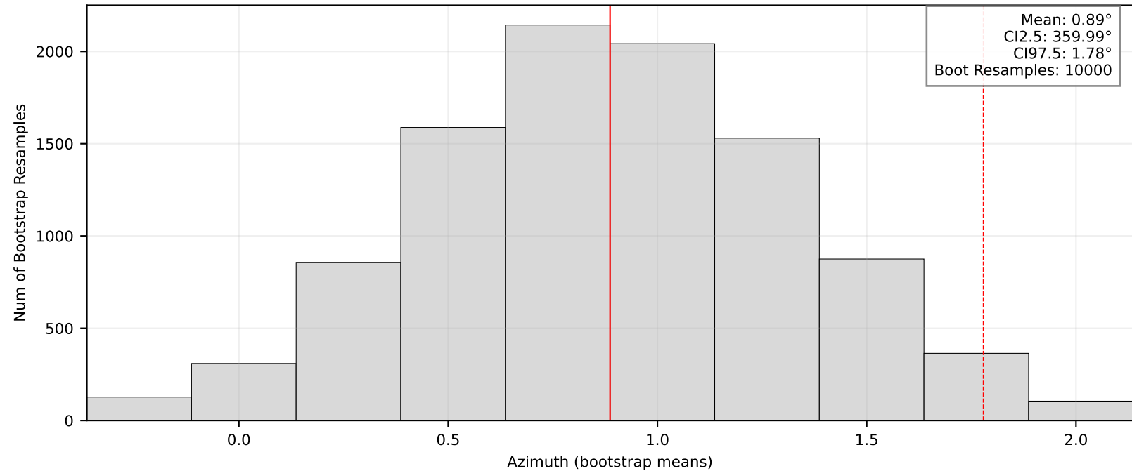
Bootstrap Means/95% CI: BK,JCC
