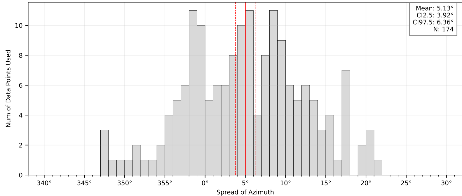
Bootstrap Mean and Confidence Intervals: BK.BRIC
