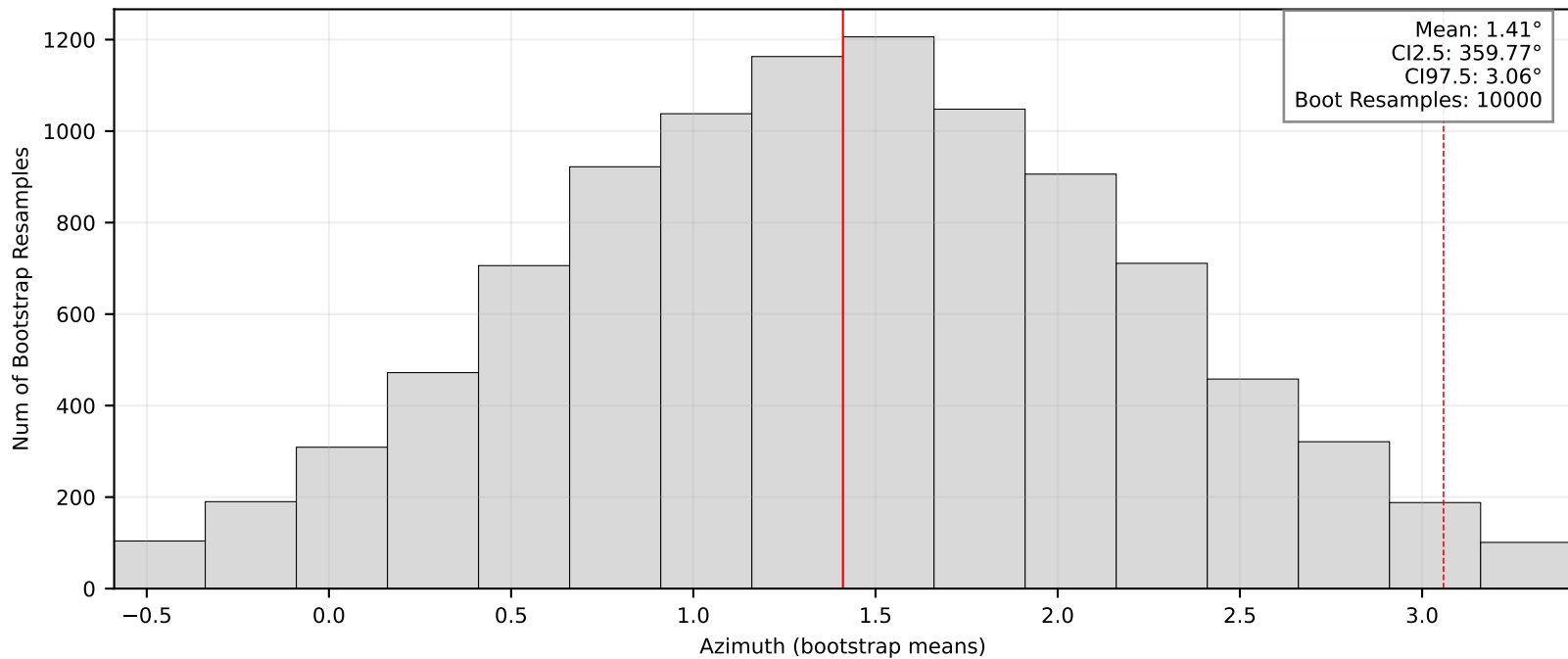
Bootstrap Means/95% CI: BK.PWAY
