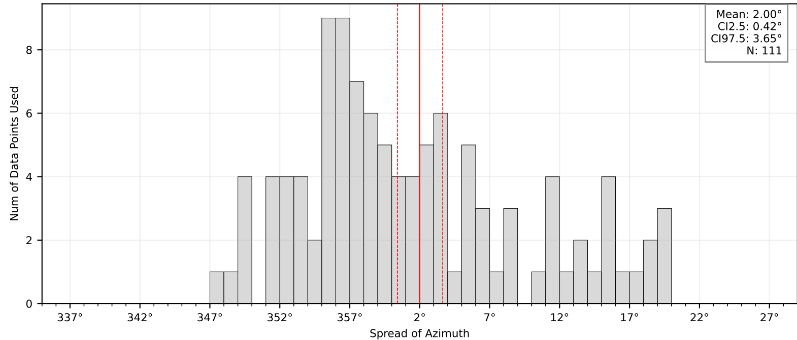
Bootstrap Mean and Confidence Intervals: BK.WROK
