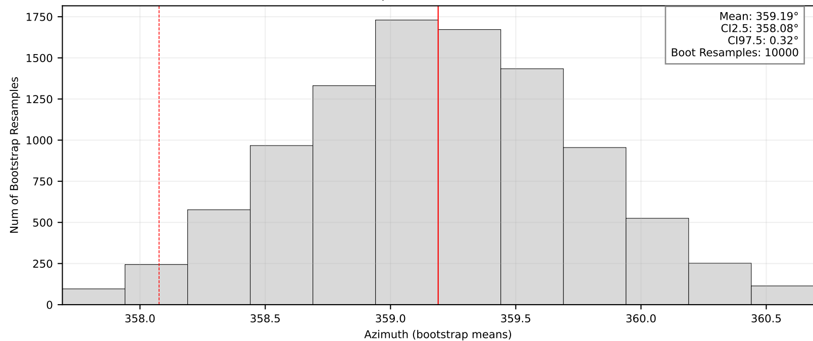
Bootstrap Means/95% CI: BK.MHC
