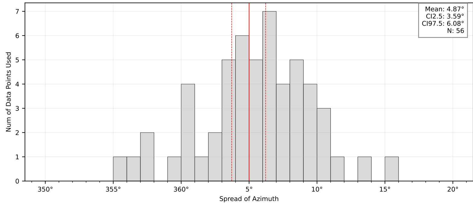
Bootstrap Mean and Confidence Intervals: BK.PIT6
