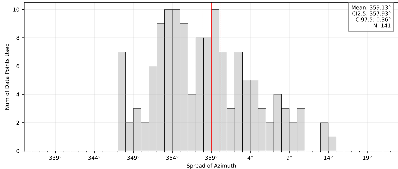
Bootstrap Mean and Confidence Intervals: BK.RAVE
