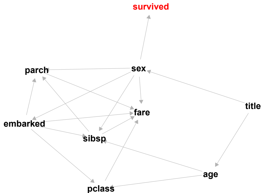
Figure 17: Bayesian Network (BN2).
