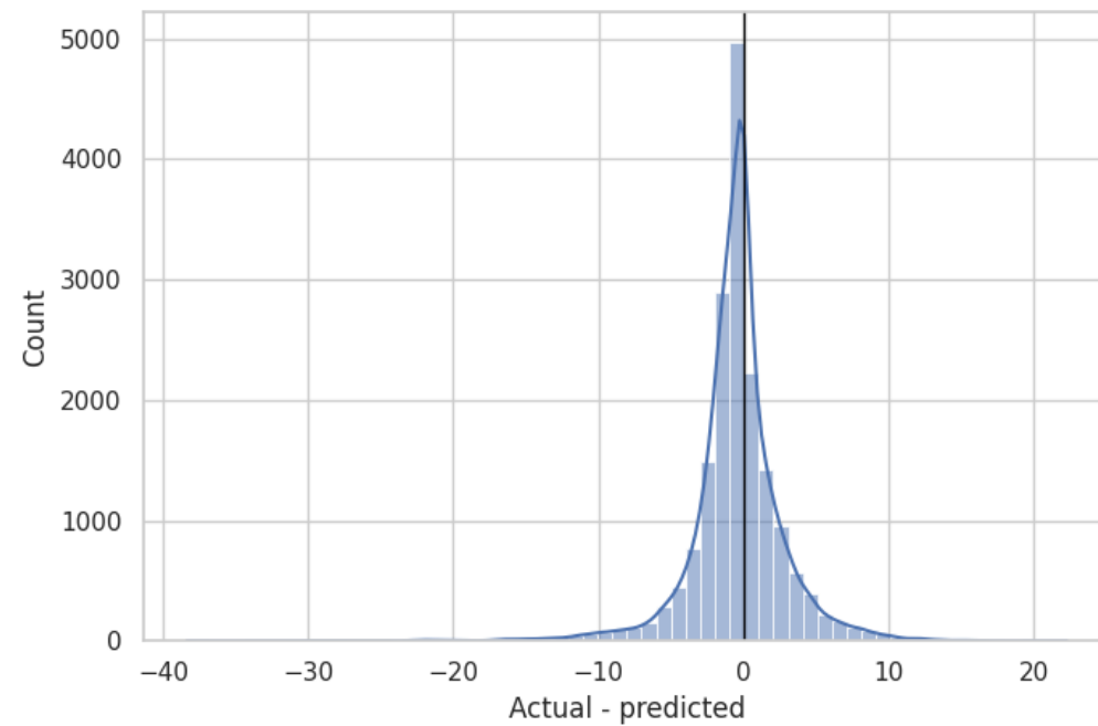
Test Residual Distribution
