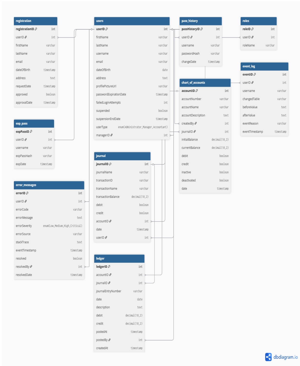
Figure 2: Database Diagram
