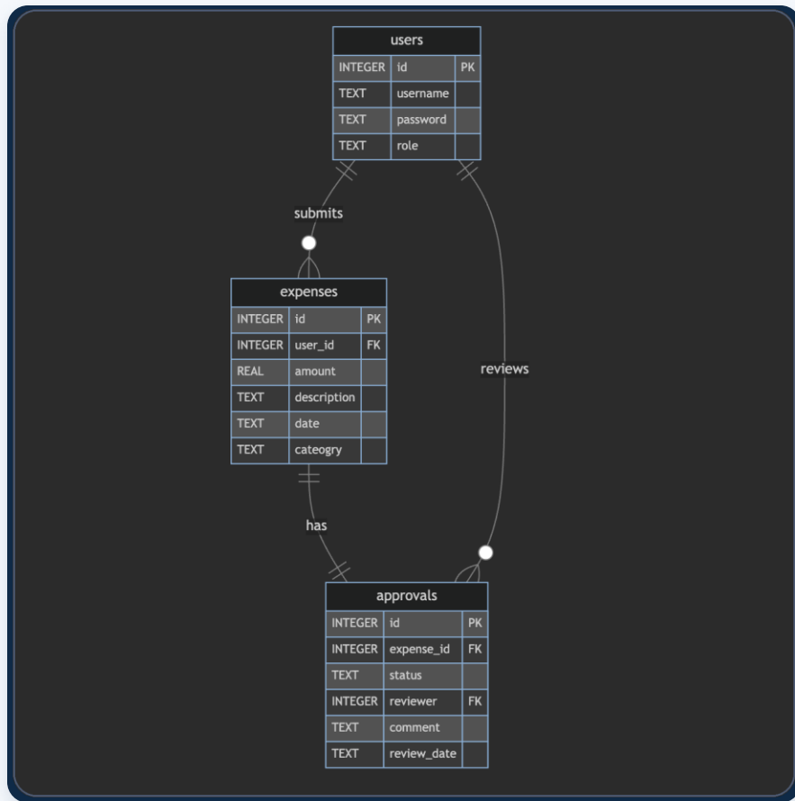
Entity Relationship Diagram · users · expenses · approvals
