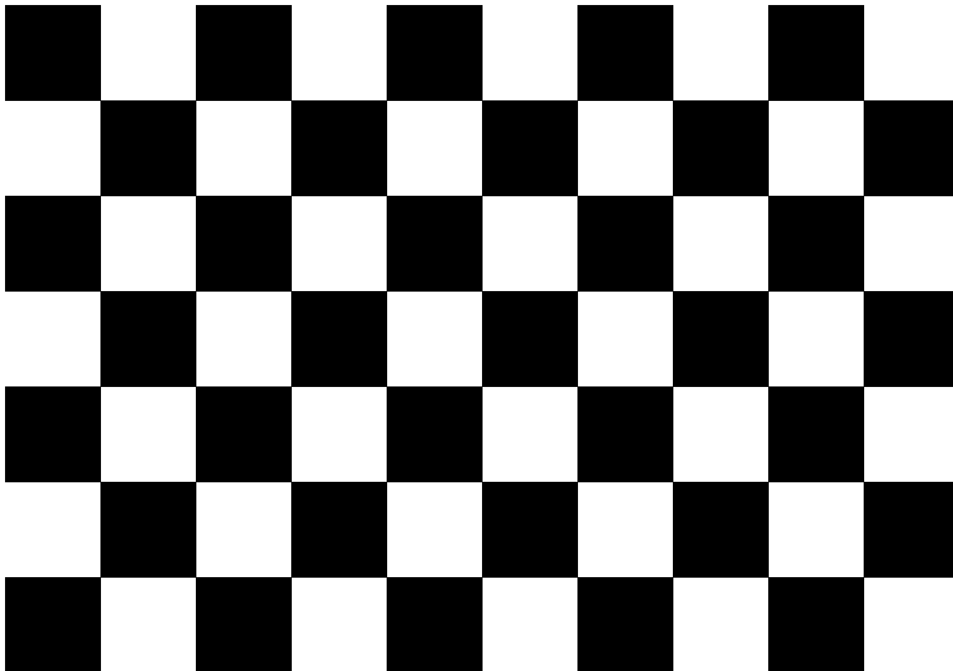
Checkerboard 9×6 inner corners | 25 mm squares | Board 250×175 mm
