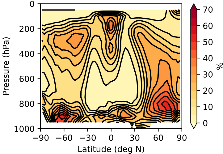
(a) Cloud fraction (3600ppm, DJF)
