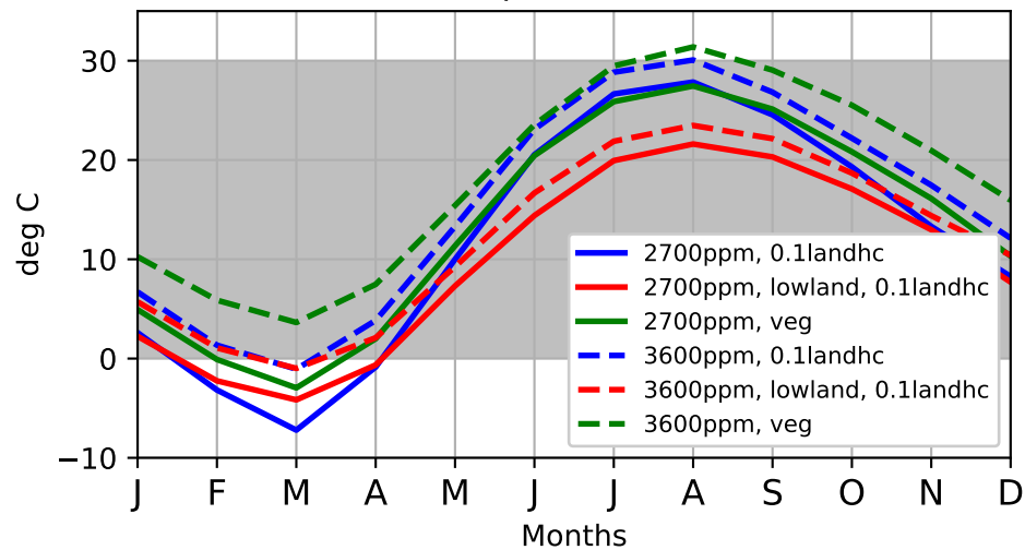
(c) Surface temperature (land, >70 lat)
