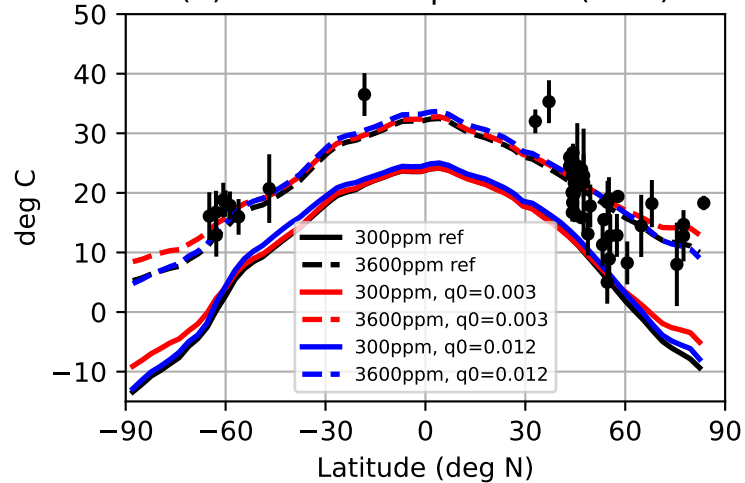
(b) Surface temperature (land)
