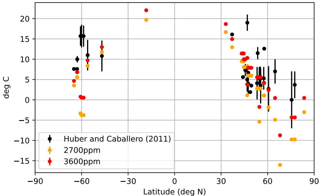
Cold month mean land temperature pointwise comparison
