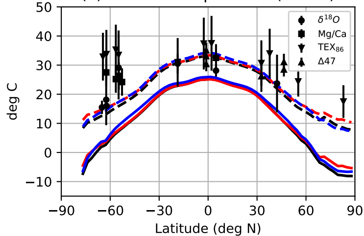
(a) Surface temperature (ocean)
