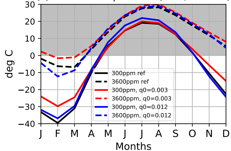
(c) Surface temperature (land, >70 lat)
