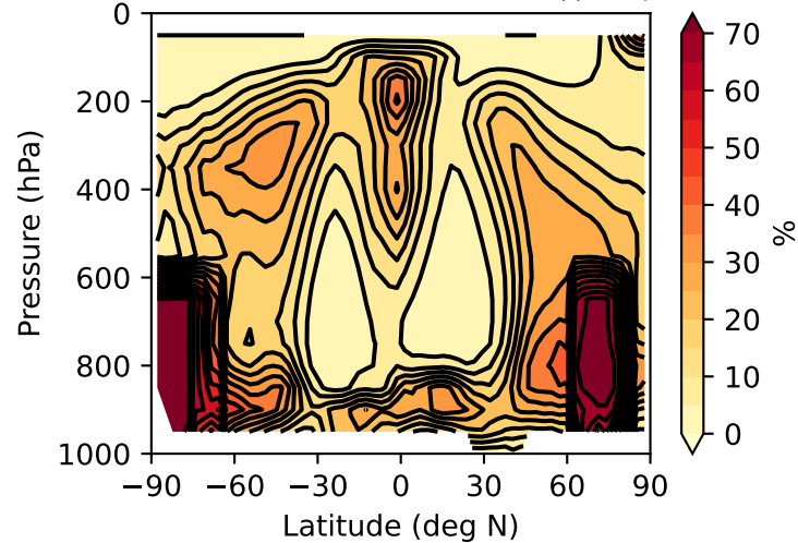
(c) Cloud fraction (low land 0.7, 3600ppm, DJF)
