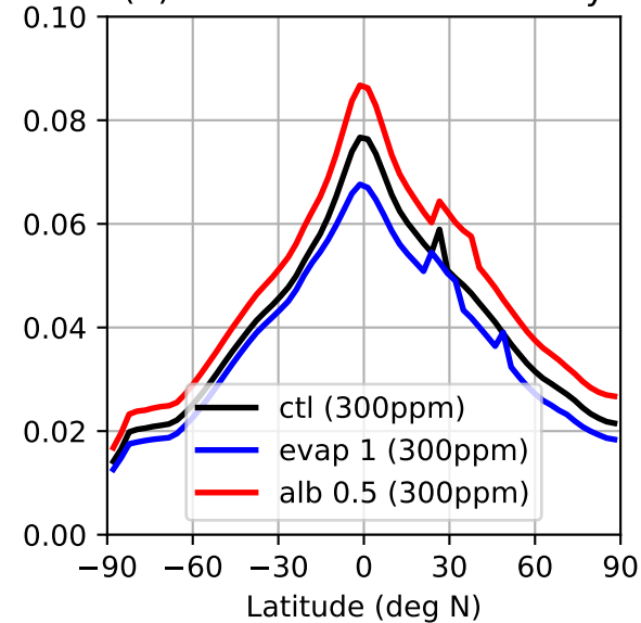
(h) Vertical sum of humidity
