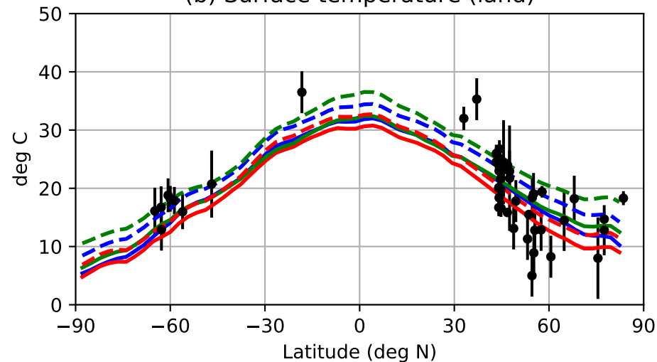
(b) Surface temperature (land)
