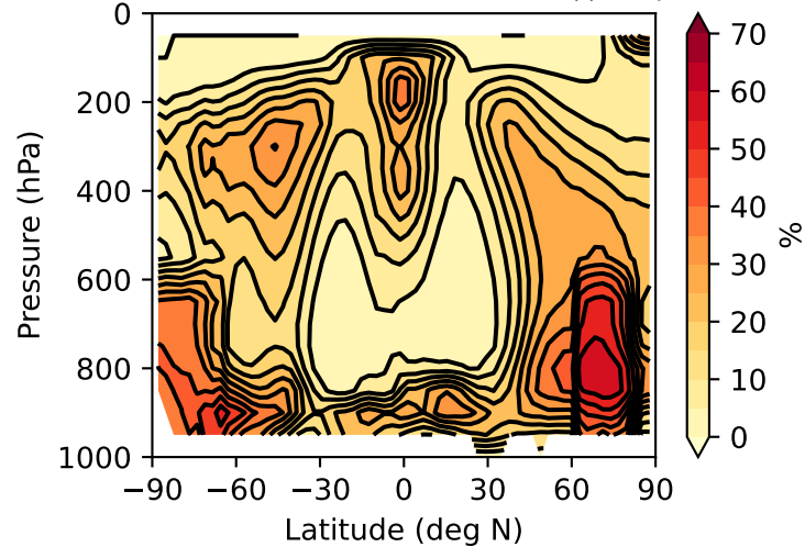
(b) Cloud fraction (low land 0.35, 3600ppm, DJF)
