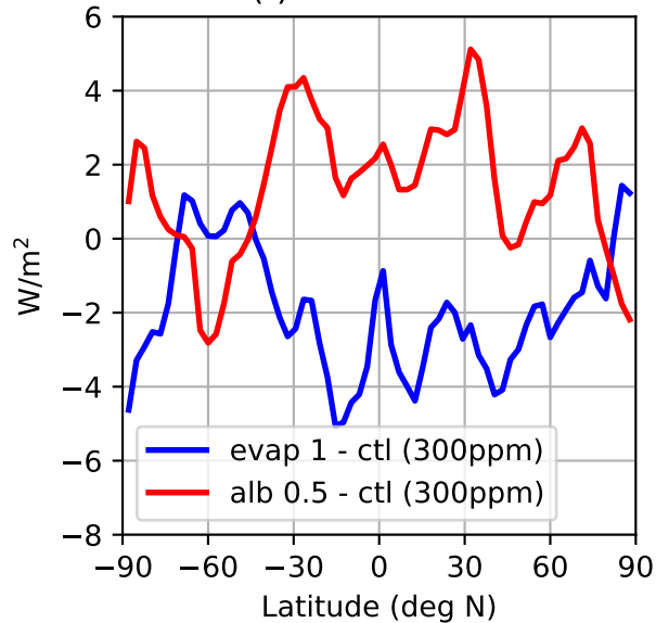
(f) TOA net SW
