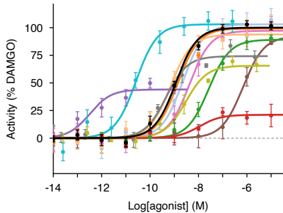
Pooled cAMP inhibition assay
