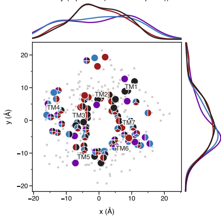
LoF · x-y (top-down (membrane plane))
