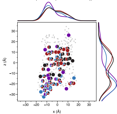
LoF · x-z (side view (ChimeraX camera))
