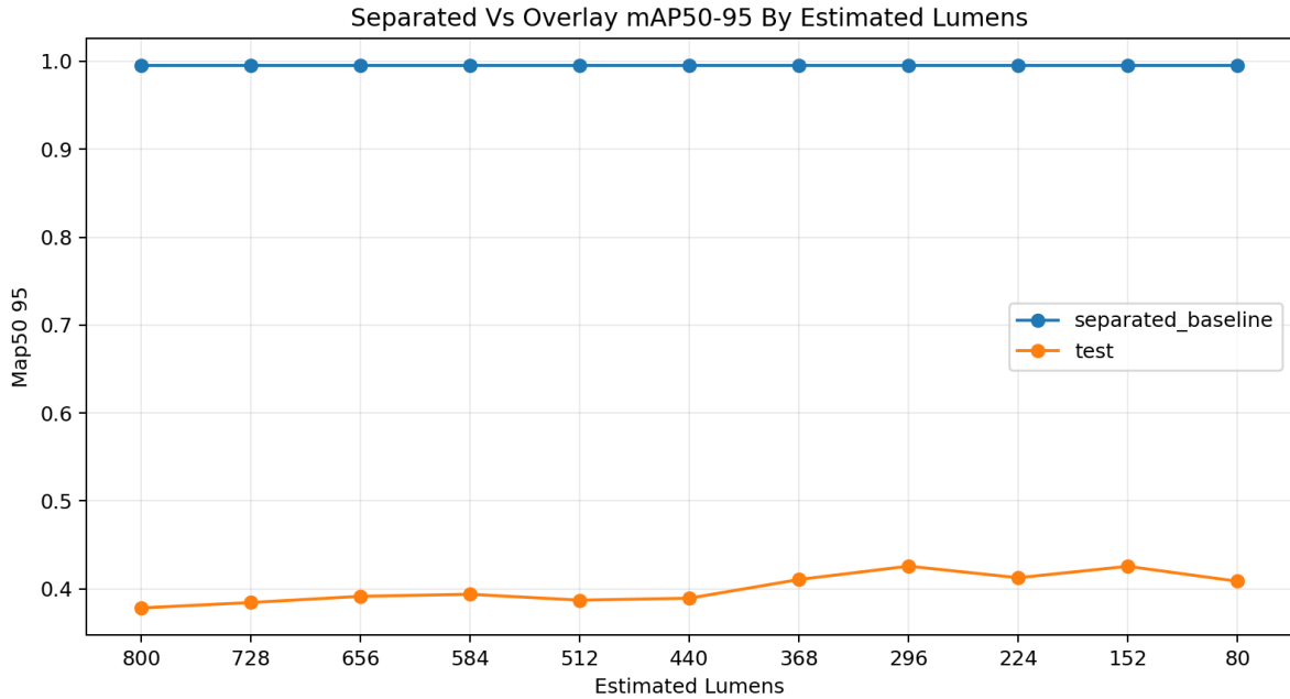
Figure 3: Separated versus overlay layout: mAP50-95 across the estimated-lumens range. The overlay condition produces the largest degradation (mAP50-95 = 0.389).
