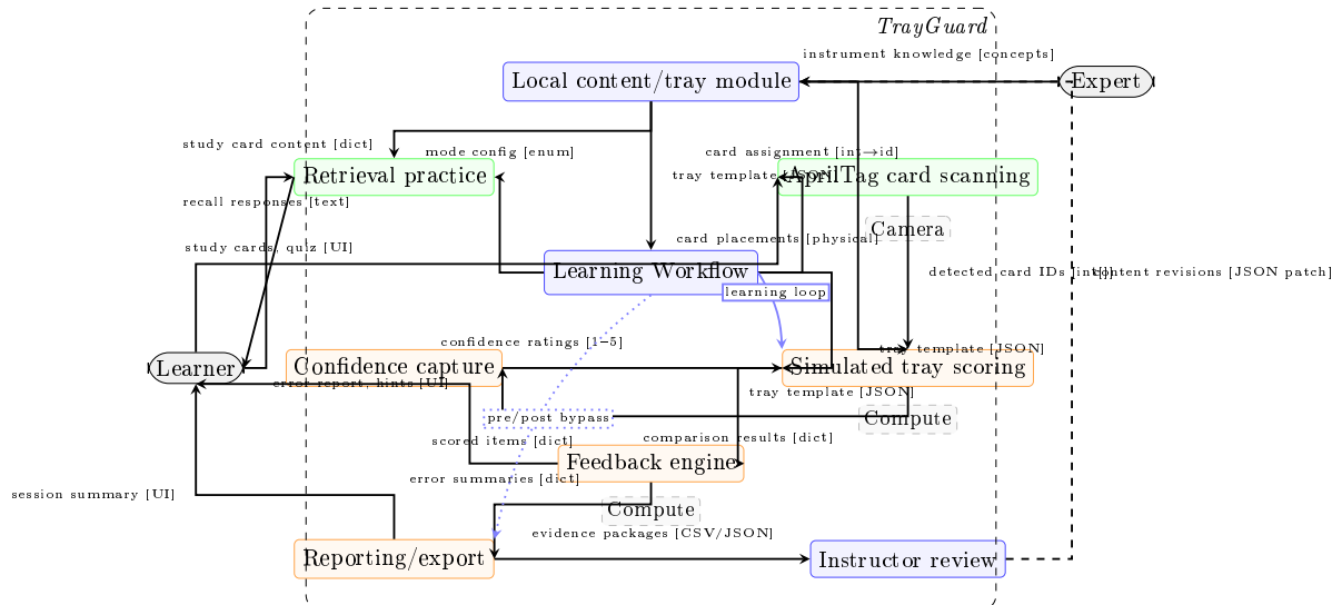
Figure 5: Functional block diagram. Please I really tried.
