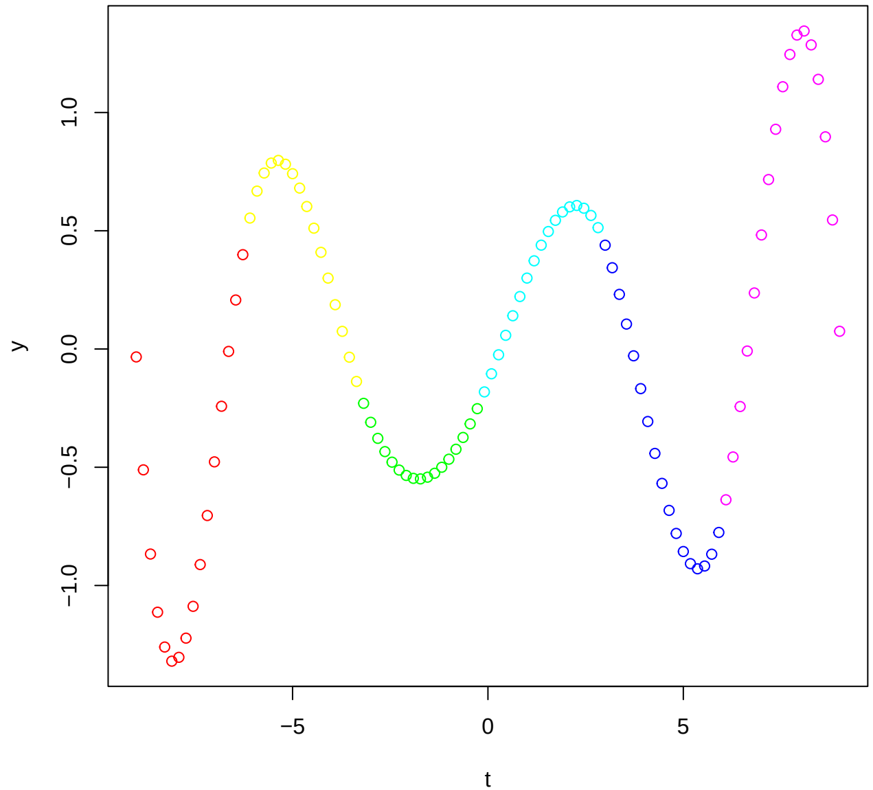
Fitted Function
