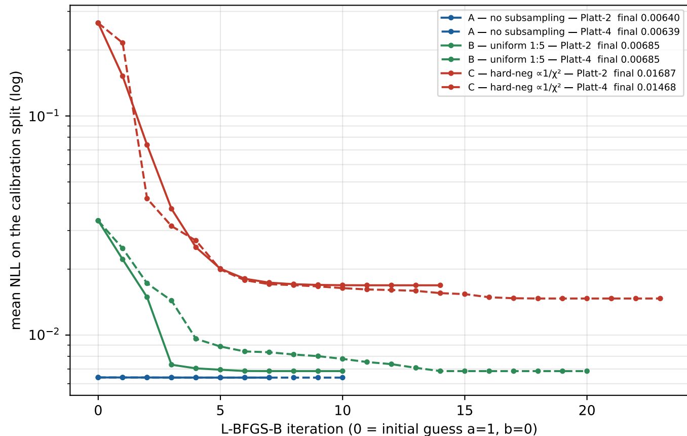
F4 Calibration fit convergence. The NLL is convex in the Platt parameters, so these traces are monotone and the optimum is global — the curve shows cost, not risk of a bad local minimum.
