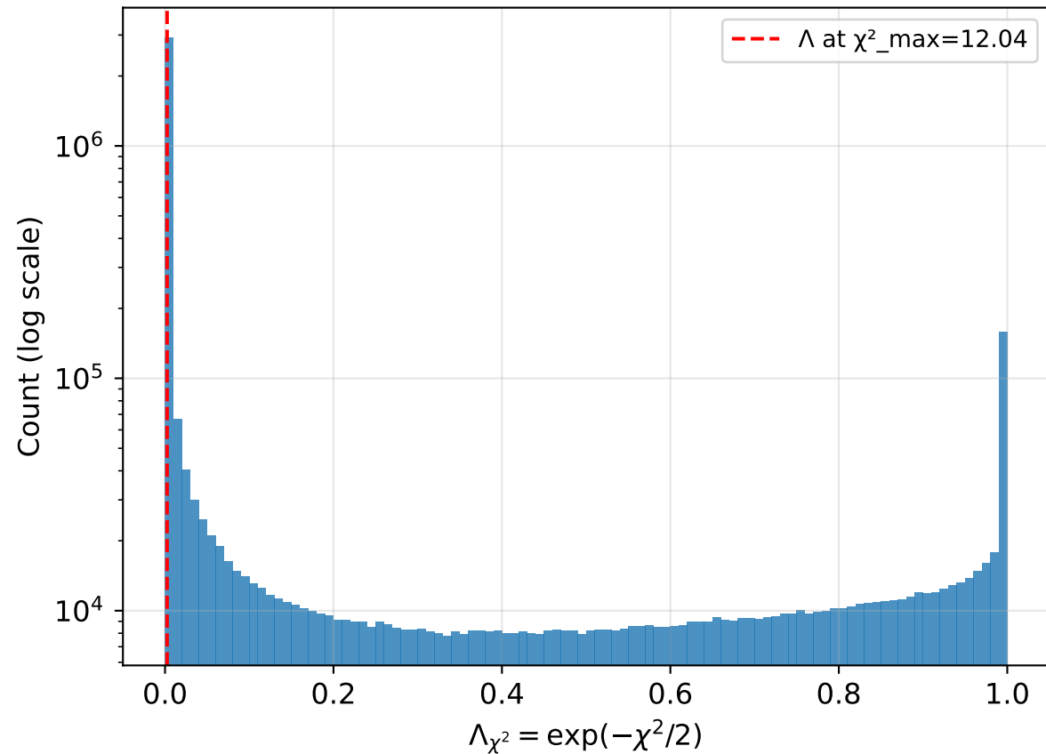
Distribution of Predicted Probabilities (all candidates)
