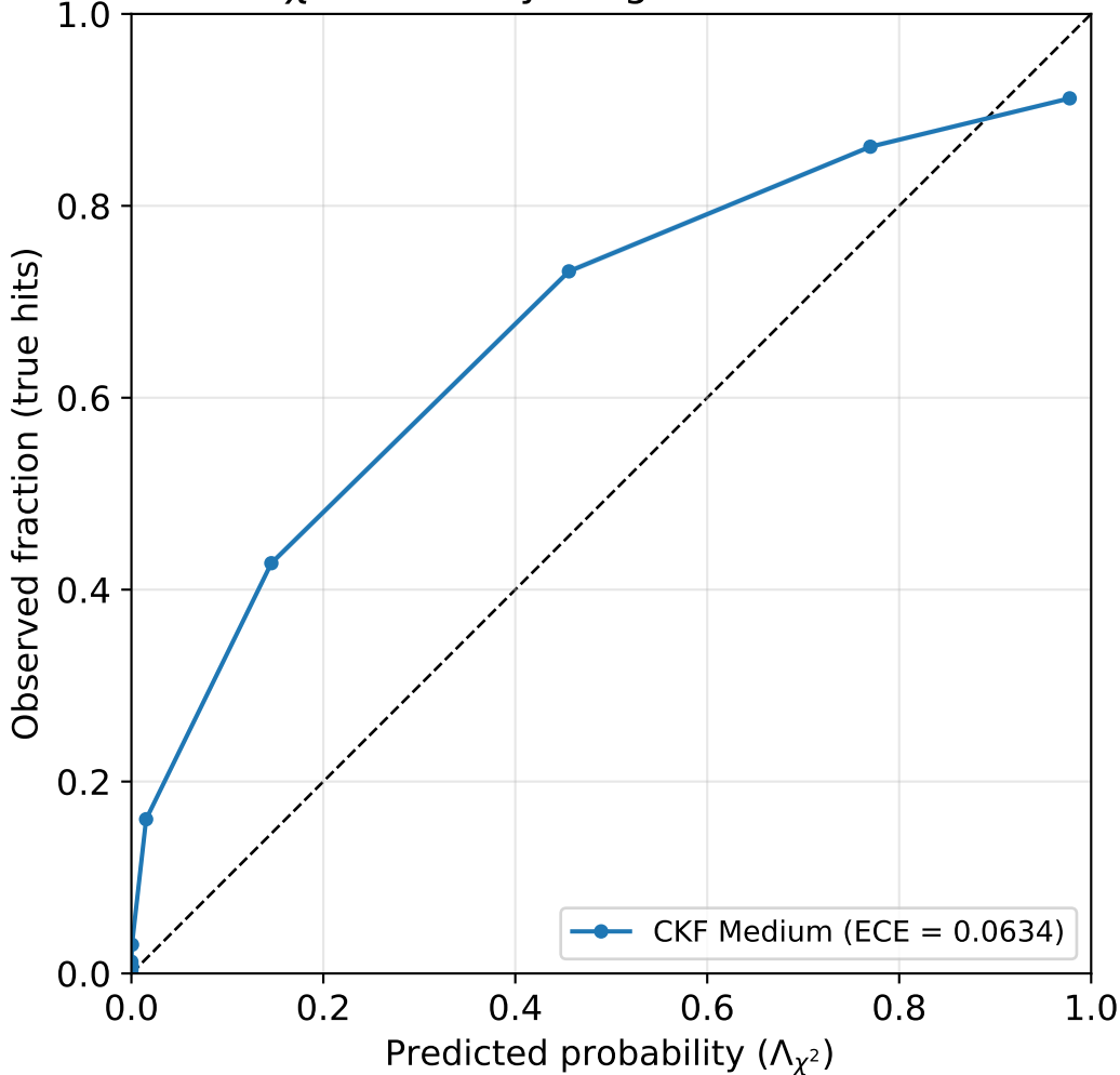
CKF \chi^2 Reliability Diagram — Medium OP
