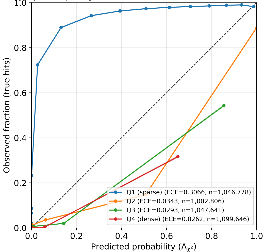
Reliability by Occupancy Quartile (Window Count ( 10\sigma bounding box))
