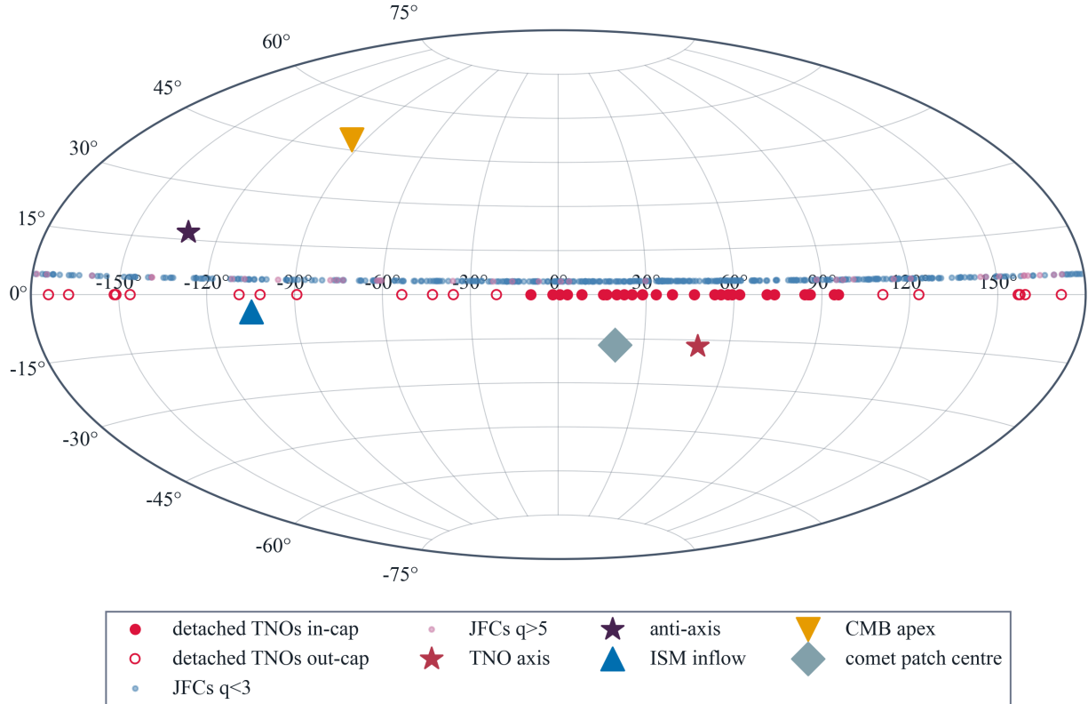
Figure 6: Every measured population on one ecliptic projection ( \lambda, \beta ). Filled circles: detached TNOs inside the 60° axis cap; open circles: detached TNOs outside it; small dots: the injected JFC chain ( q < 3 AU blue, q > 5 AU purple). Reference directions: TNO axis (red star), independently recovered comet patch centre (teal diamond), ISM inflow (blue triangle), CMB apex (orange triangle), anti-axis (purple star). The resident cluster, the transit patch, and the injected chain all land on the same axis. Pipeline output: step 057 ( results/figures/step_b22_one_map.png ).
