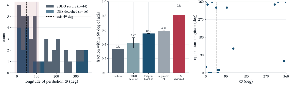
Figure 1: Independent-survey resident audit (step 085). The 16 DES detached objects ( a > 150 , q > 30 AU) scored against the pre-declared \varpi cap: 13 land inside (filled), with the cohort resultant about \bar{\varpi} = 23.3^\circ inside the registered interval — against a uniform expectation of 1/3 and the cohort's own elevated discovery-footprint baseline of 0.55. Pipeline output: step 085 ( results/figures/step_b50_des_resident.png ).
