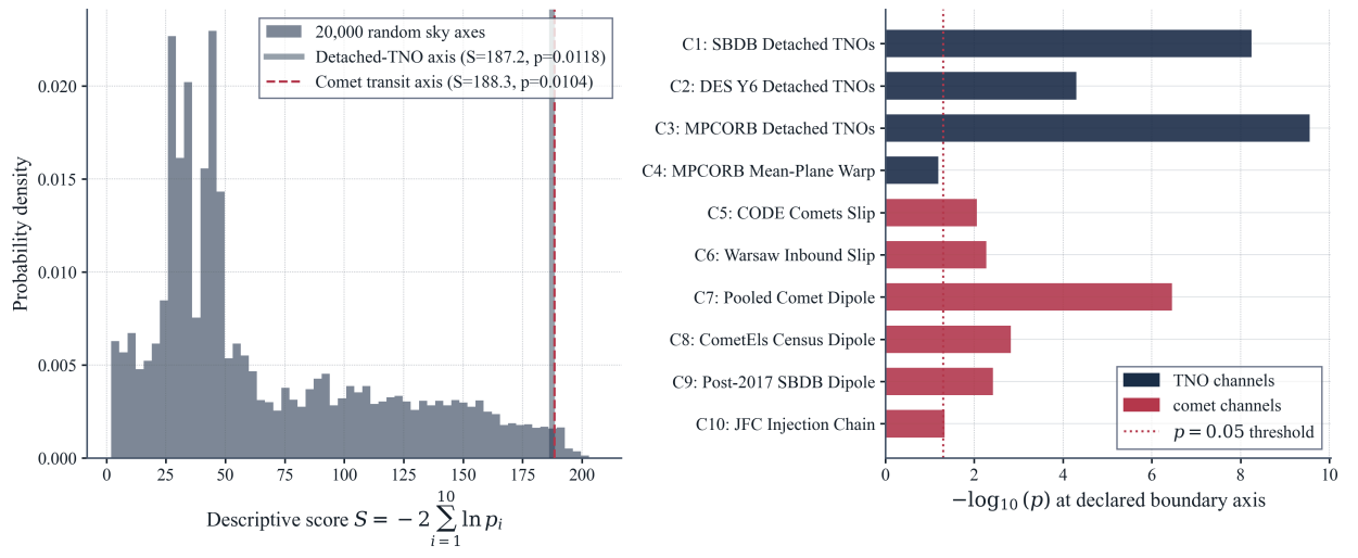
Figure 7: Ten-channel global cross-survey and multi-lineage synthesis (step 126). Left: distribution of the omnibus Fisher statistic S_{10} across 20,000 random sky directions (grey), against the values evaluated at the resident detached-TNO axis ( S_{10} = 187.2 , direction-permutation rank p = 0.0118 , solid) and the comet transit axis ( S_{10} = 188.3 , p = 0.0104 , red dashed) — both declared directions sit at the extreme upper edge of the random-direction landscape. Right: per-channel -\log_{10}(p) evaluated at the declared boundary axis for all ten channels across six catalogue lineages (SBDB, DES, MPCORB, CODE, Warsaw, CometEls; resident-population channels navy, comet channels red; dotted line: p = 0.05 ), demonstrating that the convergence is carried by the ensemble rather than any single catalogue. Pipeline output: step 126 ( results/figures/step_b90_global_synthesis.png , results/step_b90_global_synthesis.json ).
