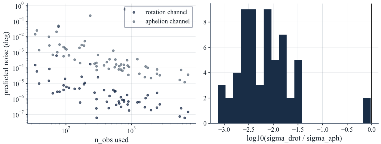
Figure 5: Reconstruction-error sensitivity audit of the two-channel dissociation (step 150). Each post-2017 dual-leg member's published SBDB element sigmas are injected as independent Monte-Carlo perturbations (16 primary draws plus two restricted-element sets of 10 draws per object) and propagated to the boundary sphere under the identical force model. Left: per-object predicted noise on the leg-rotation and aphelion-direction observables versus observation count — the rotation channel sits about two orders of magnitude lower at every quality stratum. Right: the per-object sensitivity ratio \sigma_{\Delta\varpi}/\sigma_{\text{aph}} — no member's rotation channel is the more error-exposed (median ratio 0.00612), and at the error amplitude required to fake the rotation residual the same perturbation would displace the aphelion datum by \sim 0.61^\circ . Pipeline output: step 150 ( results/figures/supplementary/step_b114_channel_dissociation.png ).
