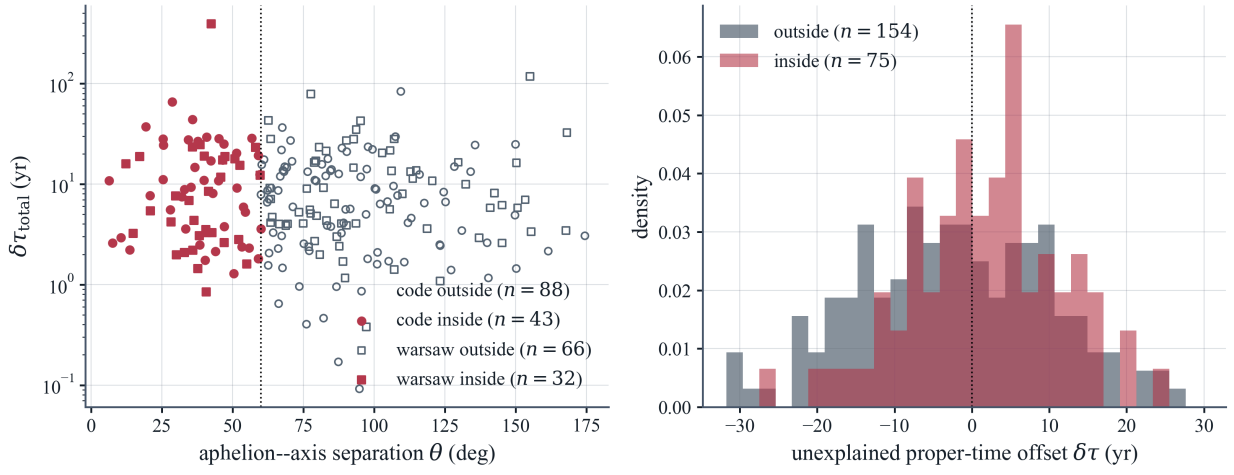
Figure 3: The transit anomaly in equivalent orbital time units. Left: \delta\tau_{\text{total}} = \delta\theta r_b^2/h for the pooled CODE (circles) and Warsaw (squares) cohorts versus aphelion-axis separation; the in-cap points (red) sit systematically high. Right: the residual after regression on the measured encounter budget. This conversion is not itself a proper-time measurement. Pipeline output: step 065 ( results/figures/step_b30_proper_time_slip.png ).
