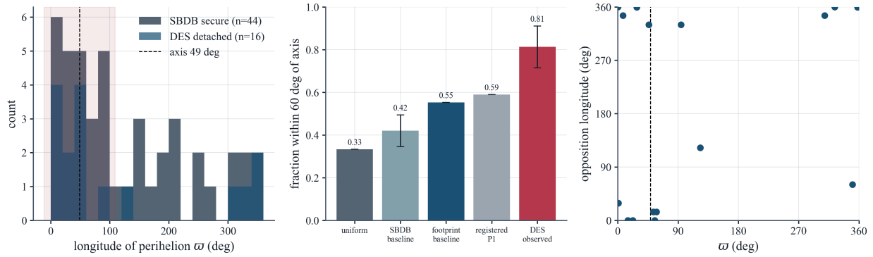
Figure 1: Independent-survey resident audit (step 085). The 16 DES detached objects ( a > 150 , q > 30 AU) scored against the pre-declared \varpi cap: 13 land inside (filled), with the cohort resultant about \bar{\varpi} = 23.3^\circ inside the registered interval — against a uniform expectation of 1/3 and the cohort's own elevated discovery-footprint baseline of 0.55. Pipeline output: step 085 ( results/figures/step_b50_des_resident.png ).
