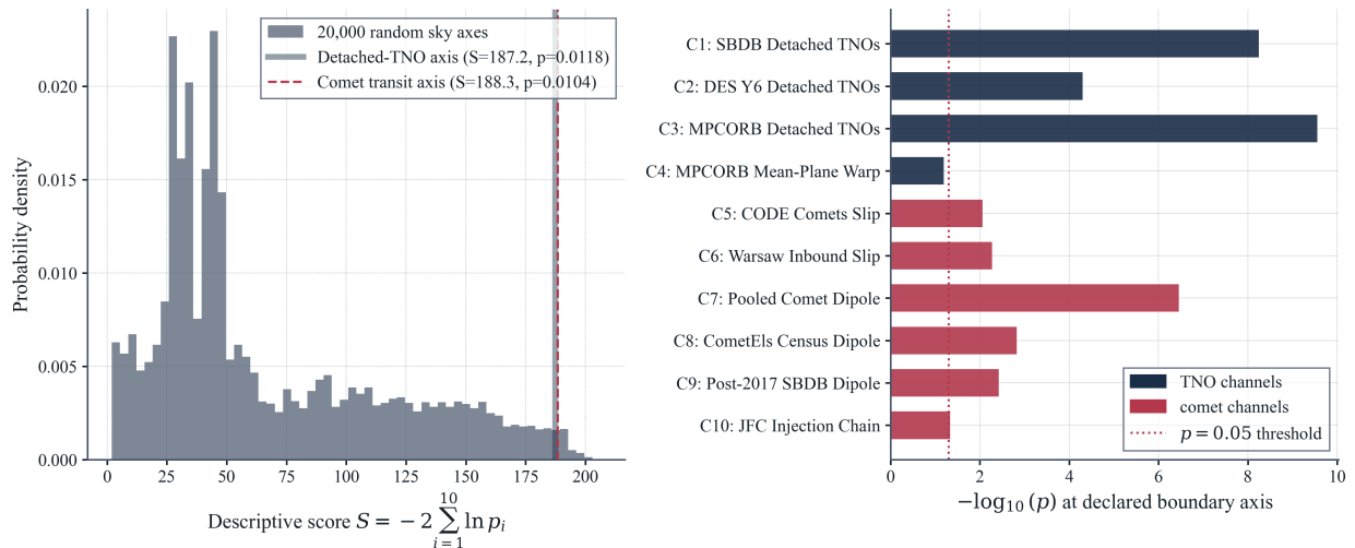
Figure 6: Ten-channel global cross-survey and multi-lineage synthesis (step 126). Left: distribution of the omnibus Fisher statistic S_{10} across 20,000 random sky directions (grey), with the 95th, 99th, and 99.9th percentiles marked, against the values evaluated at the resident detached-TNO axis ( S_{10} = 187.2 , p = 0.012 , red dashed) and the comet transit axis ( S_{10} = 188.3 , p = 0.010 , teal dotted). Right: on-sky directions of all ten channels across six catalogue lineages (SBDB, DES, MPCORB, CODE, Warsaw, CometEls), demonstrating tight convergence on the declared 60^\circ boundary sector (dashed circle). Pipeline output: step 126 ( results/figures/step_b90_global_synthesis.png , results/step_b90_global_synthesis.json ).
