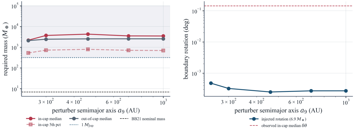
Figure 7: Perturber distance ladder (step 087). The in-cap required perturber mass — the mass an inserted point mass would need to inject the catalogued rotation — as a function of perturber semimajor axis, 250–1000 AU. The median bound stays at brown-dwarf scale throughout ( \sim 2186\text{--}4290 M_{\oplus} ; m_{\text{req}} \propto a_9^{+0.2} ) and 100 per cent of in-cap comets require more than a Jupiter mass at every rung — the dotted line marks the one-Jupiter-mass level, 318 M_{\oplus} , which the required mass exceeds at every rung. Right panel: the rotation a nominal 6.9 M_{\oplus} perturber actually injects compared with the observed in-cap median — the injected curve sits orders of magnitude below the observed level at every rung. The exclusion is geometric, not parametric. Pipeline output: step 087 ( results/figures/step_b52_distance_ladder.png ).
