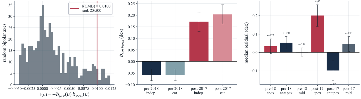
Figure 2: The bipolar unification test on the independent two-leg refit record (step 129). Left: the joint opposite-polarity statistic J(u) = -b_{\text{pre}}(u)b_{\text{post}}(u) evaluated on 500 random sky axes — the CMB-anchored axis ranks 25/500. Centre: signed CMB-frame dipole amplitude by era — the pre-2018 record carries the negative polarity, the post-2017 record the positive, on both the independent refits and the catalogued elements. Right: bipolar-cap audit — the era split reproduces on the cap-facing hemispheres while the mid-latitude control stays flat. Pipeline output: step 129 ( results/figures/step_b93_bipolar_unification.png ).
