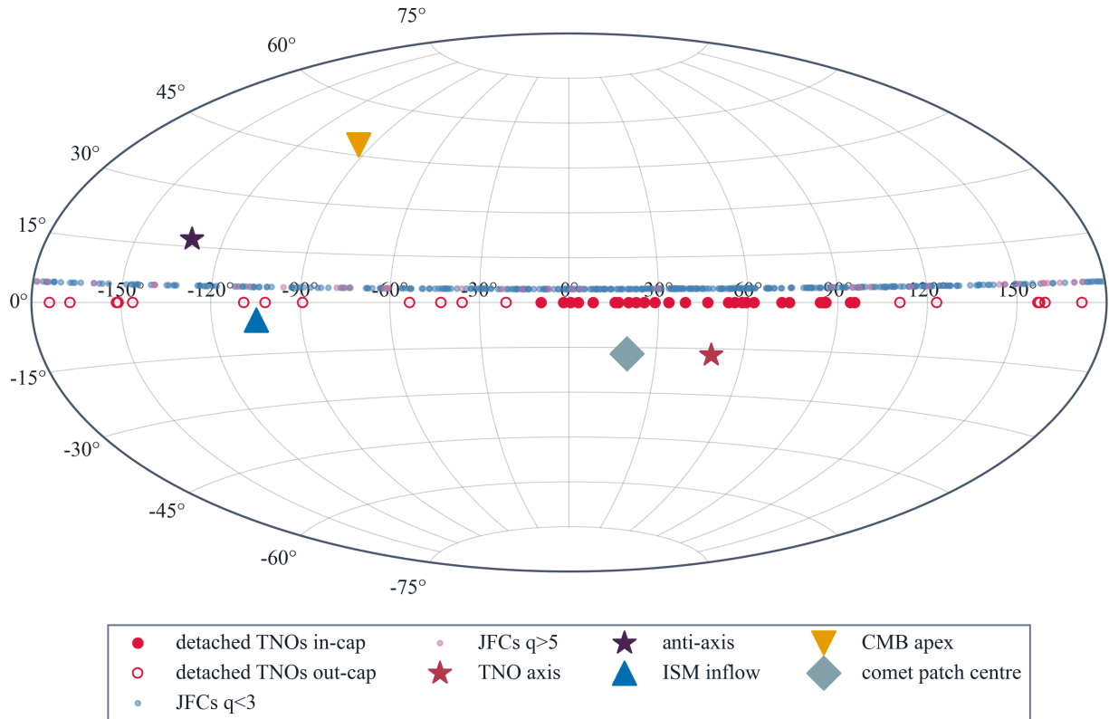
Figure 5: Every measured population on one ecliptic projection ( \lambda, \beta ). Filled circles: detached TNOs inside the 60^\circ axis cap; open circles: detached TNOs outside it; small dots: the injected JFC chain ( q < 3 AU blue, q > 5 AU purple). Reference directions: TNO axis (red star), independently recovered comet patch centre (teal diamond), ISM inflow (blue triangle), CMB apex (orange triangle), anti-axis (purple star). The resident cluster, the transit patch, and the injected chain all land on the same axis. Pipeline output: step 057 ( results/figures/step_b22_one_map.png ).
