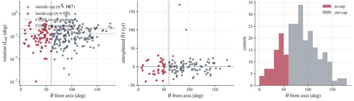
Figure 4: The prospective holdout at the pre-declared axis (step 117). Left: full-pass periapsis-direction rotation versus aphelion-axis separation for the 255 integrated post-2017 comets — the in-cap members (red) sit at or below the out-of-cap members, the CODE gradient inverted (dashed lines: the CODE in-cap and out-of-cap medians). Centre: kick-regressed unexplained slip versus axis separation — the in-cap offset is negative (median -5.5 yr). Right: the cohort's aphelion distribution about the declared axis. Pipeline output: step 117 ( results/figures/step_b81_prospective_lpc.png ).
