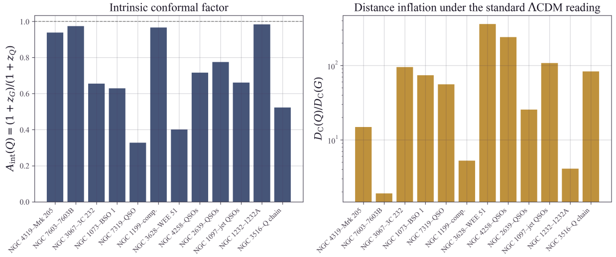
Figure 1. Left: the intrinsic conformal factor A_{\text{int}}(Q) = (1 + z_G)/(1 + z_Q) for each pair—a continuous distribution of local proper-time depths, all sub-unity. Right: the distance-inflation factor the standard redshift–distance reading requires for the same pairs, reaching a factor of 361 for the NGC 3628 minor-axis quasar.
