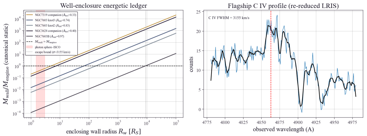
Figure 4. Left: the canonical static enclosure ledger—the wall mass in units of the engine mass against enclosing wall radius in Schwarzschild radii for the measured emitters. The wall reaches the engine mass at R_w/R_S = 6/\Delta u^2 ; the shaded band marks the photon-sphere–ISCO interior where no bound emitter can sit, and the dotted line marks the bound-gas ceiling for the flagship's measured dispersion. Right: the C IV region of the re-reduced NGC 7319 companion spectrum with its measured FWHM = 3,155 km/s—ordinary broad-line kinematics that exclude any near-horizon emitter placement.
