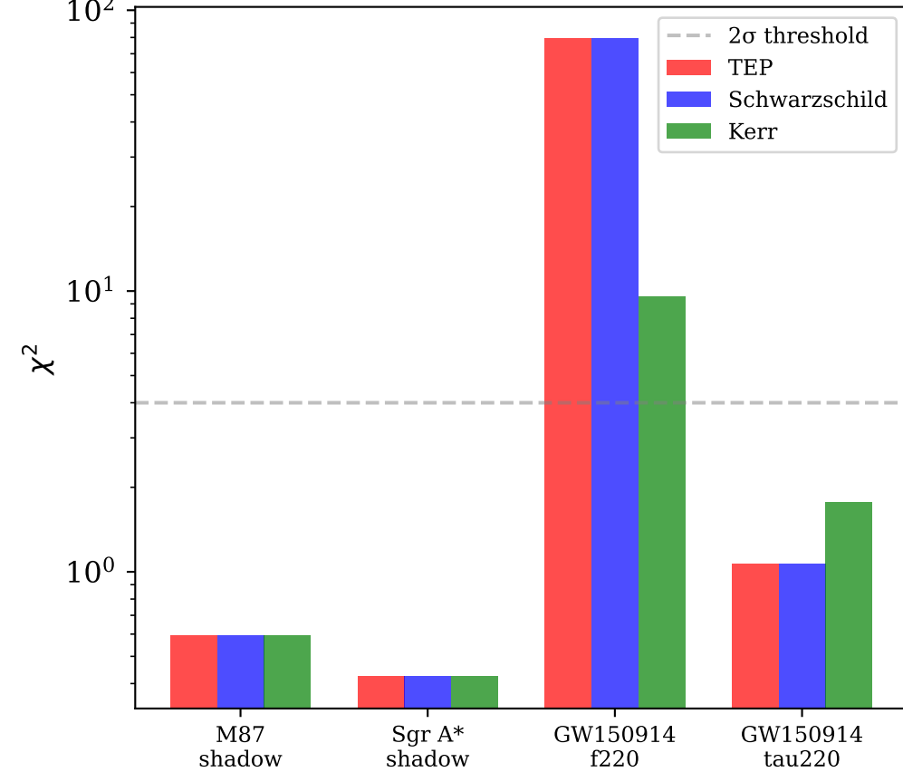
Constraint comparison
