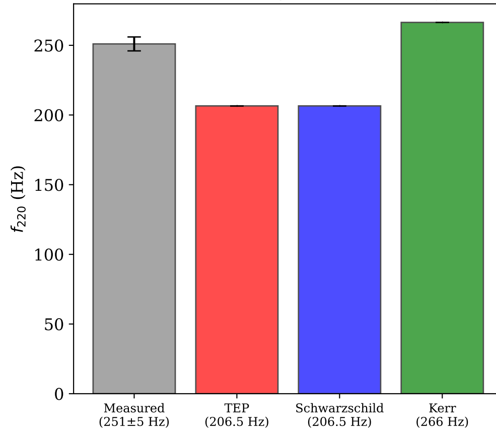
GW150914 ringdown frequency
