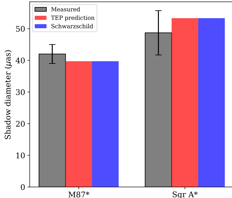
EHT shadow diameter comparison
