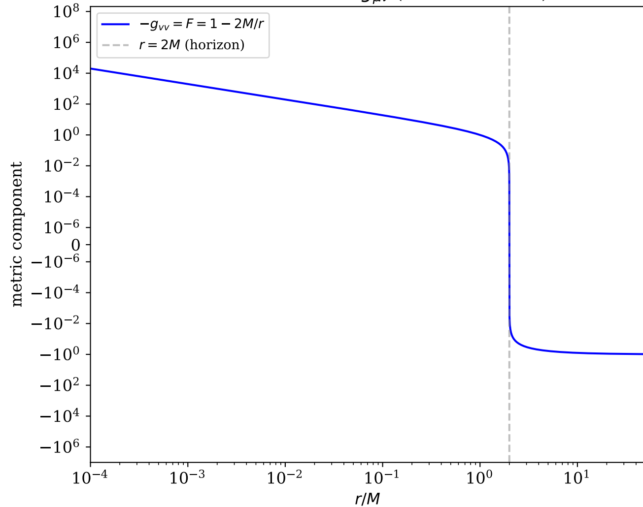
Geometric metric g_{\mu\nu} (Schwarzschild)
