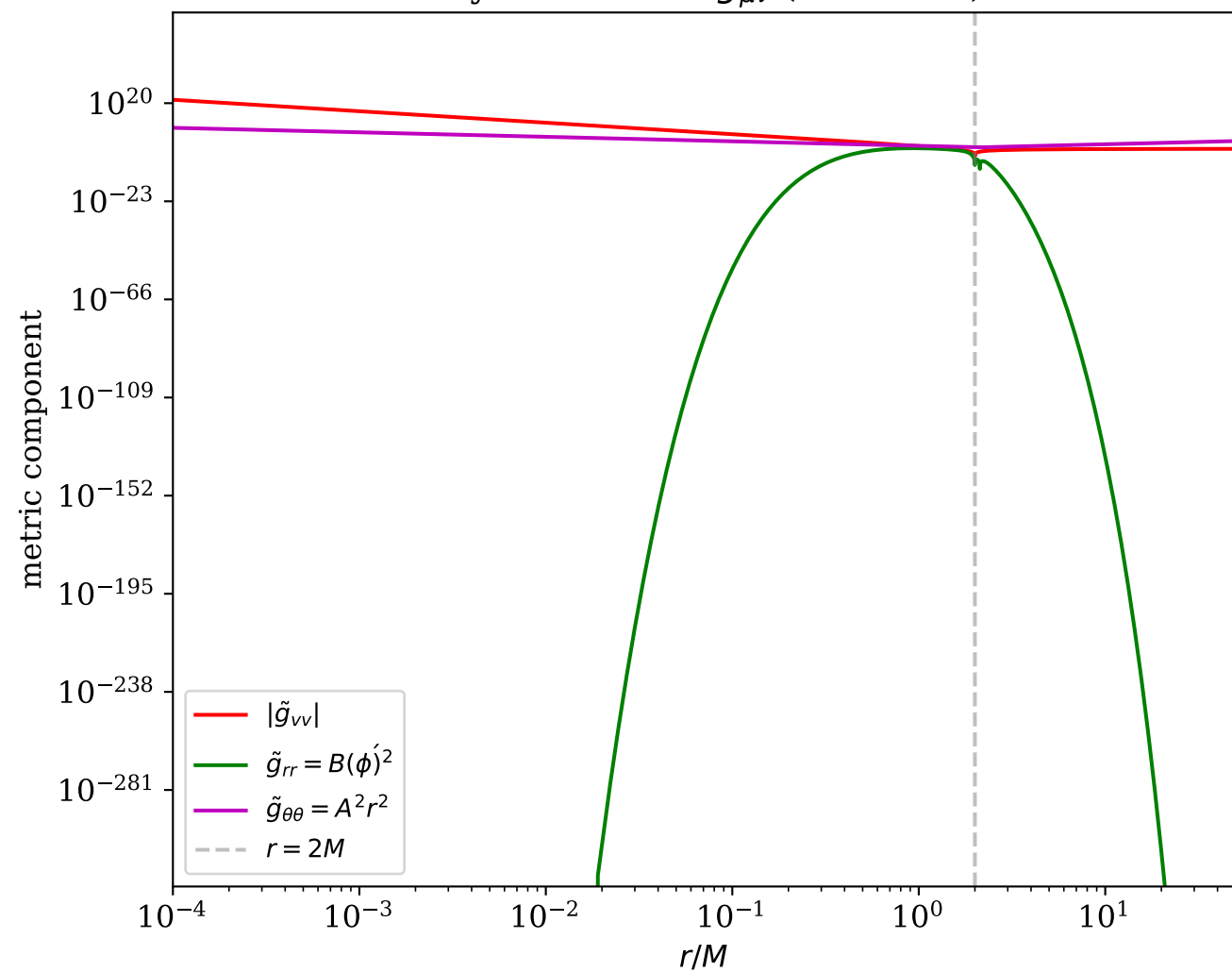
Physical metric \tilde{g}_{\mu\nu} (disformal)
