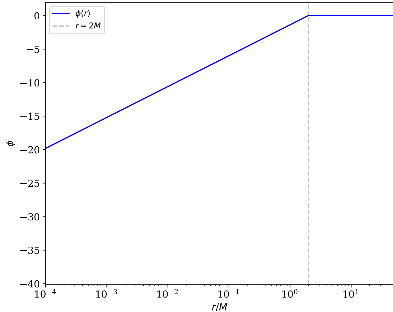
Scalar field profile
