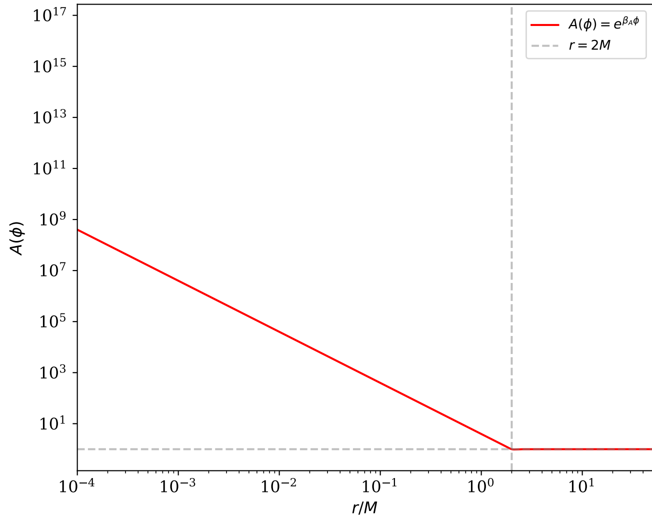
Conformal clock factor
