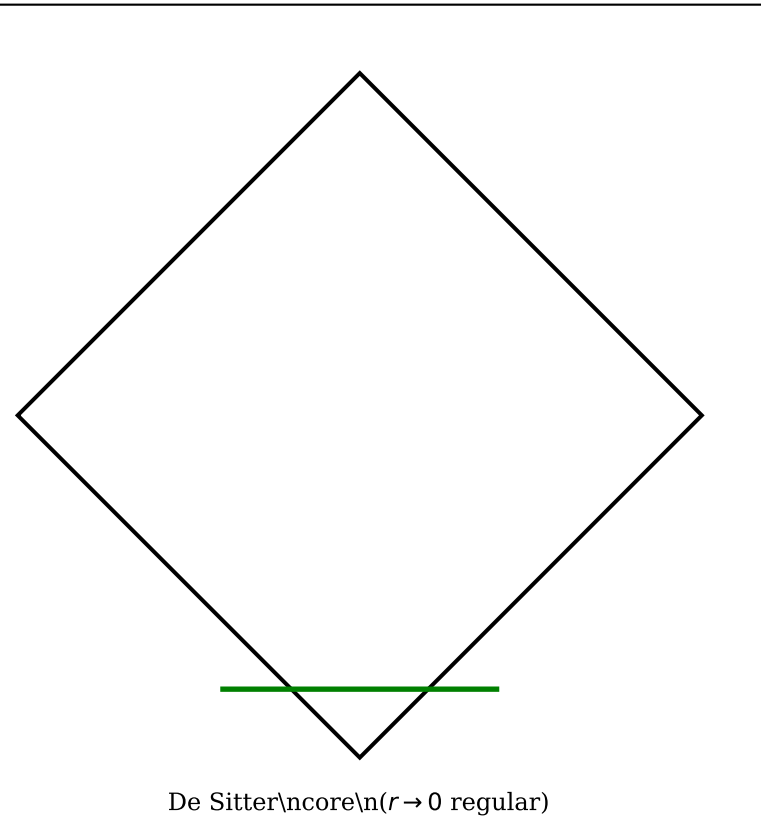
Regular BH
