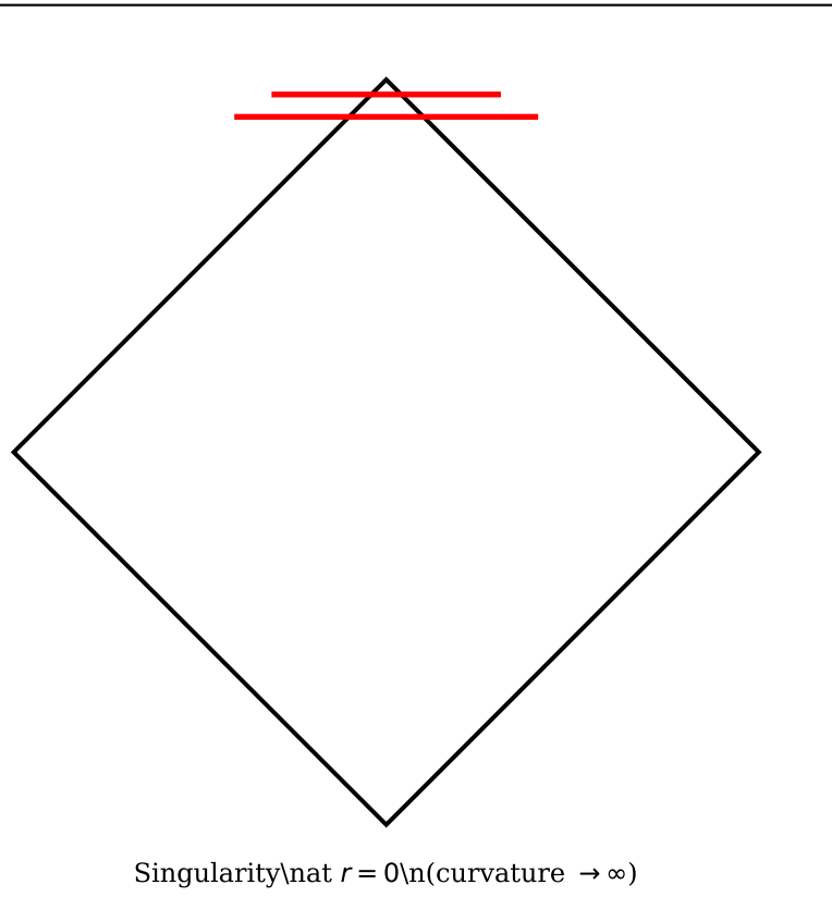
Schwarzschild
