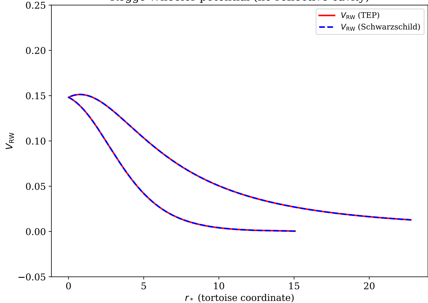
Regge-Wheeler potential (no reflective cavity)
