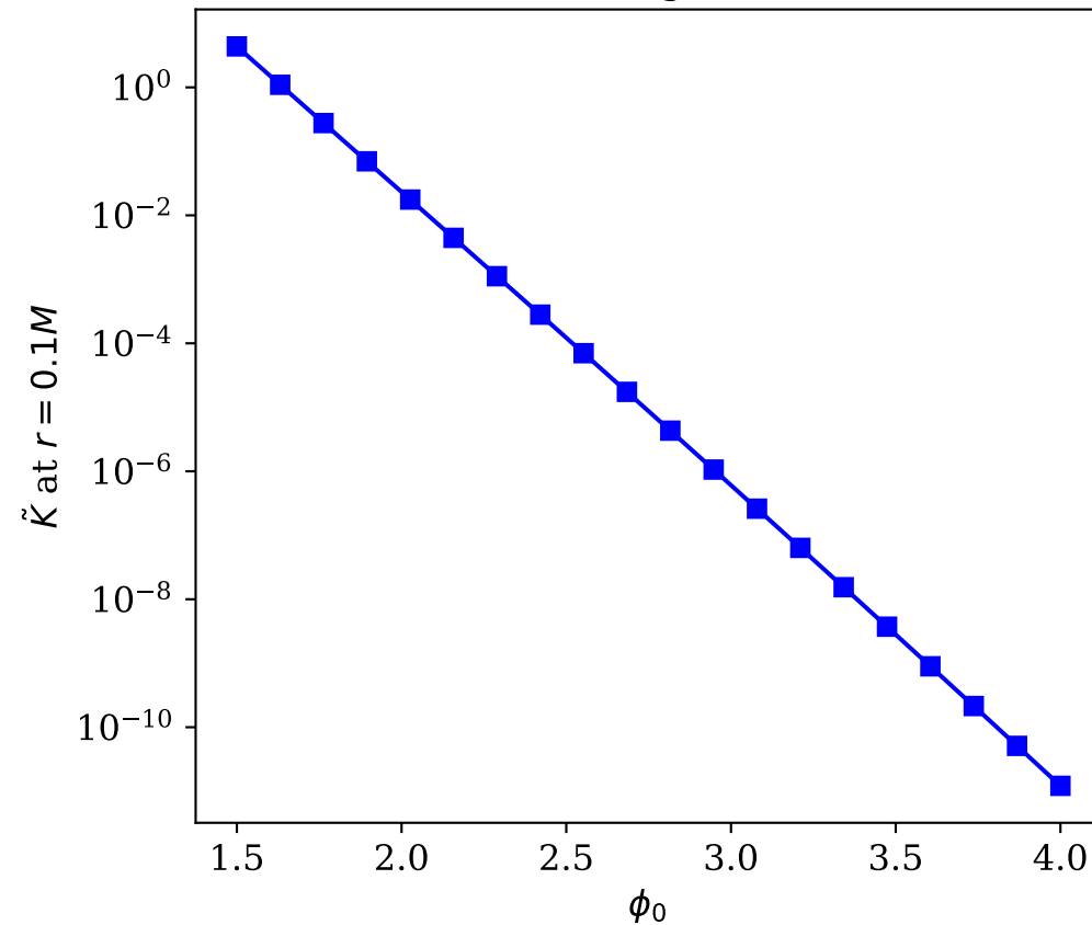
Curvature regularization
