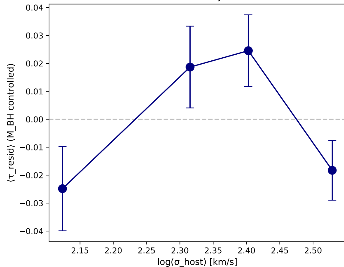
Binned Analysis
