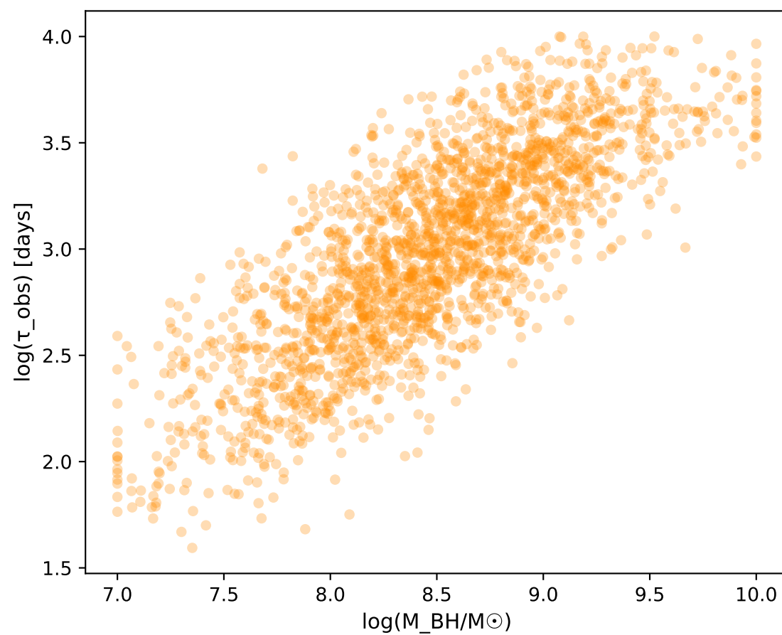
Timescale vs Black Hole Mass
