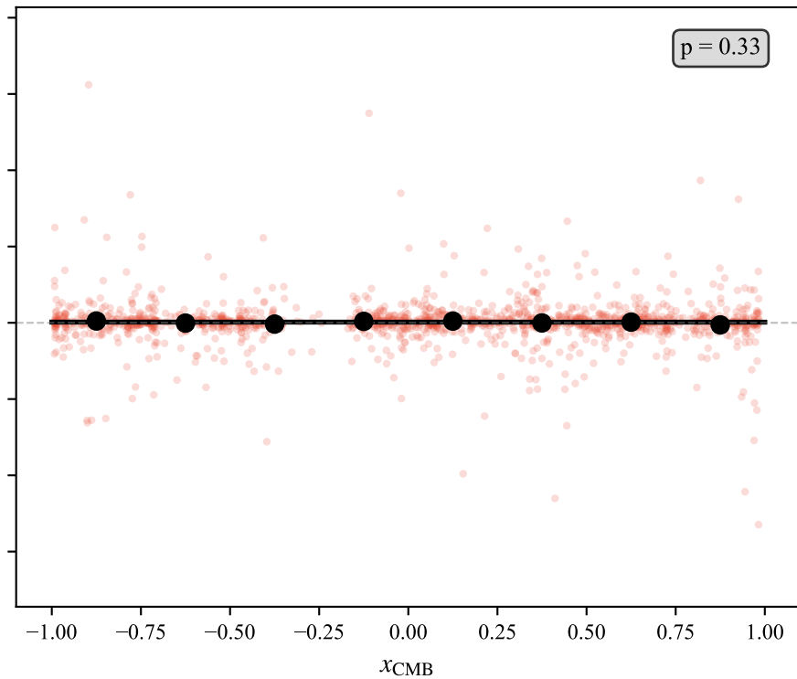
Gas Kinematics Slope = -0.1 km/s
