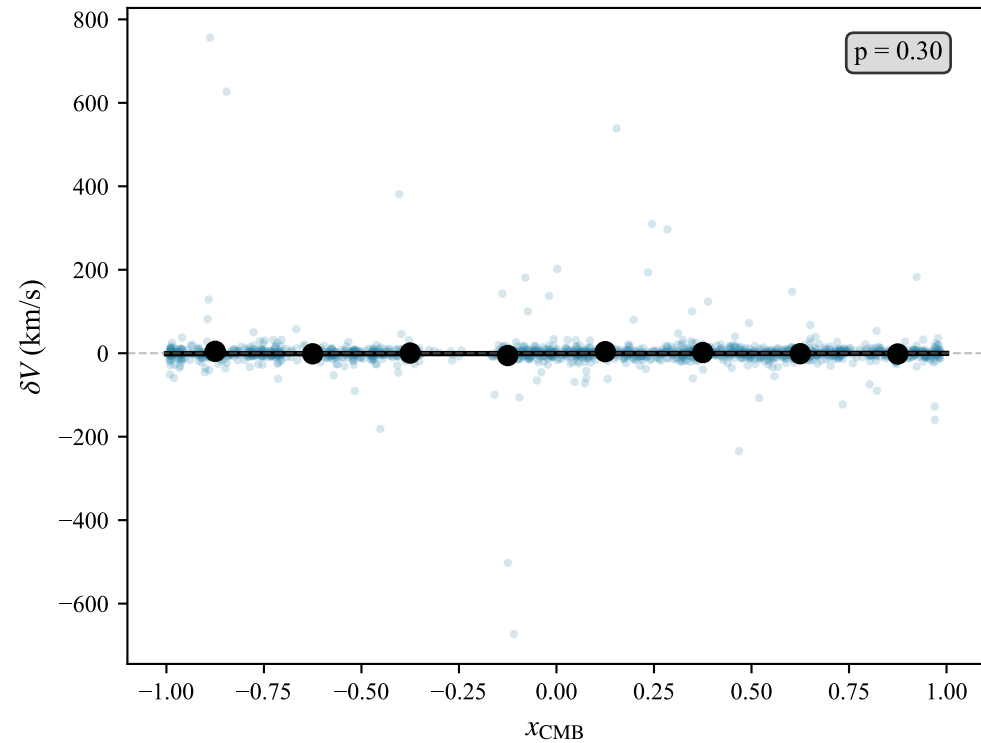
Stellar Kinematics Slope = 0.4 km/s
