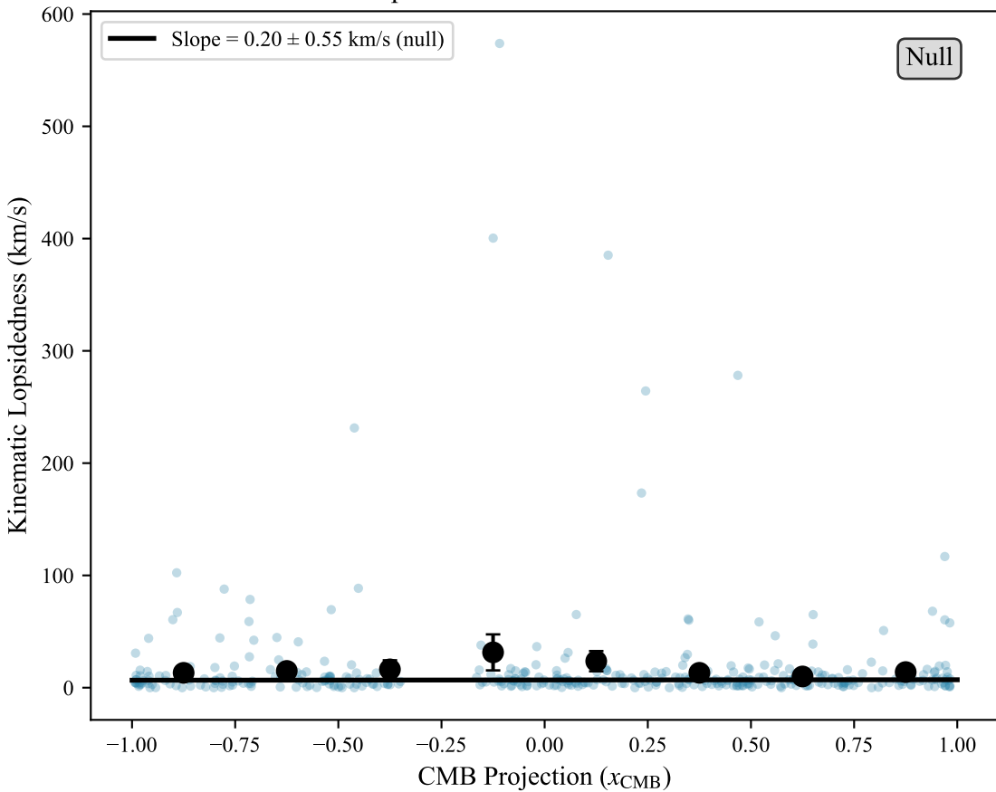
Lopsidedness-CMB Correlation
