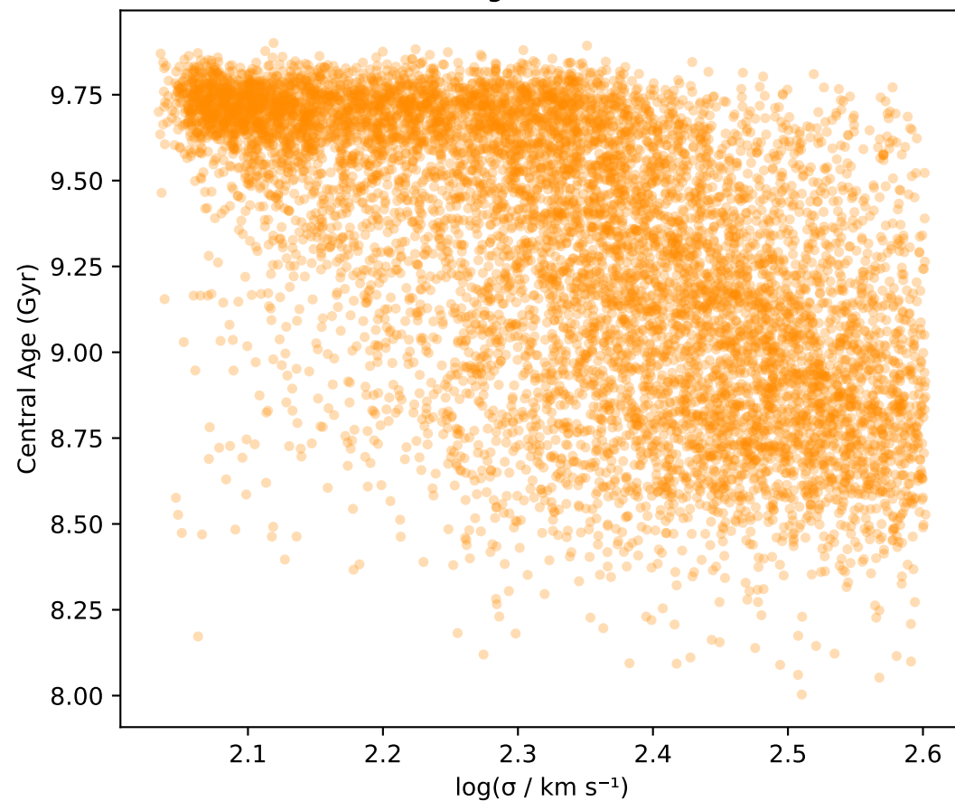
B. Central Age vs \sigma ( r = -0.603 )
