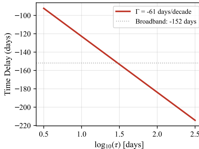
E. DESJ0408 A-D: Scale-Dependent Delay
