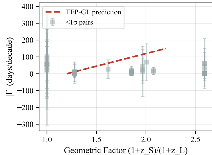
D. Temporal Shear vs Geometric Factor
