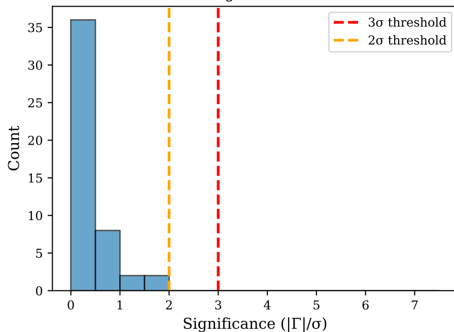
C. Detection Significance Distribution
