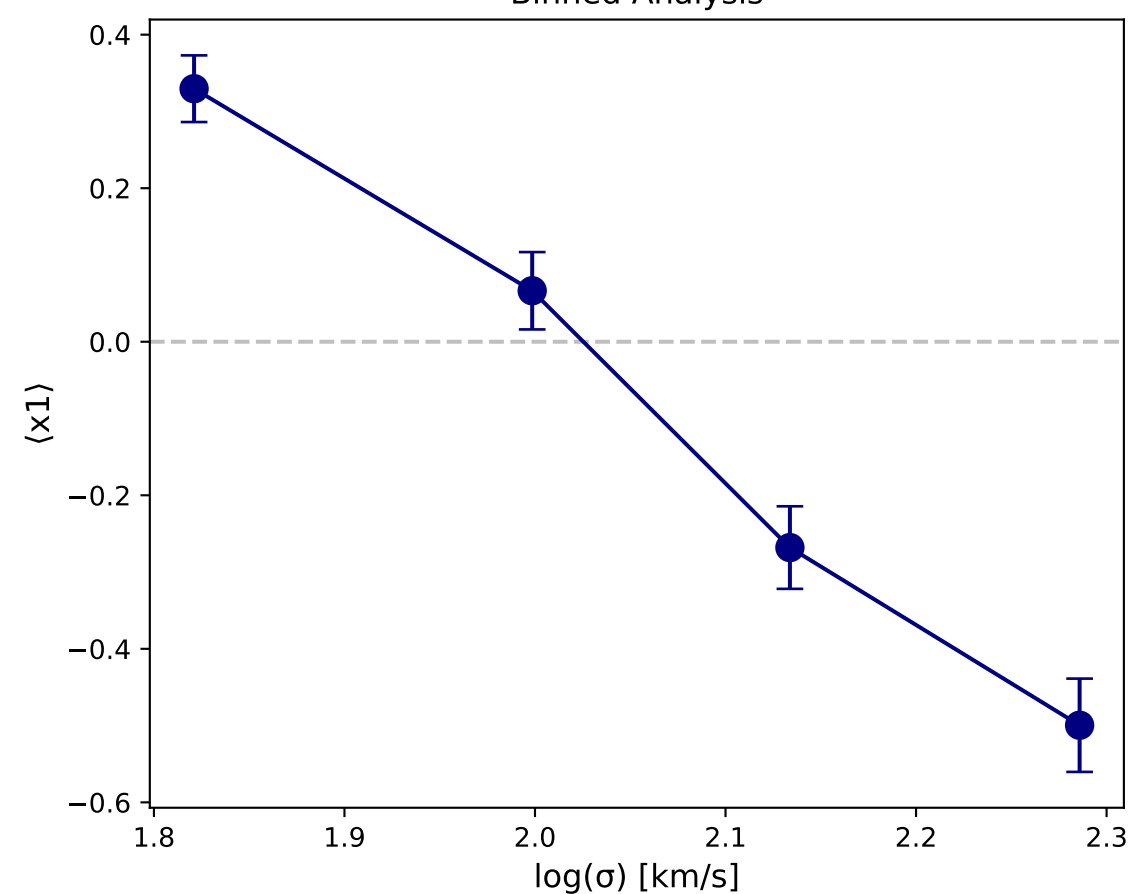
Binned Analysis
