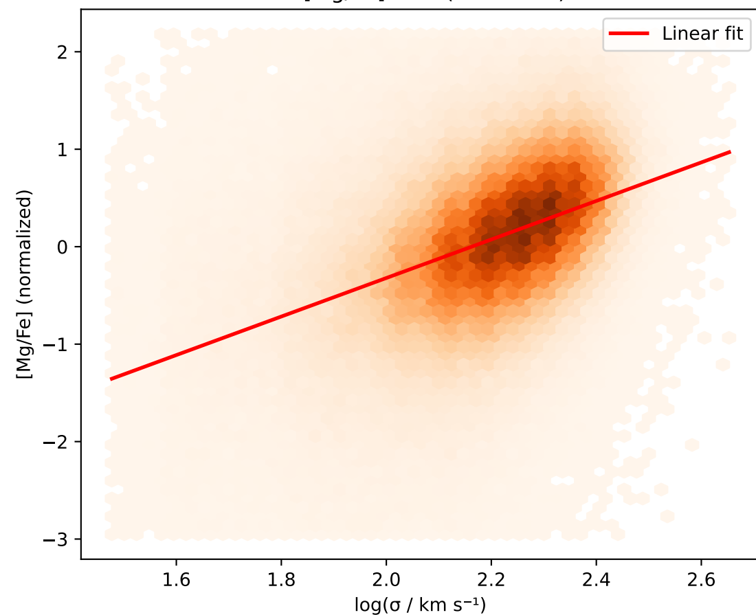
D. TEP Signature: \Delta r = -0.373 ( p = 0.0\text{e}+00 )
