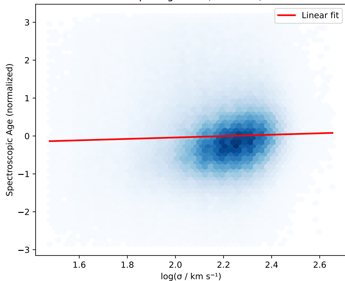
C. Age Indicators by \sigma Class
