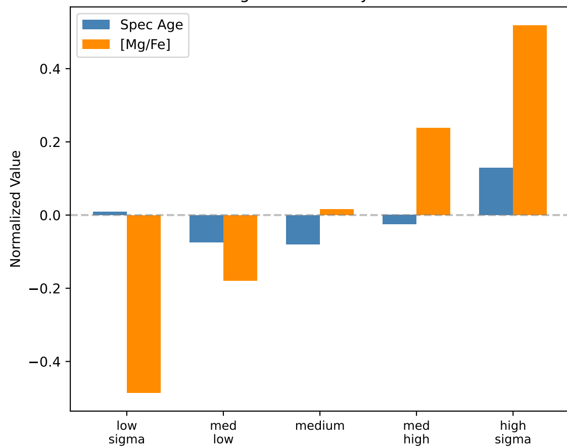
C. Age Indicators by \sigma Class
