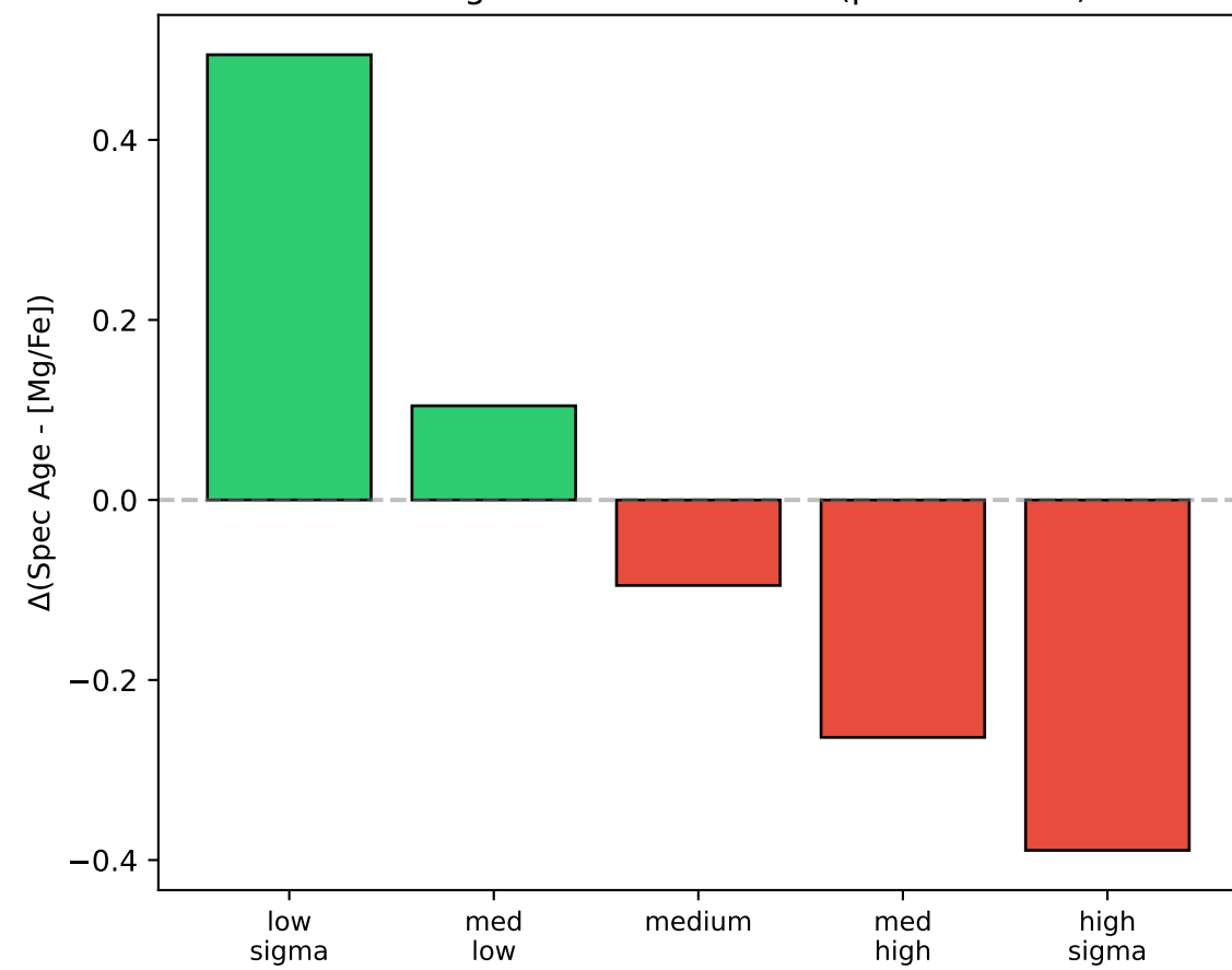
D. TEP Signature: \Delta r = -0.373 ( p = 0.0\text{e}+00 )
