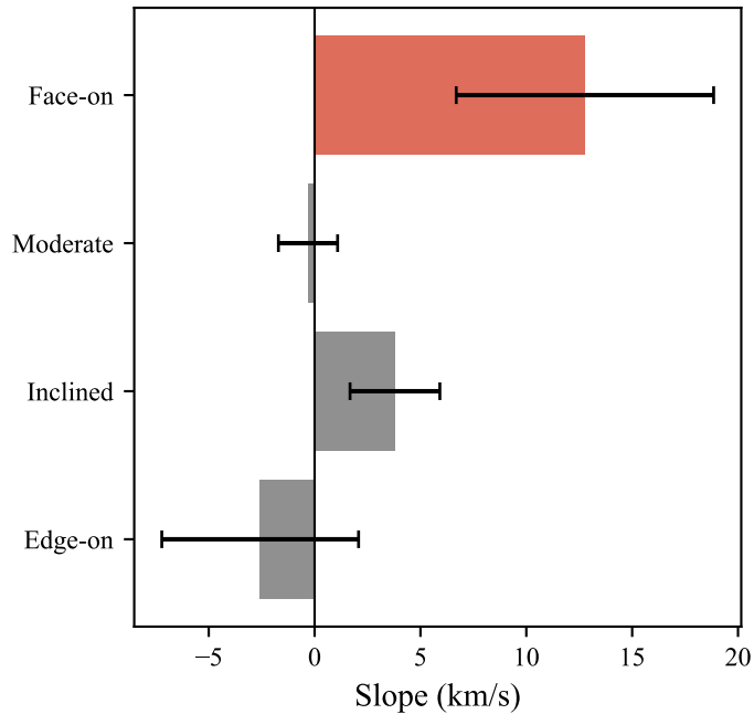
Inclination Stratification (Axial Ratio b/a)
