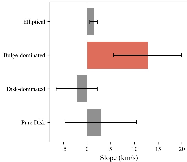
Morphology Stratification (Sérsic Index)
