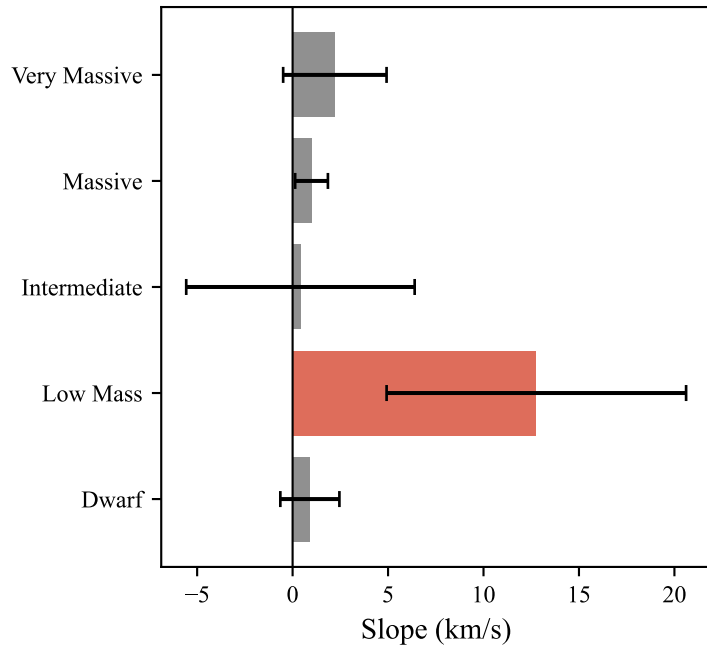
Mass Stratification (Velocity Dispersion)
