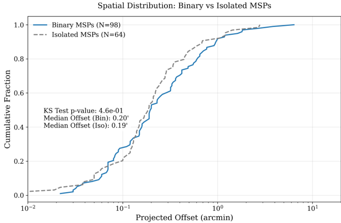
Figure 3.2: Spatial Distribution of Binary vs Isolated MSPs. Cumulative distribution functions (CDF) of projected offsets for Binary (blue) and Isolated (gray) MSPs. The distributions are statistically indistinguishable (KS test p = 0.46 ), with nearly identical median offsets (0.20' vs 0.19'). This rules out radial bias as the driver of the -0.32 dex spin-down difference; both populations sample the same dynamical environment.
