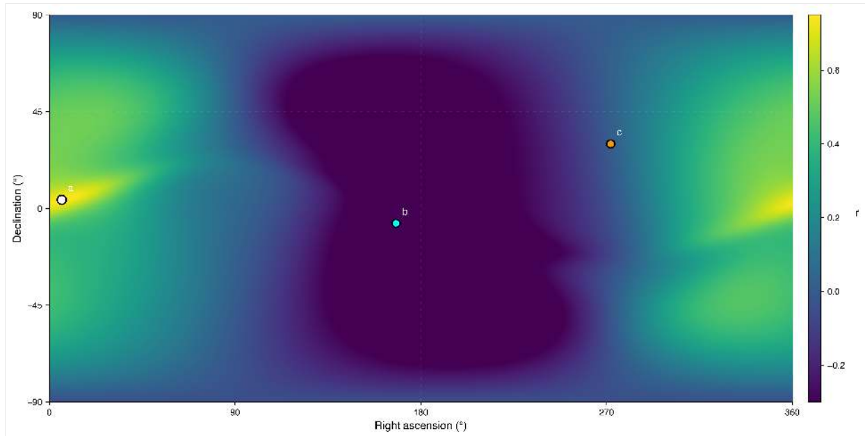
Figure 7: Reference direction identification via comprehensive sky search. Correlation strength ( r ) between predicted and observed anisotropy modulation across 65,341 candidate background velocity directions ( 1^\circ resolution grid, representing ultra-high resolution verification; primary analysis performed at 5^\circ resolution with 2,701 directions), under the corrected prograde orbital-velocity convention. Markers: (a) Best-fit direction (RA=6°, Dec=+4°, r=0.746 ), (b) CMB dipole control (RA=168°, Dec=-7°, 162^\circ separation — anti-phase), (c) Solar apex control (RA=272°, Dec=+30°, 92^\circ separation), and (d) Earth's aphelion-velocity tangent (RA \approx 12°, Dec \approx +5°, 6^\circ separation). The correlation peak lies in the ecliptic plane near Earth's orbital velocity tangent at aphelion and is nearly antipodal to the CMB dipole, excluding both fixed-frame hypotheses. Multi-resolution verification across four independent resolutions ( 10^\circ , 5^\circ , 2.5^\circ , 1^\circ ) spanning a 93-fold range in grid density shows monotonic convergence with asymptotic behavior (Supplementary Table S1), indicating the signal is robust across resolution scales. Color scale shows Pearson correlation coefficient. Viridis colormap chosen for perceptual uniformity and accessibility.
