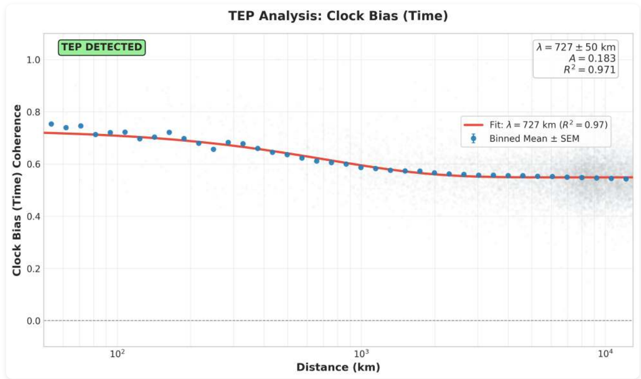
Figure 3.2: Phase coherence of clock bias between station pairs as a function of inter-station distance. Baseline GPS (L1) fit yields \lambda_T = 727 \pm 50 km with R^2 = 0.971 . Error bars represent standard error of the mean within each distance bin.
