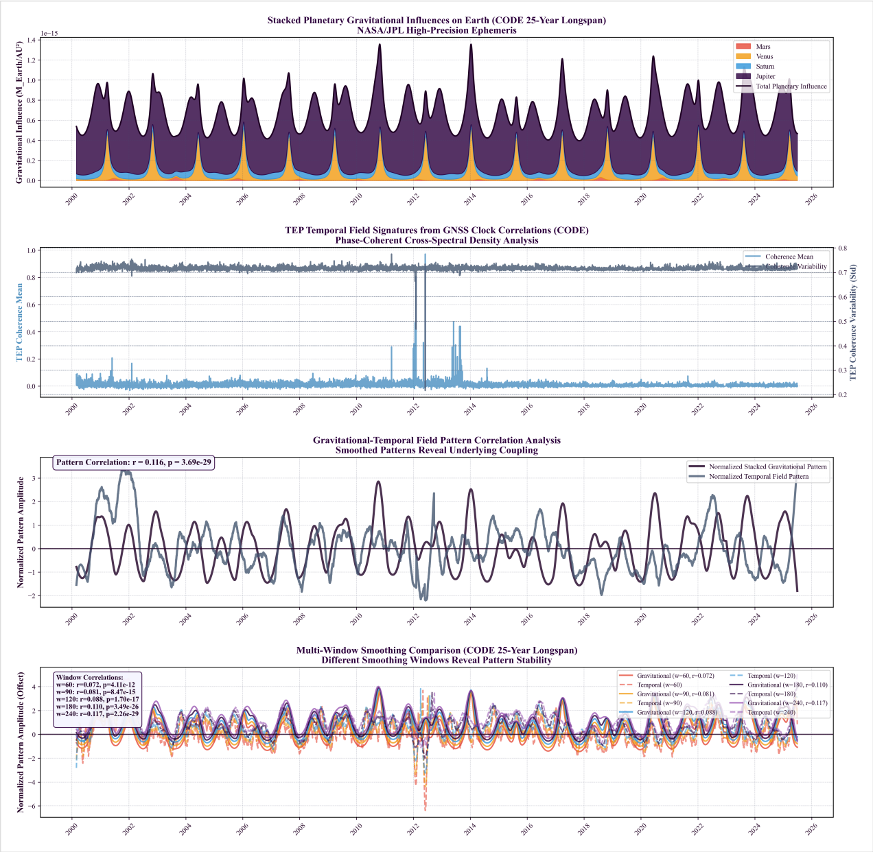
Figure 3.5.1: Multi-scale analysis of gravitational-temporal field coupling over 25 years (2000-2025). (A) Stacked planetary gravitational influences ( M/r^2 ) from JPL ephemeris showing relative contributions of Mars, Venus, Saturn, and Jupiter to total perturbation. (B) Daily network coherence variability (standard deviation across station pairs, light blue points) with Savitzky-Golay smoothing (dark line) reveals sustained temporal patterns. (C) Pattern correlation analysis between smoothed gravitational influence and coherence variability ( r = 0.116 , p = 3.69 \times 10^{-29} ) demonstrates systematic coupling. (D) Multi-window smoothing comparison (30-240 days) validates pattern stability with inter-window correlations r > 0.88 .
