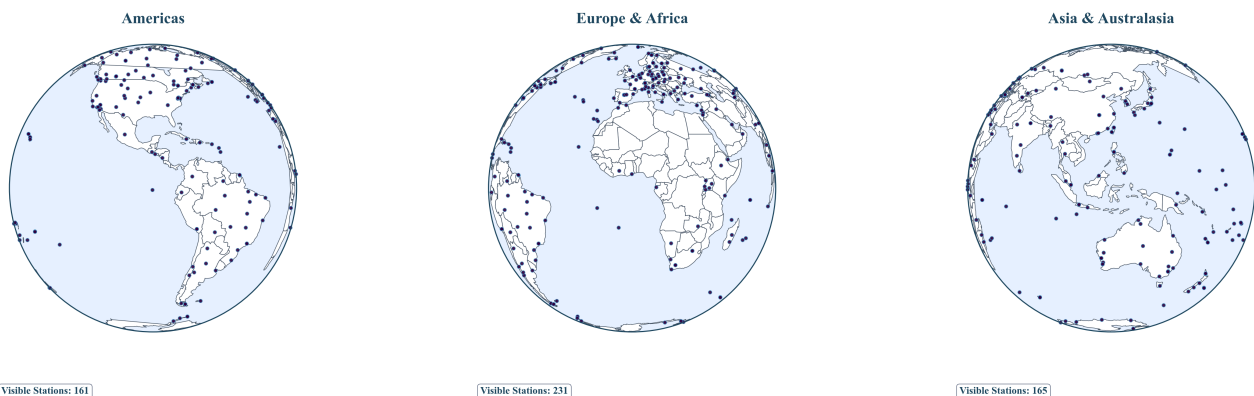
Figure 1a. Global GNSS Station Network: Three-globe perspective showing global GNSS infrastructure with ~360 stations used in this analysis. High station overlap between the source analysis centers enables robust cross-validation.
