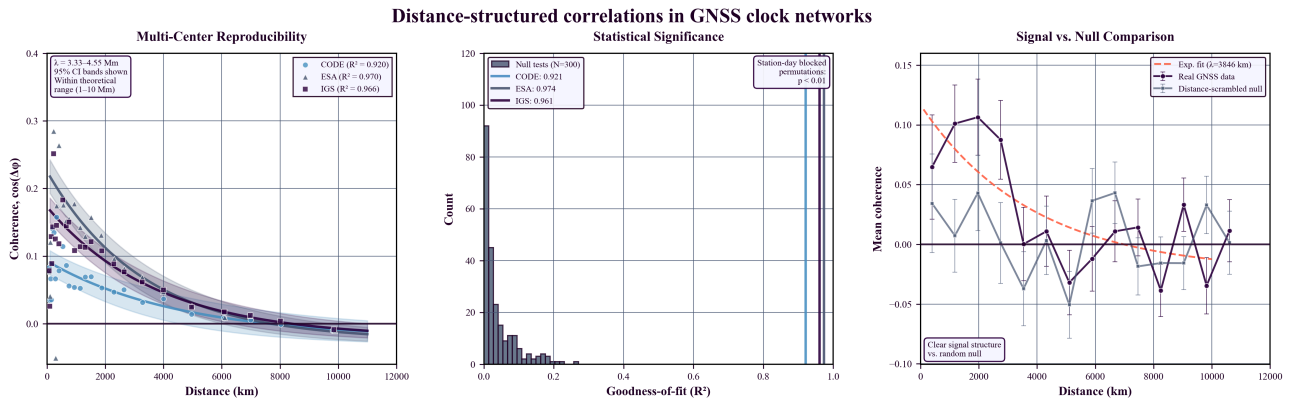
Figure 4. Continental-scale correlations in GNSS atomic clock networks. (a) Multi-center reproducibility: Exponential decay with 95% confidence intervals. The primary correlation length ( \lambda ) of 3,330–4,549 km is consistent across centers. (b) Statistical significance: Permutation tests demonstrate real R^2 values as extreme outliers. (c) Signal structure: Distance-scrambled comparison confirms spatial organization of correlations.
