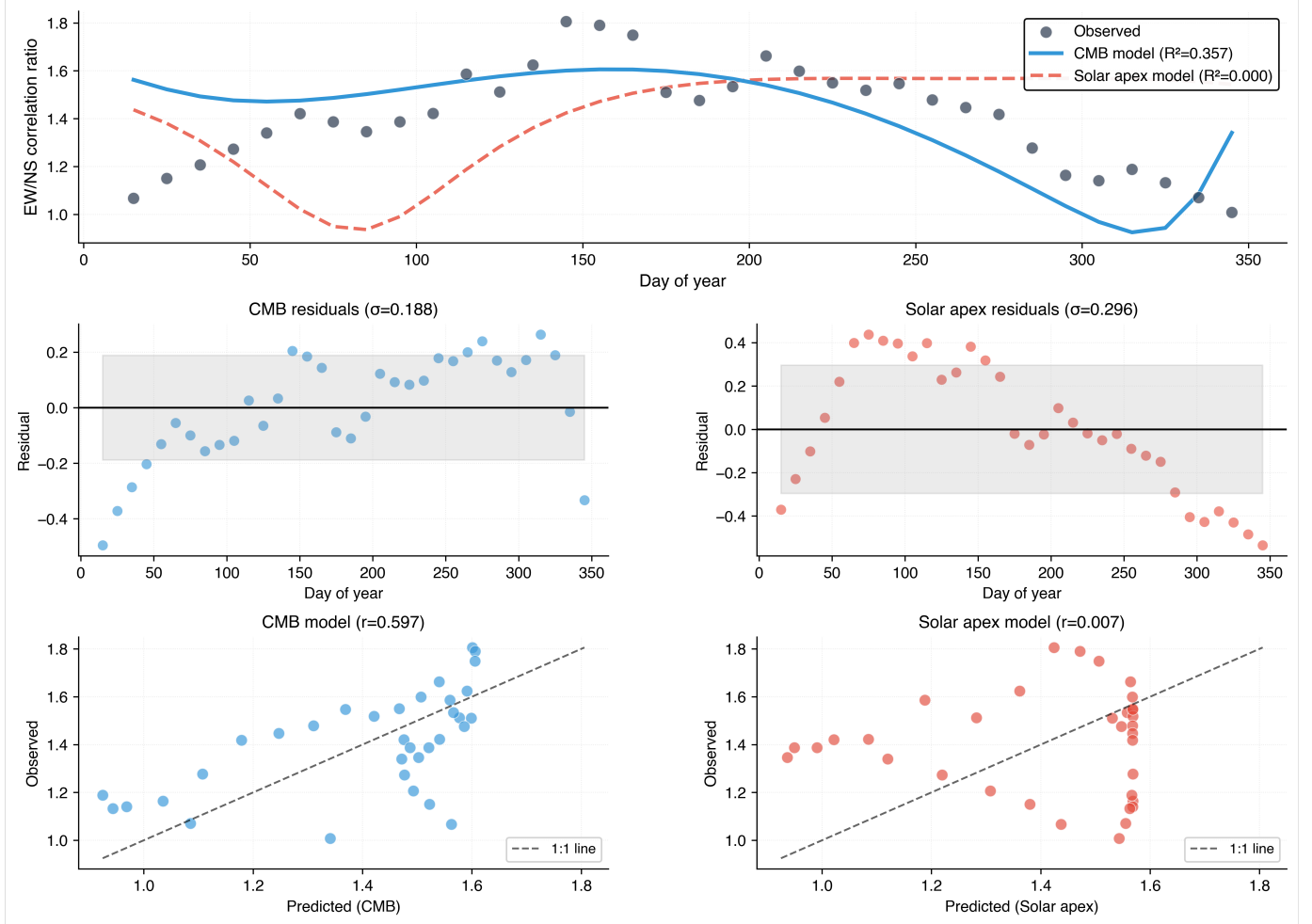
Figure 8: Detailed model comparison showing annual modulation prediction accuracy. Top panel: Observed EW/NS correlation ratios (gray points) across 34 temporal windows spanning 25.3 years, overlaid with predictions from CMB dipole model (blue, R^2=0.357 ) and Solar Apex model (red dashed, R^2\approx 0 ). Middle panels: Residual distributions for both models, with shaded \pm 1\sigma regions. CMB residuals ( \sigma=0.188 ) show no systematic bias; Solar Apex residuals ( \sigma=0.296 ) are 57% larger. Bottom panels: Predicted vs observed scatter plots demonstrating strong correlation for CMB model ( r=0.597 ) and near-zero correlation for Solar Apex model ( r=0.007 ). The 1:1 line (dashed) indicates perfect prediction. This comprehensive diagnostic confirms the CMB frame as the operative reference frame for temporal modulation.
