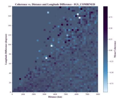
Figure 5c. IGS Combined: Cross-solution consistency validates robustness across software packages.
