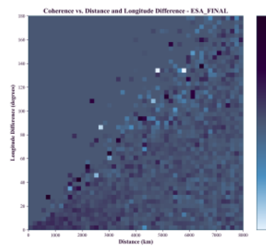
Figure 5b. ESA Final: Consistent patterns across distinct processing chains.
