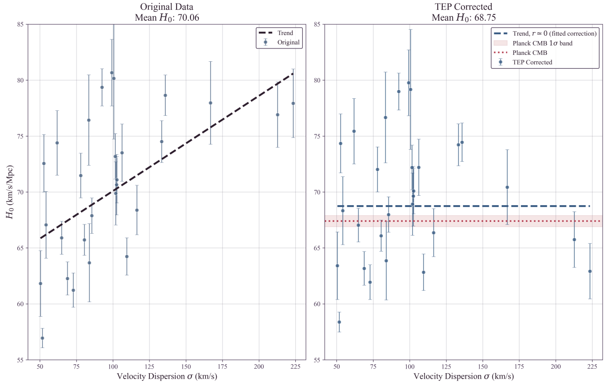
Figure 3: Effect of TEP correction on the distance ladder. Left: Original SH0ES data (29-host Hubble-flow-safe sample) showing the dependence of H_0 on host velocity dispersion ( \sigma , proxy for potential depth). The dashed line is a simple linear empirical fit to highlight the raw correlation; the formal quadratic physical model ( H_0 \propto \sigma^2 ) is applied to generate the corrected data in the right panel. The orange-highlighted outlier NGC 4639 ( H_0 \approx 47.3 km/s/Mpc) is explicitly annotated; jackknife analysis shows its removal strengthens the correlation, confirming it is a defensive robustness check rather than a liability. Right: TEP-corrected data ( \kappa_{\text{Cep}} \approx 1.05 \times 10^6 mag, \sigma^2/c^2 scaling). The corrected panel shows r \approx 0 by construction since \kappa_{\text{Cep}} is fitted to remove the trend; this is a fitted-correction diagnostic, not an independent validation statistic. Independent robustness is assessed by jackknife, host-contrast likelihood, train/test, anchor, and systematics tests. The unified mean (68.75 km/s/Mpc; bootstrap mean 68.80 \pm 1.46 ) is statistically consistent with Planck (dashed line, 0.91\sigma tension). Error bars represent standard measurement uncertainties.
