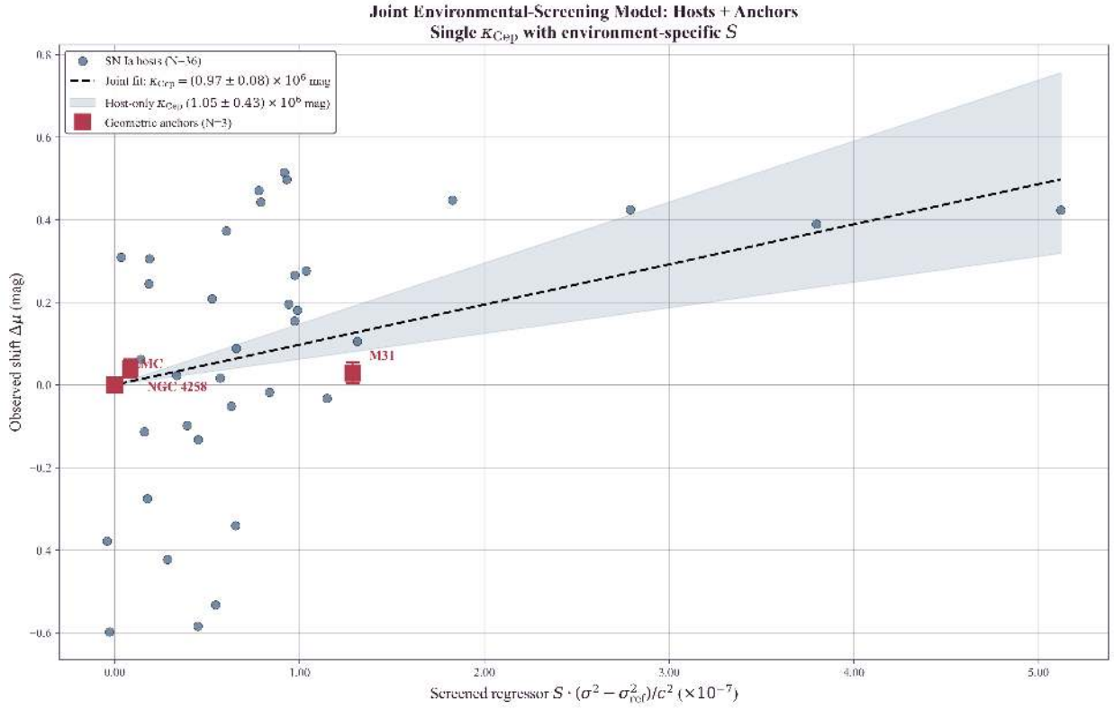
Figure 5: Joint environmental-screening model fit to 36 SN Ia hosts (blue circles) and 3 geometric anchors (red squares). All objects share a single Observable Response Coefficient \kappa_{\text{Cep}} = (0.97 \pm 0.08) \times 10^6 \text{ mag} , with environment-specific screening factors S_k attenuating the regressor for group-embedded anchors. The shaded band shows the host-only 1\sigma interval ((1.62 \pm 0.89) \times 10^6 \text{ mag}) .
