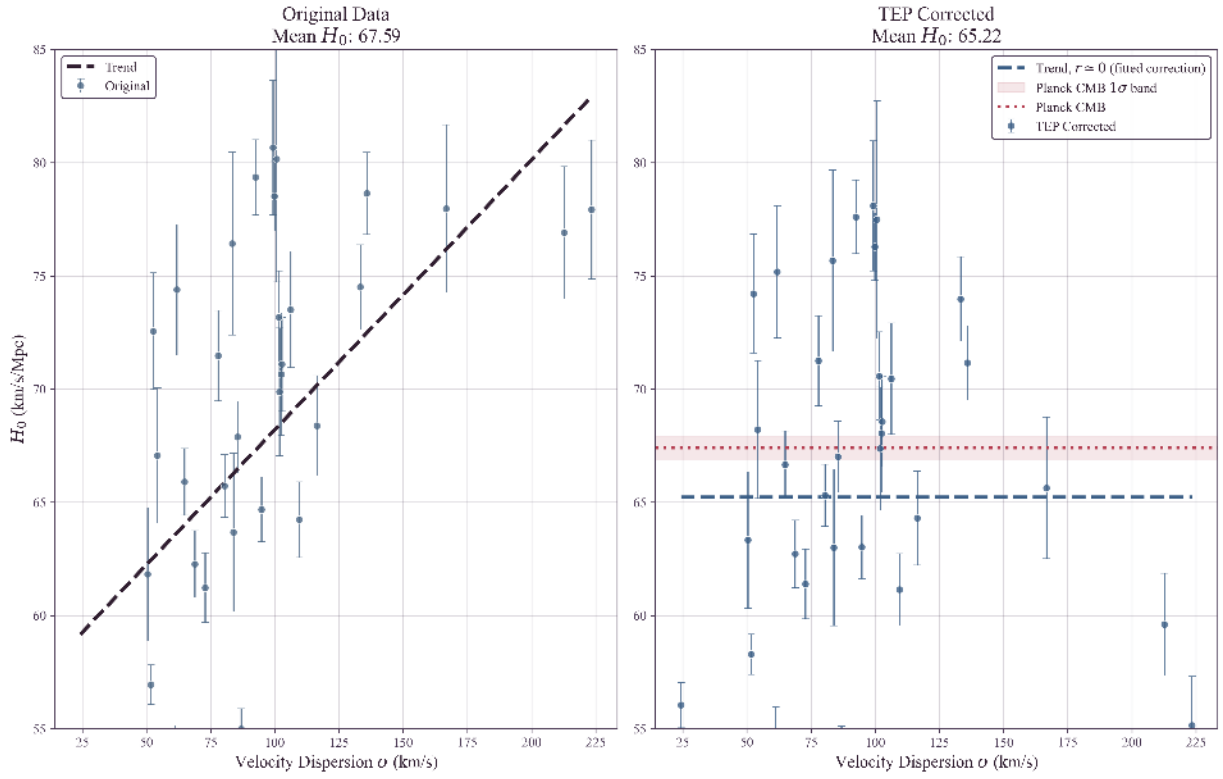
Figure 3: Effect of TEP correction on the distance ladder. Left: Original SH0ES data (36-host sample) showing the dependence of H_0 on host velocity dispersion ( \sigma , proxy for potential depth). The dashed line is a simple linear empirical fit to highlight the raw correlation; the formal quadratic physical model ( H_0 \propto \sigma^2 ) is applied to generate the corrected data in the right panel. The orange-highlighted outlier NGC 4639 ( H_0 \approx 47.3 km/s/Mpc) is explicitly annotated; jackknife analysis shows its removal strengthens the correlation, confirming it is a defensive robustness check rather than a liability. Right: TEP-corrected data ( \kappa_{\text{Cep}} \approx 1.62 \times 10^6 mag, \sigma^2/c^2 scaling). The corrected panel shows r \simeq 0 by construction since \kappa_{\text{Cep}} is fitted to remove the trend; this is a fitted-correction diagnostic, not an independent validation statistic. Independent robustness is assessed by jackknife, host-contrast likelihood, train/test, anchor, and systematics tests. The unified mean (65.22 km/s/Mpc; bootstrap mean 65.09 \pm 1.70 ) is statistically consistent with Planck (dashed line, 1.23\sigma tension). Error bars represent standard measurement uncertainties.
