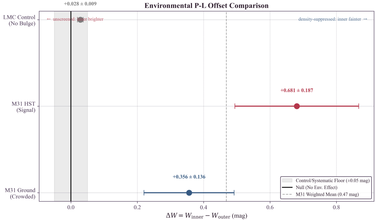
Figure 8: Synthesis of environmental differential tests. Both ground-based and HST M31 data show ‘Inner Fainter’ offsets consistent with TEP shear suppression (inner bulge more suppressed → less period contraction). The LMC control shows no large offset ( \sim 0.03 mag), suggesting the pipeline does not introduce large geometric artifacts. The solid vertical line marks the null hypothesis ( \Delta W = 0 ); the dashed vertical line marks the inverse-variance weighted mean of the M31 offsets. Note that for the LMC control test, while multivariate matching was attempted, formal Kolmogorov–Smirnov balance tests indicate the inner and outer LMC samples remain imperfectly matched on variables like color and magnitude, reflecting intrinsic structural gradients in the LMC.
