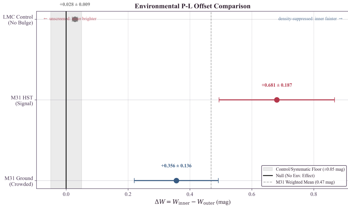
Figure 8: Synthesis of environmental differential tests. Both ground-based and HST M31 data show 'Inner Fainter' offsets consistent with TEP shear suppression (inner bulge more suppressed \rightarrow less period contraction). The LMC control shows no large offset ( \sim 0.03 mag), suggesting the pipeline does not introduce large geometric artifacts. The solid vertical line marks the null hypothesis ( \Delta W = 0 ); the dashed vertical line marks the inverse-variance weighted mean of the M31 offsets. Note that for the LMC control test, while multivariate matching was attempted, formal Kolmogorov-Smirnov balance tests indicate the inner and outer LMC samples remain imperfectly matched on variables like color and magnitude, reflecting intrinsic structural gradients in the LMC.
