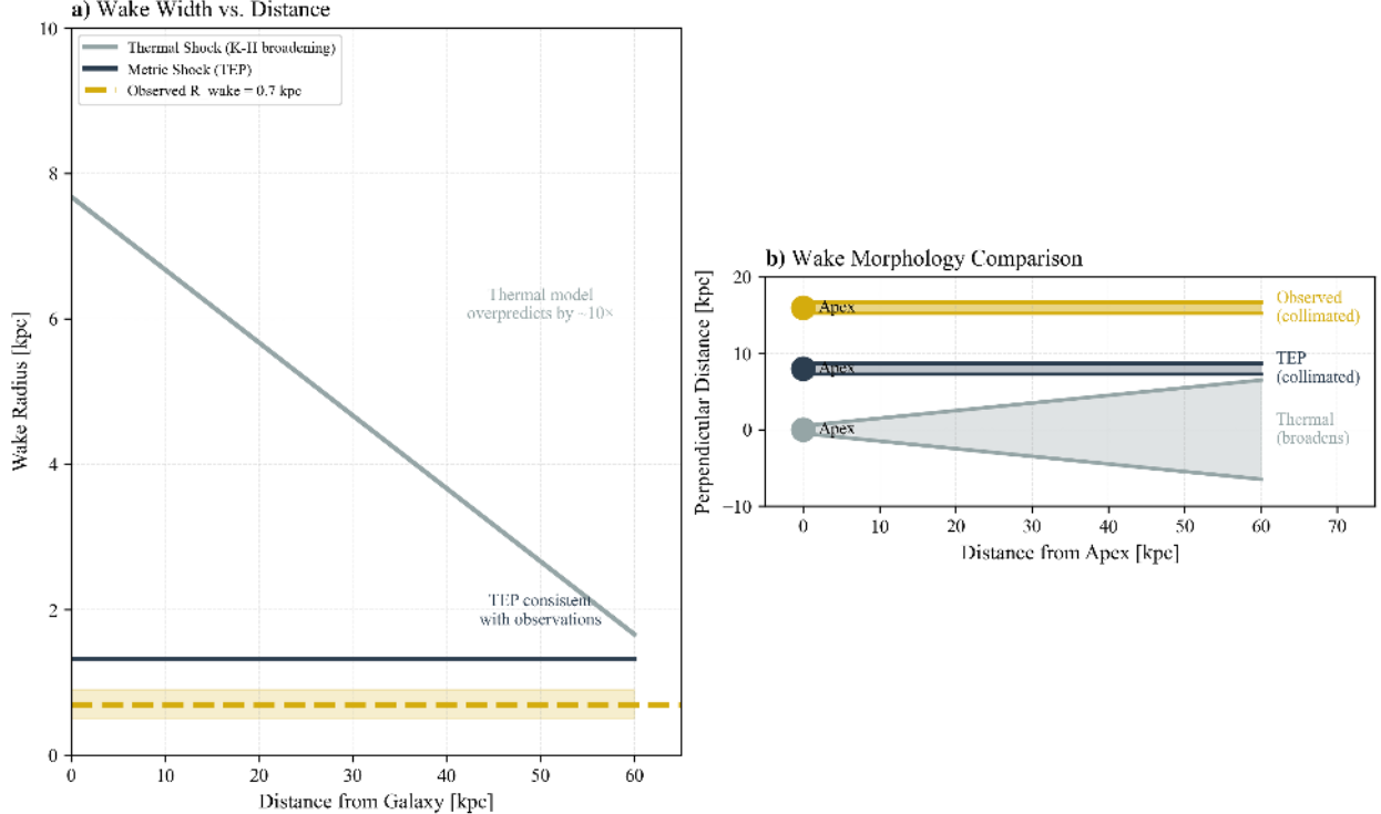
Figure 6: Wake Geometry Analysis. (A) Wake width vs. distance from galaxy. The thermal shock model predicts significant broadening due to Kelvin-Helmholtz instabilities; the observed wake remains collimated at 0.7 kpc. (B) Schematic comparison of wake morphologies. The 50:1 aspect ratio is inconsistent with thermal turbulence.
