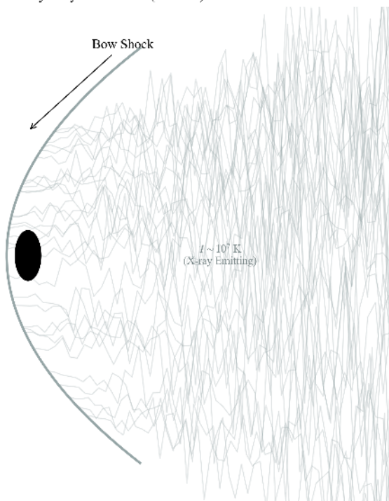
a) Standard Hydrodynamic Model (Thermal)
