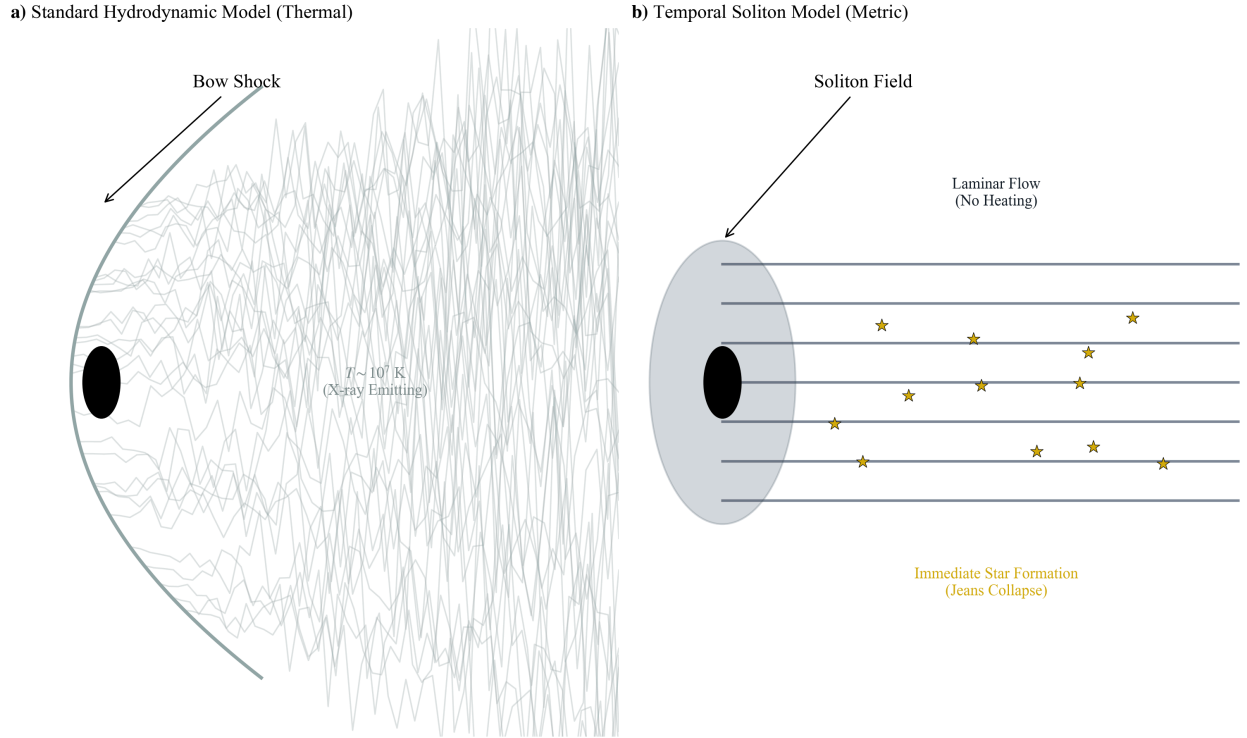
Figure 3: The Anatomy of the Wake. Left (turbulent/hot): A standard hydrodynamic model, where a physical projectile generates turbulence and post-shock heating ( T \gtrsim 10^7 K). Kelvin-Helmholtz instabilities disrupt the wake boundary, and the Jeans length exceeds 100 kpc, suppressing sub-kpc fragmentation. Right (laminar/cold): A metric-shock model, where a propagating region of time dilation produces a coherent disturbance without bulk thermalization. Gas remains near T \sim 10^4 K, the wake boundary stays sharp (aspect ratio 50:1), and fragmentation into star-forming clumps is permitted. This left-right contrast provides a qualitative discriminant between models.
