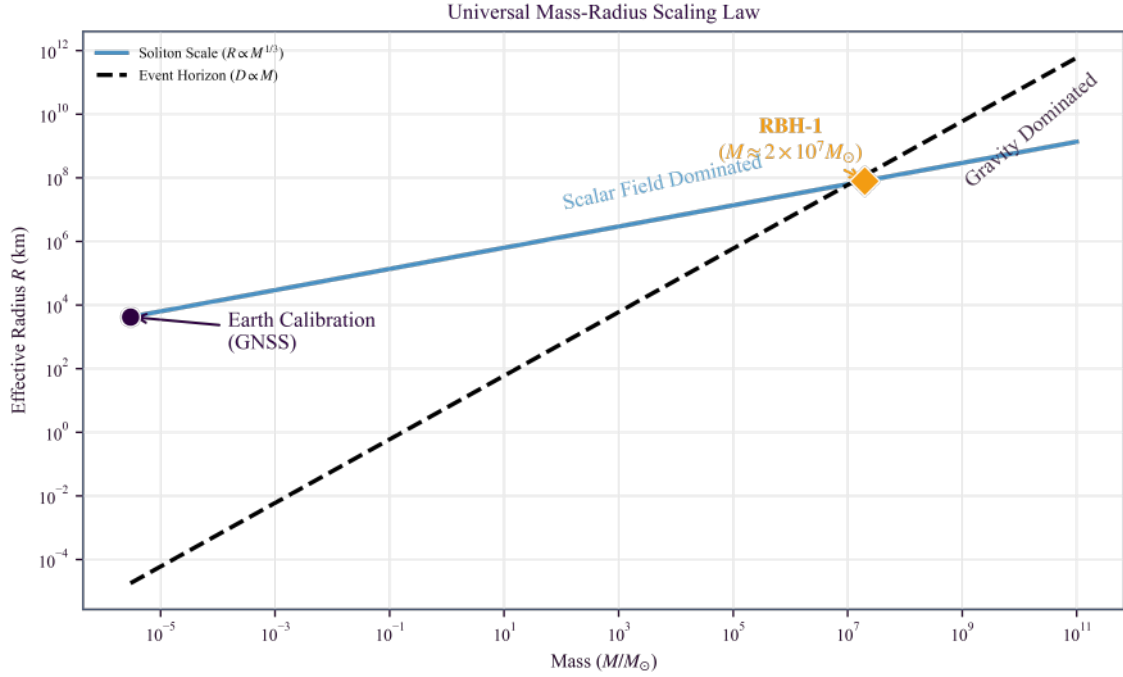
Figure C.1: The Universal Scaling Plot. The trajectory represents the saturation scaling law ( R \propto M^{1/3} ), calibrated via terrestrial GNSS data ( L_e \approx 4200 km). This single parameter is consistent with the onset of dark matter dynamics in spiral galaxies (SPARC) and the critical anti-glitch period in magnetars, organizing phenomena across 40 orders of magnitude in mass (pending dependency audit).
